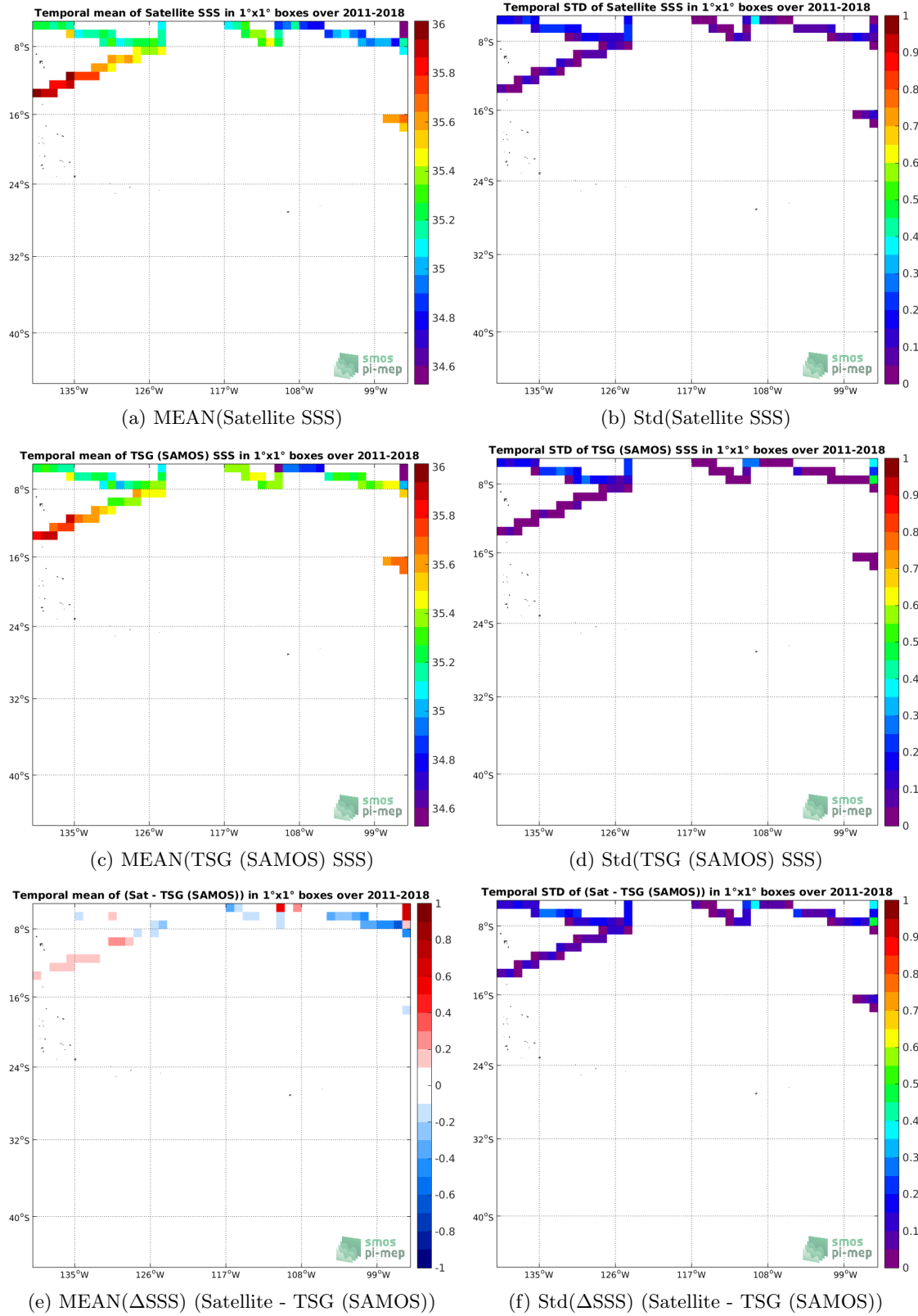
Figure 6: Temporal mean (left) and Std (right) of SSS from SMOS L3 v2 - 9-Days (BEC) (top), TSG (SAMOS) (middle), and of \Delta SSS (Satellite - TSG (SAMOS)). Only match-up pairs are used to generate these maps.
