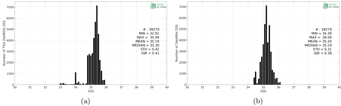
Figure 2: Histograms of SSS from TSG (SAMOS) (a) and SMOS L3 v2 - 9-Days (BEC) (b) considering all match-up pairs per bins of 0.1 over the OTT zone Pi-MEP region and for the full satellite product period.
