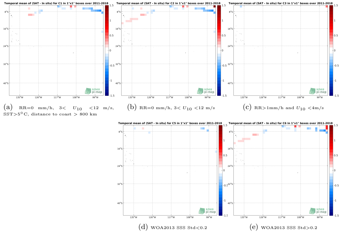
Figure 12: Temporal mean gridded over spatial boxes of size 1^\circ \times 1^\circ of \Delta SSS (SMOS L3 v2 - 9-Days (BEC) - TSG (SAMOS)) for 5 different subdatasets corresponding to: RR=0 mm/h, 3 < U_{10} < 12 m/s, SST > 5^\circ C , distance to coast > 800 km (a), RR=0 mm/h, 3 < U_{10} < 12 m/s (b), RR > 1 mm/h and U_{10} < 4 m/s (c), WOA2013 SSS Std < 0.2 (d), WOA2013 SSS Std > 0.2 (e).
