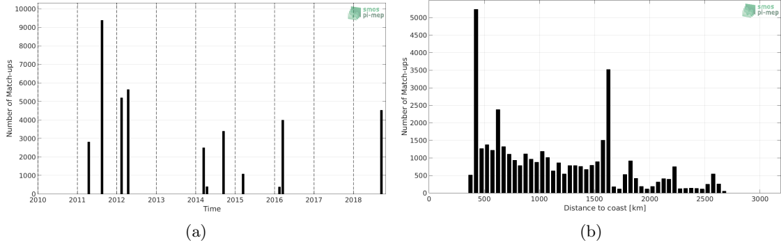
Figure 1: Number of match-ups between TSG (SAMOS) and SMOS L3 v2 - 9-Days (BEC) SSS as a function of time (a) and as function of the distance to coast (b) over the OTT zone Pi-MEP region and for the full satellite product period.
