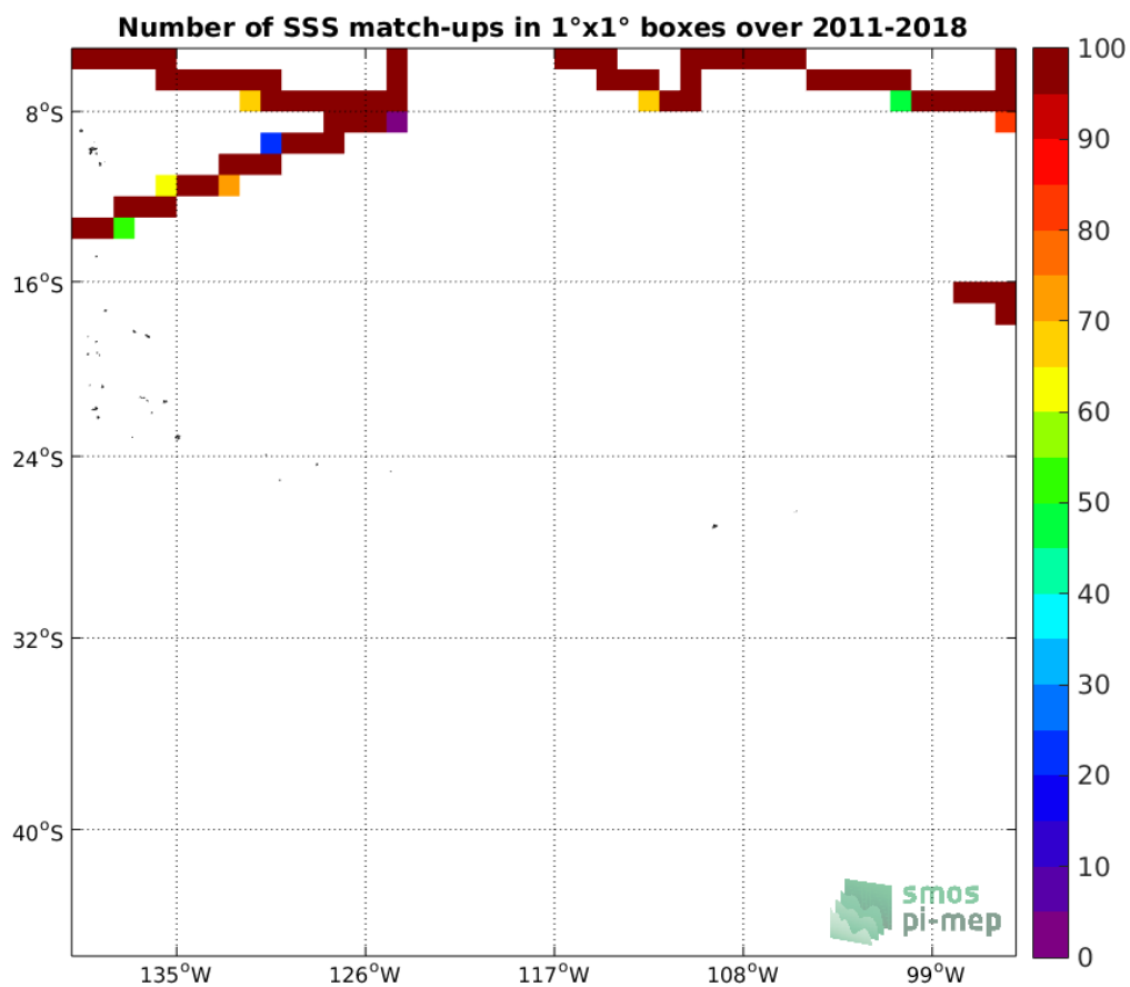
Figure 4: Number of SSS match-ups between TSG (SAMOS) SSS and the SMOS L3 v2 - 9-Days (BEC) SSS product for the OTT zone Pi-MEP region over 1°x1° boxes and for the full satellite product period.
