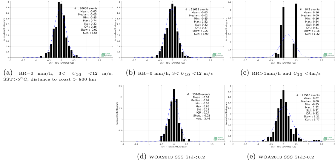
Figure 13: Normalized histogram of \Delta SSS (SMOS L3 v2 - 9-Days (BEC) - TSG (SAMOS)) for 5 different subdatasets corresponding to: RR=0 mm/h, 3 < U_{10} < 12 m/s, SST>5°C, distance to coast > 800 km (a), RR=0 mm/h, 3 < U_{10} < 12 m/s (b), RR>1mm/h and U_{10} < 4 m/s (c), WOA2013 SSS Std<0.2 (d), WOA2013 SSS Std>0.2 (e).
