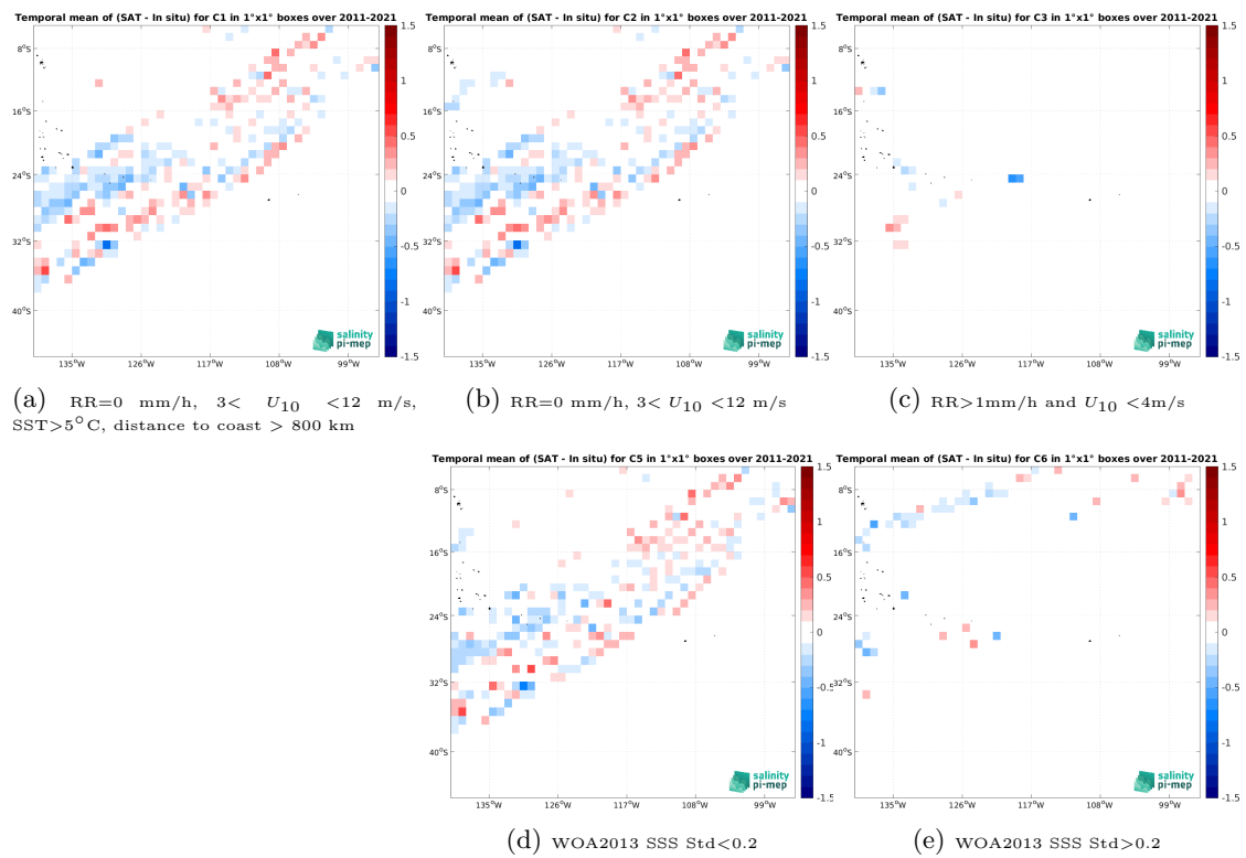
Figure 14: Temporal mean gridded over spatial boxes of size 1^\circ \times 1^\circ of \Delta\text{SSS} (SMOS SSS L3 v2 - 9-Days (BEC) - TSG (LEGOS-DM)) for 5 different subdatasets corresponding to:RR=0 mm/h, 3 < U_{10} < 12 m/s, SST >5^\circ\text{C} , distance to coast > 800 km (a), RR=0 mm/h, 3 < U_{10} < 12 m/s (b), RR >1 mm/h and U_{10} < 4 m/s (c), WOA2013 SSS Std <0.2 (d), WOA2013 SSS Std >0.2 (e).
