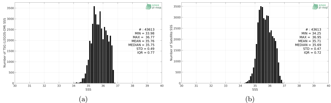
Figure 2: Histograms of SSS from TSG (LEGOS-DM) (a) and SMOS L3 v2 - 9-Days (BEC) (b) considering all match-up pairs per bins of 0.1 over the OTT zone Pi-MEP region and for the full satellite product period.
