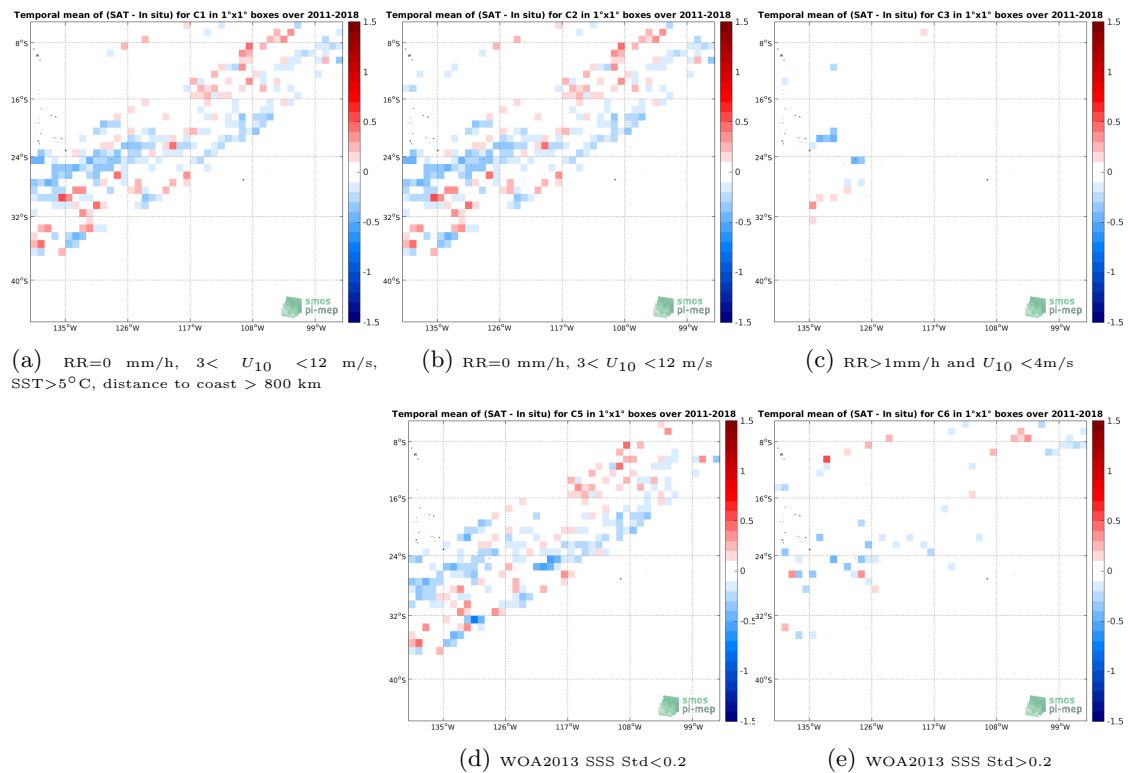
Figure 12: Temporal mean gridded over spatial boxes of size 1^\circ \times 1^\circ of \Delta SSS (SMOS L3 v2 - 9-Days (BEC) - TSG (LEGOS-DM)) for 5 different subdatasets corresponding to:RR=0 mm/h, 3 < U_{10} < 12 m/s, SST >5^\circ\text{C} , distance to coast > 800 km (a), RR=0 mm/h, 3 < U_{10} < 12 m/s (b), RR >1 mm/h and U_{10} < 4 m/s (c), WOA2013 SSS Std <0.2 (d), WOA2013 SSS Std >0.2 (e).
