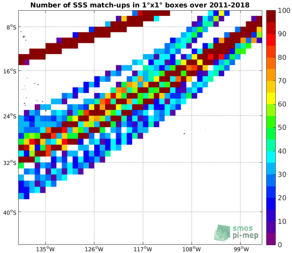
Figure 4: Number of SSS match-ups between TSG (LEGOS-DM) SSS and the SMOS L3 v2 - 9-Days (BEC) SSS product for the OTT zone Pi-MEP region over 1°x1° boxes and for the full satellite product period.
