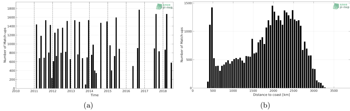
Figure 1: Number of match-ups between TSG (LEGOS-DM) and SMOS L3 v2 - 9-Days (BEC) SSS as a function of time (a) and as function of the distance to coast (b) over the OTT zone Pi-MEP region and for the full satellite product period.
