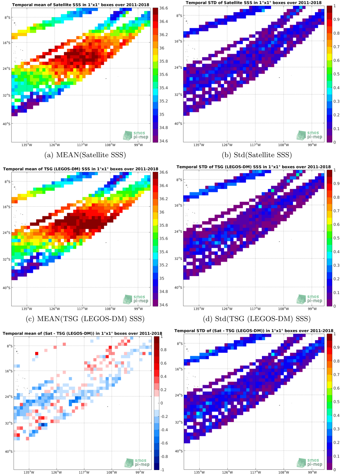
Figure 6: Temporal mean (left) and Std (right) of SSS from SMOS L3 v2 - 9-Days (BEC) (top), TSG (LEGOS-DM) (middle), and of \Delta SSS (Satellite - TSG (LEGOS-DM)). Only match-up pairs are used to generate these maps.
