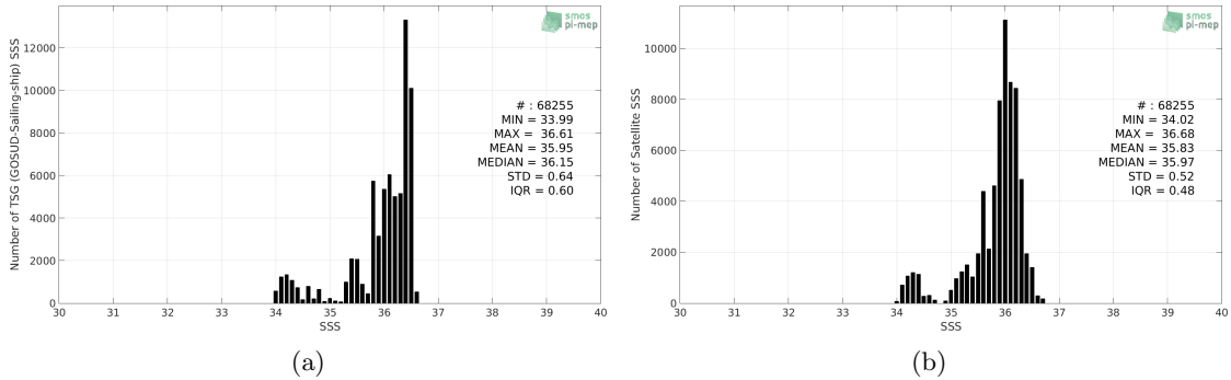
Figure 2: Histograms of SSS from TSG (GOSUD-Sailing-ship) (a) and SMOS L3 v2 - 9-Days (BEC) (b) considering all match-up pairs per bins of 0.1 over the OTT zone Pi-MEP region and for the full satellite product period.
