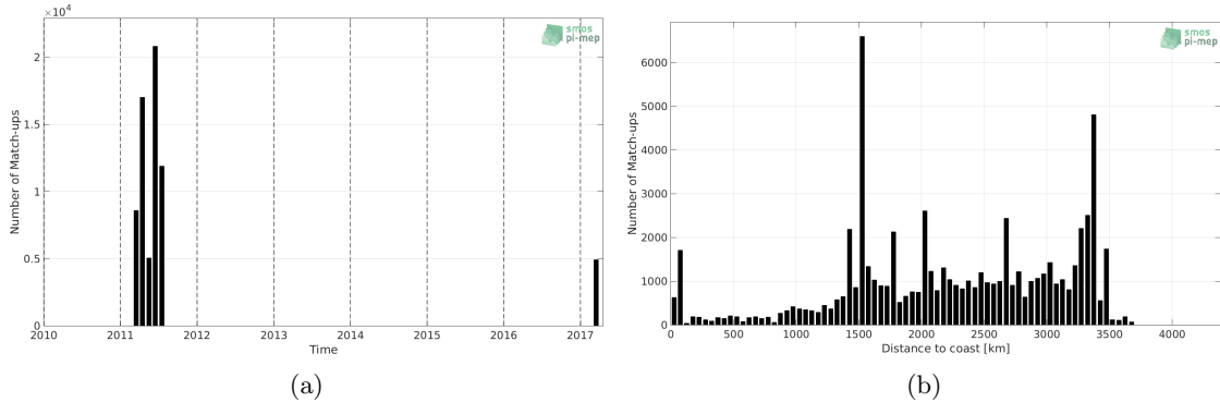
Figure 1: Number of match-ups between TSG (GOSUD-Sailing-ship) and SMOS L3 v2 - 9-Days (BEC) SSS as a function of time (a) and as function of the distance to coast (b) over the OTT zone Pi-MEP region and for the full satellite product period.
