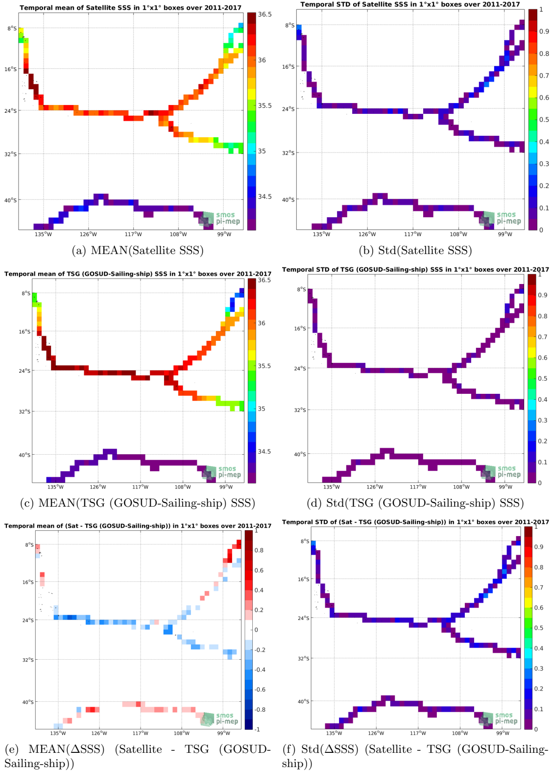
Figure 6: Temporal mean (left) and Std (right) of SSS from SMOS L3 v2 - 9-Days (BEC) (top), TSG (GOSUD-Sailing-ship) (middle), and of \Delta SSS (Satellite - TSG (GOSUD-Sailing-ship)). Only match-up pairs are used to generate these maps.
