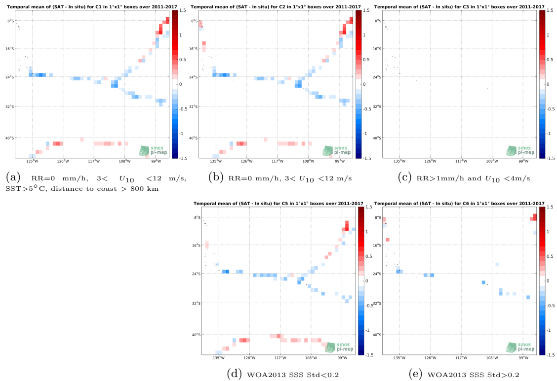
Figure 12: Temporal mean gridded over spatial boxes of size 1^\circ \times 1^\circ of \Delta SSS (SMOS L3 v2 - 9-Days (BEC) - TSG (GOSUD-Sailing-ship)) for 5 different subdatasets corresponding to: RR=0 mm/h, 3 < U_{10} < 12 m/s, SST > 5^\circ C , distance to coast > 800 km (a), RR=0 mm/h, 3 < U_{10} < 12 m/s (b), RR > 1 mm/h and U_{10} < 4 m/s (c), WOA2013 SSS Std<0.2 (d), WOA2013 SSS Std>0.2 (e).
