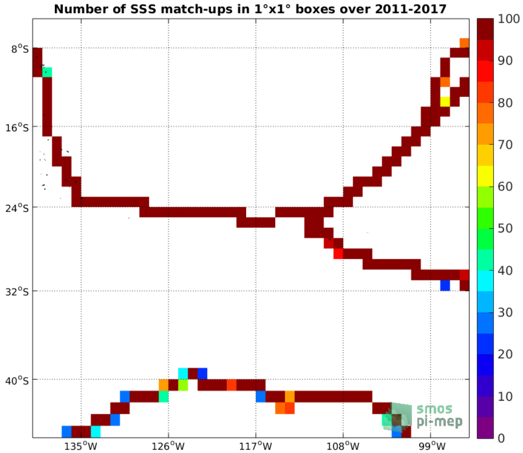
Figure 4: Number of SSS match-ups between TSG (GOSUD-Sailing-ship) SSS and the SMOS L3 v2 - 9-Days (BEC) SSS product for the OTT zone Pi-MEP region over 1°x1° boxes and for the full satellite product period.
