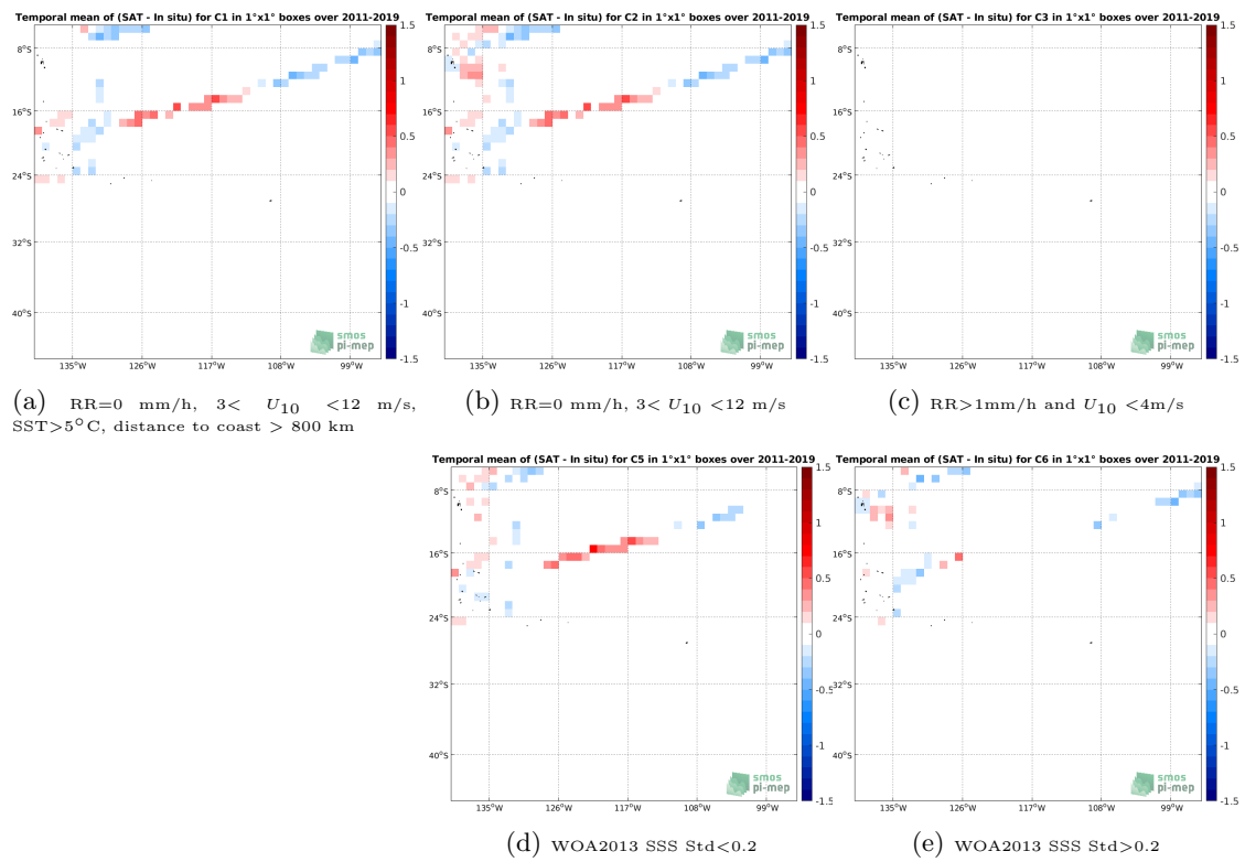
Figure 12: Temporal mean gridded over spatial boxes of size 1^\circ \times 1^\circ of \Delta\text{SSS} (SMOS SSS L3 v2 - 9-Days (BEC) - TSG (GOSUD-Research-vessel)) for 5 different subdatasets corresponding to:RR=0 mm/h, 3 < U_{10} < 12 m/s, SST>5°C, distance to coast > 800 km (a), RR=0 mm/h, 3 < U_{10} < 12 m/s (b), RR>1mm/h and U_{10} < 4 m/s (c), WOA2013 SSS Std<0.2 (d), WOA2013 SSS Std>0.2 (e).
