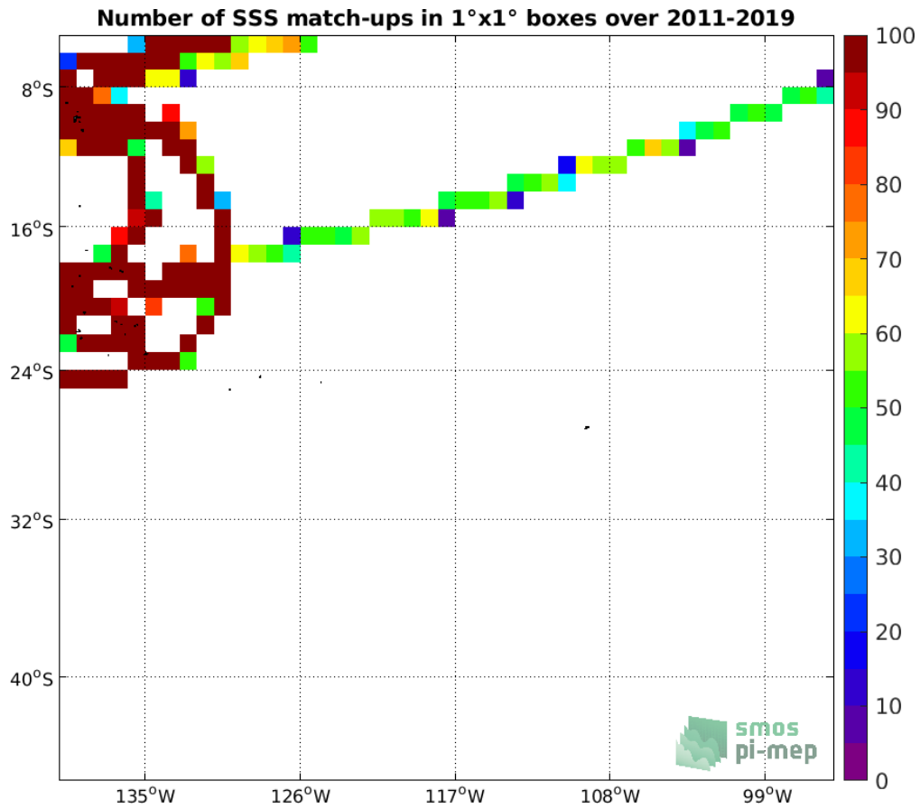
Figure 4: Number of SSS match-ups between TSG (GOSUD-Research-vessel) SSS and the SMOS SSS L3 v2 - 9-Days (BEC) SSS product for the OTT zone Pi-MEP region over 1^{\circ} \times 1^{\circ} boxes and for the full satellite product period.
