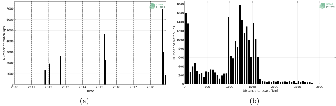
Figure 1: Number of match-ups between TSG (GOSUD-Research-vessel) and SMOS L3 v2 - 9-Days (BEC) SSS as a function of time (a) and as function of the distance to coast (b) over the OTT zone Pi-MEP region and for the full satellite product period.
