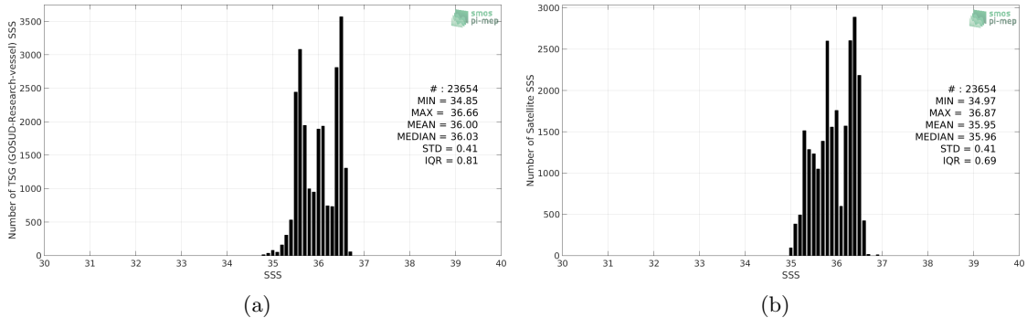
Figure 2: Histograms of SSS from TSG (GOSUD-Research-vessel) (a) and SMOS L3 v2 - 9-Days (BEC) (b) considering all match-up pairs per bins of 0.1 over the OTT zone Pi-MEP region and for the full satellite product period.
