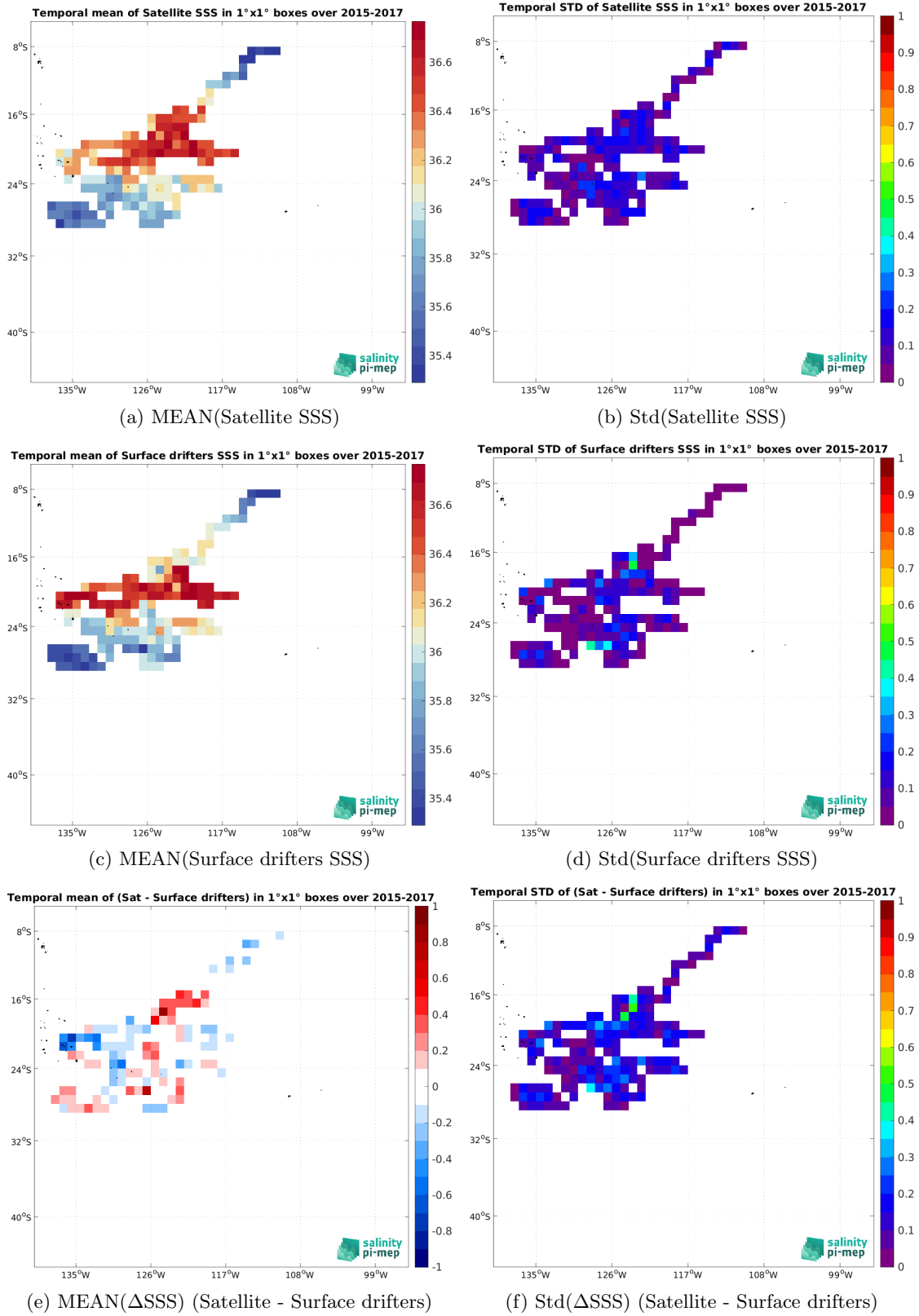
Figure 6: Temporal mean (left) and Std (right) of SSS from SMOS SSS L3 v2 - 9-Days (BEC) (top), Surface drifters (middle), and of \Delta SSS (Satellite - Surface drifters). Only match-up pairs are used to generate these maps.
