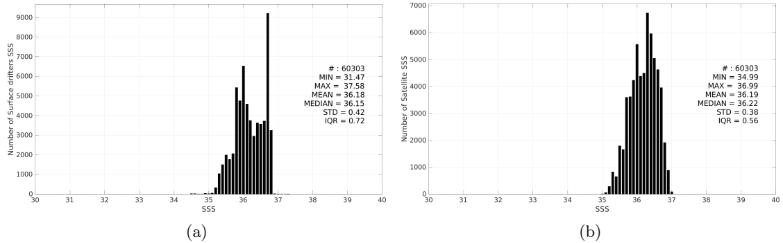
Figure 3: Histograms of SSS from Surface drifters (a) and SMOS SSS L3 v2 - 9-Days (BEC) (b) considering all match-up pairs per bins of 0.1 over the OTT zone Pi-MEP region and for the full satellite product period.
