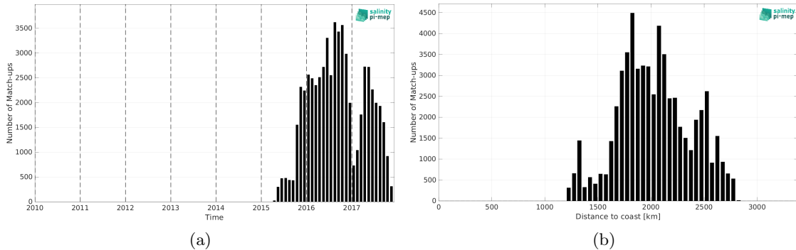
Figure 2: Number of match-ups between Surface drifters and SMOS SSS L3 v2 - 9-Days (BEC) SSS as a function of time (a) and as function of the distance to coast (b) over the OTT zone Pi-MEP region and for the full satellite product period.
