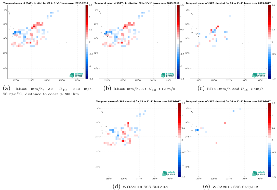
Figure 13: Temporal mean gridded over spatial boxes of size 1^\circ \times 1^\circ of \Delta SSS (SMOS SSS L3 v2 - 9-Days (BEC) - Surface drifters) for 5 different subdatasets corresponding to:RR=0 mm/h, 3 < U_{10} < 12 m/s, SST >5^\circ C, distance to coast > 800 km (a), RR=0 mm/h, 3 < U_{10} < 12 m/s (b), RR >1 mm/h and U_{10} < 4 m/s (c), WOA2013 SSS Std <0.2 (d), WOA2013 SSS Std >0.2 (e).
