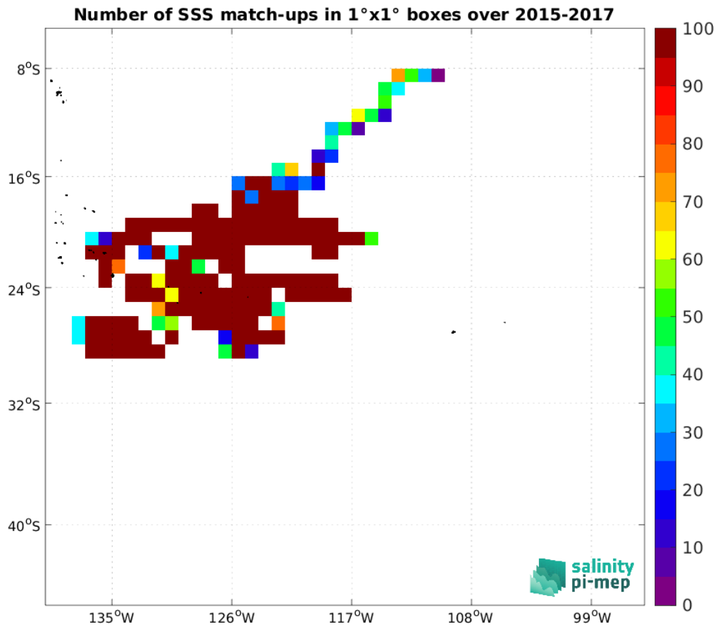
Figure 4: Number of SSS match-ups between Surface drifters SSS and the SMOS SSS L3 v2 - 9-Days (BEC) SSS product for the OTT zone Pi-MEP region over 1^\circ \times 1^\circ boxes and for the full satellite product period.
