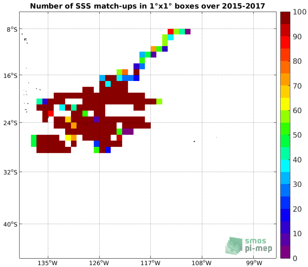
Figure 3: Number of SSS match-ups between Surface drifters SSS and the SMOS SSS L3 v2 - 9-Days (BEC) SSS product for the OTT zone Pi-MEP region over 1°x1° boxes and for the full satellite product period.
