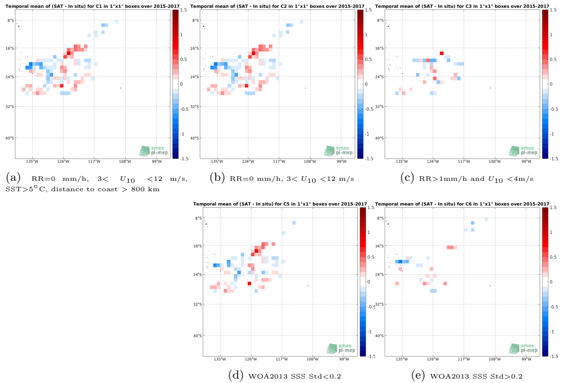
Figure 11: Temporal mean gridded over spatial boxes of size 1^\circ \times 1^\circ of \Delta\text{SSS} (SMOS SSS L3 v2 - 9-Days (BEC) - Surface drifters) for 5 different subdatasets corresponding to:RR=0 mm/h, 3 < U_{10} < 12 m/s, SST >5^\circ\text{C} , distance to coast > 800 km (a), RR=0 mm/h, 3 < U_{10} < 12 m/s (b), RR >1 mm/h and U_{10} < 4 m/s (c), WOA2013 SSS Std <0.2 (d), WOA2013 SSS Std >0.2 (e).
