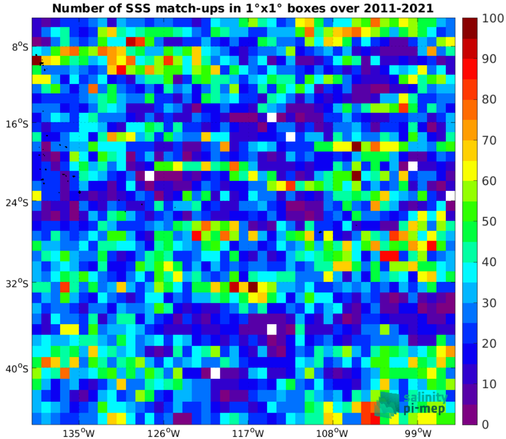
Figure 4: Number of SSS match-ups between Argo SSS and the SMOS SSS L3 v2 - 9-Days (BEC) SSS product for the OTT zone Pi-MEP region over 1^\circ \times 1^\circ boxes and for the full satellite product period.
