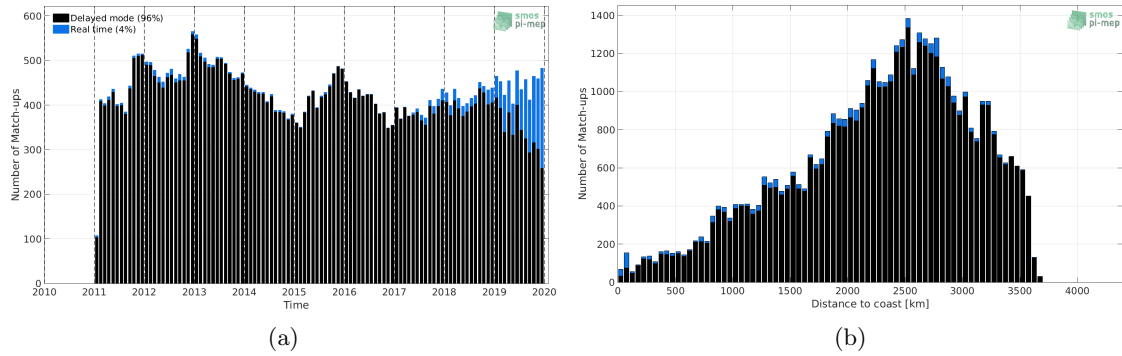
Figure 1: Number of match-ups between Argo and SMOS L3 v2 - 9-Days (BEC) SSS as a function of time (a) and as function of the distance to coast (b) over the OTT zone Pi-MEP region and for the full satellite product period.
