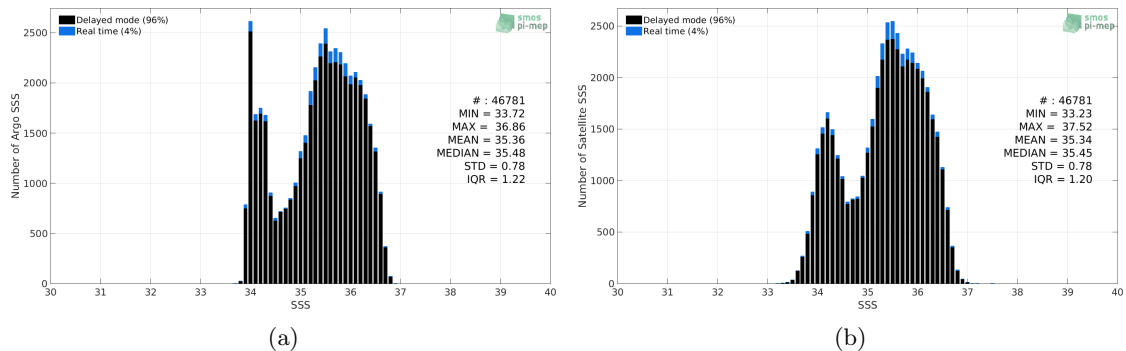
Figure 2: Histograms of SSS from Argo (a) and SMOS L3 v2 - 9-Days (BEC) (b) considering all match-up pairs per bins of 0.1 over the OTT zone Pi-MEP region and for the full satellite product period.
