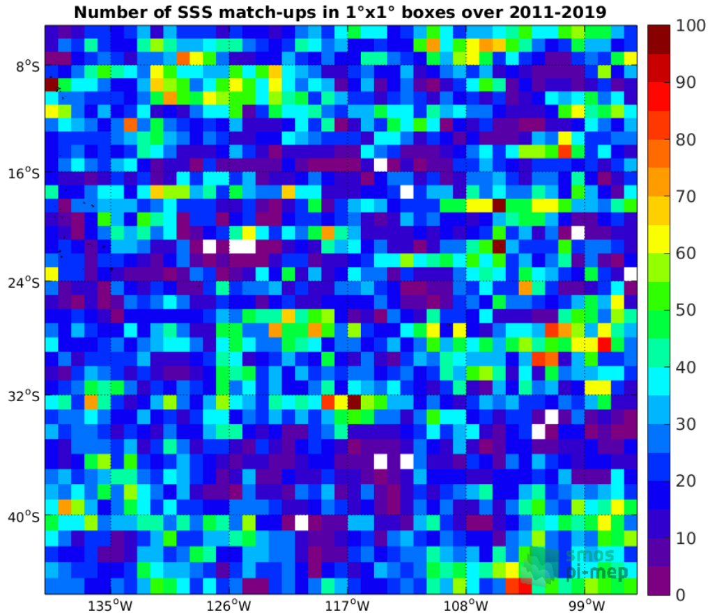
Figure 4: Number of SSS match-ups between Argo SSS and the SMOS L3 v2 - 9-Days (BEC) SSS product for the OTT zone Pi-MEP region over 1°x1° boxes and for the full satellite product period.
