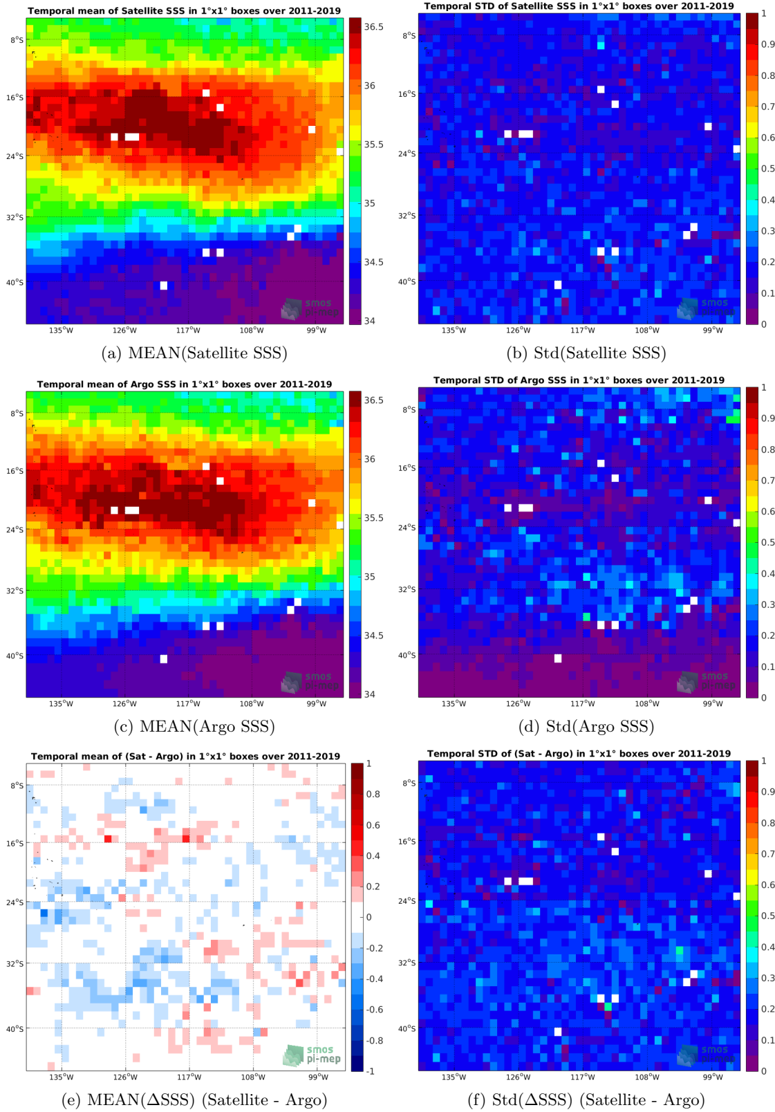
Figure 6: Temporal mean (left) and Std (right) of SSS from SMOS L3 v2 - 9-Days (BEC) (top), Argo (middle), and of \Delta SSS (Satellite - Argo). 22 Only match-up pairs are used to generate these maps.
