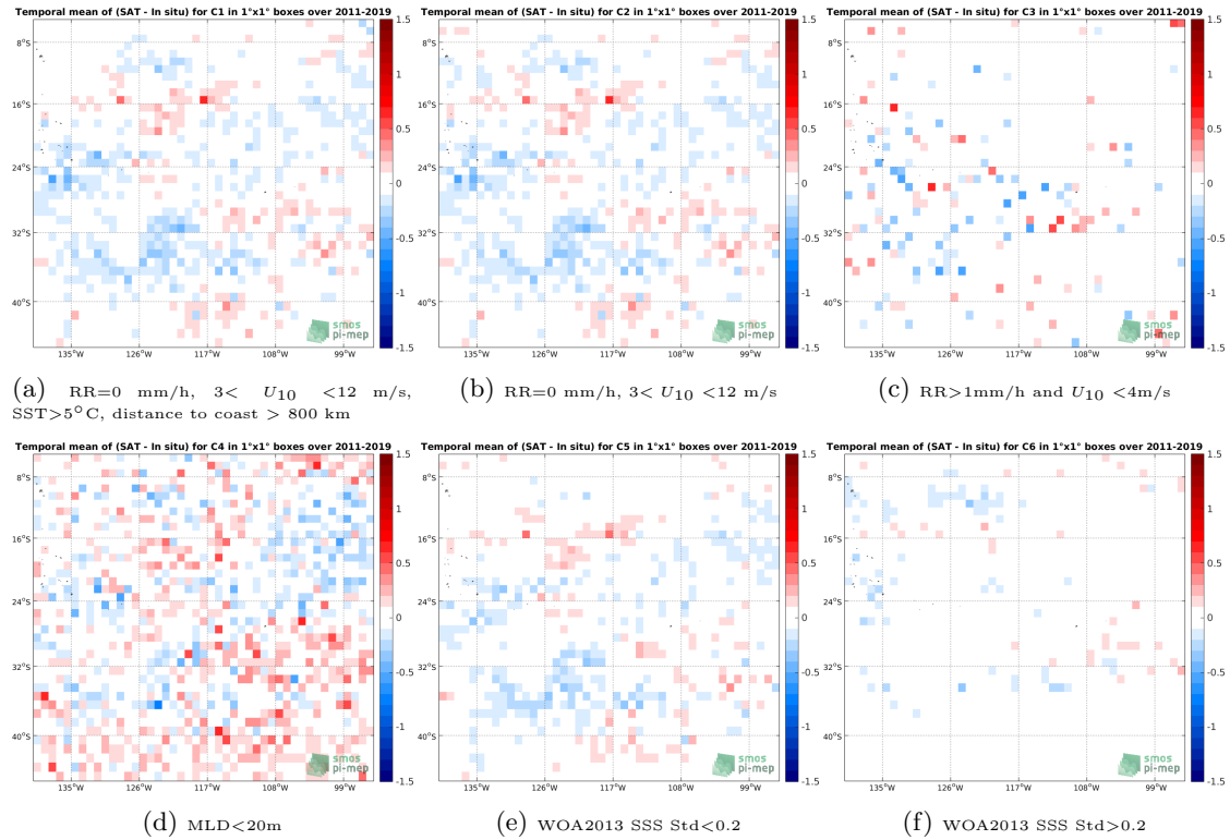
Figure 12: Temporal mean gridded over spatial boxes of size 1^\circ \times 1^\circ of \Delta SSS (SMOS L3 v2 - 9-Days (BEC) - Argo) for 6 different subdatasets corresponding to:RR=0 mm/h, 3 < U_{10} < 12 m/s, SST > 5^\circ\text{C} , distance to coast > 800 km (a), RR=0 mm/h, 3 < U_{10} < 12 m/s (b), RR > 1 mm/h and U_{10} < 4 m/s (c),MLD < 20 m (d),WOA2013 SSS Std < 0.2 (e),WOA2013 SSS Std > 0.2 (f).
