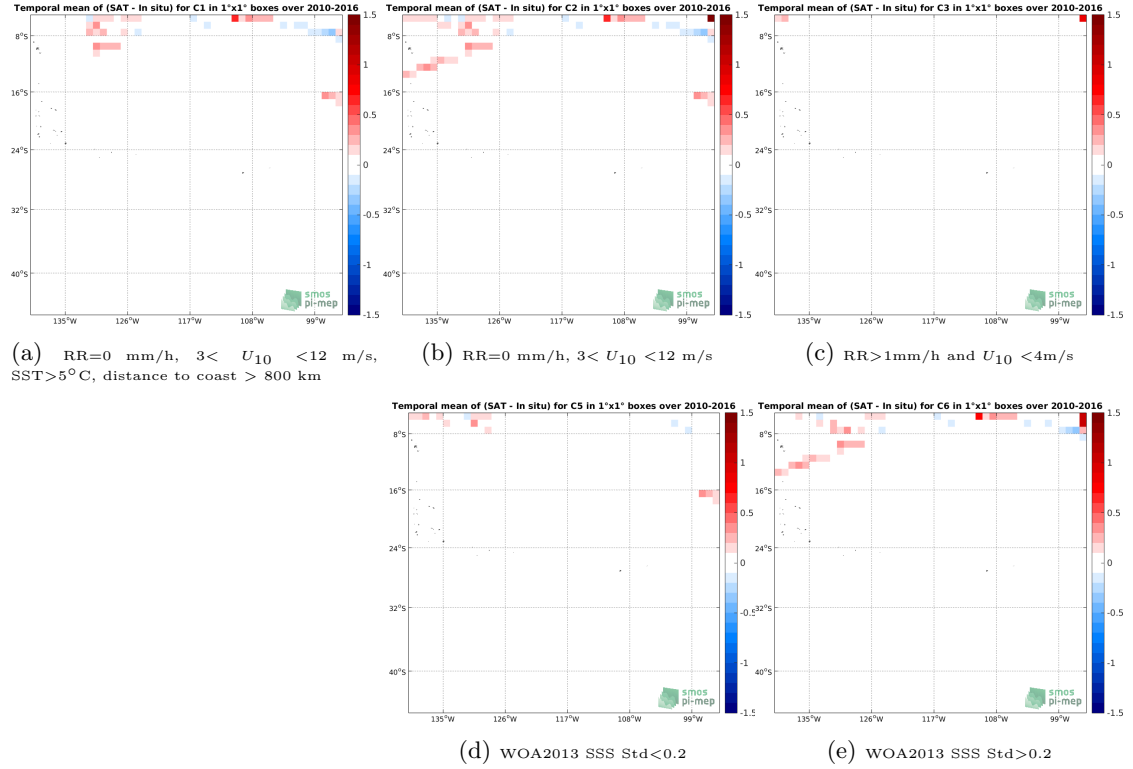
Figure 12: Temporal mean gridded over spatial boxes of size 1^\circ \times 1^\circ of \Delta SSS (SMOS-L3-BEC-OA-V1-9DAYS-0.25DEG - TSG-SAMOS) for 5 different subdatasets corresponding to:RR=0 mm/h, 3 < U_{10} < 12 m/s, SST >5^\circ C, distance to coast > 800 km (a), RR=0 mm/h, 3 < U_{10} < 12 m/s (b), RR >1 mm/h and U_{10} < 4 m/s (c), WOA2013 SSS Std <0.2 (d), WOA2013 SSS Std >0.2 (e).
