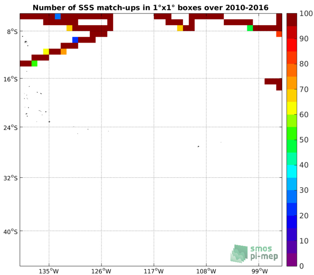
Figure 4: Number of SSS match-ups between TSG-SAMOS SSS and the SMOS-L3-BEC-OA-V1-9DAYS-0.25DEG SSS product for the OTT zone Pi-MEP region over 1°x1° boxes and for the full satellite product period.
