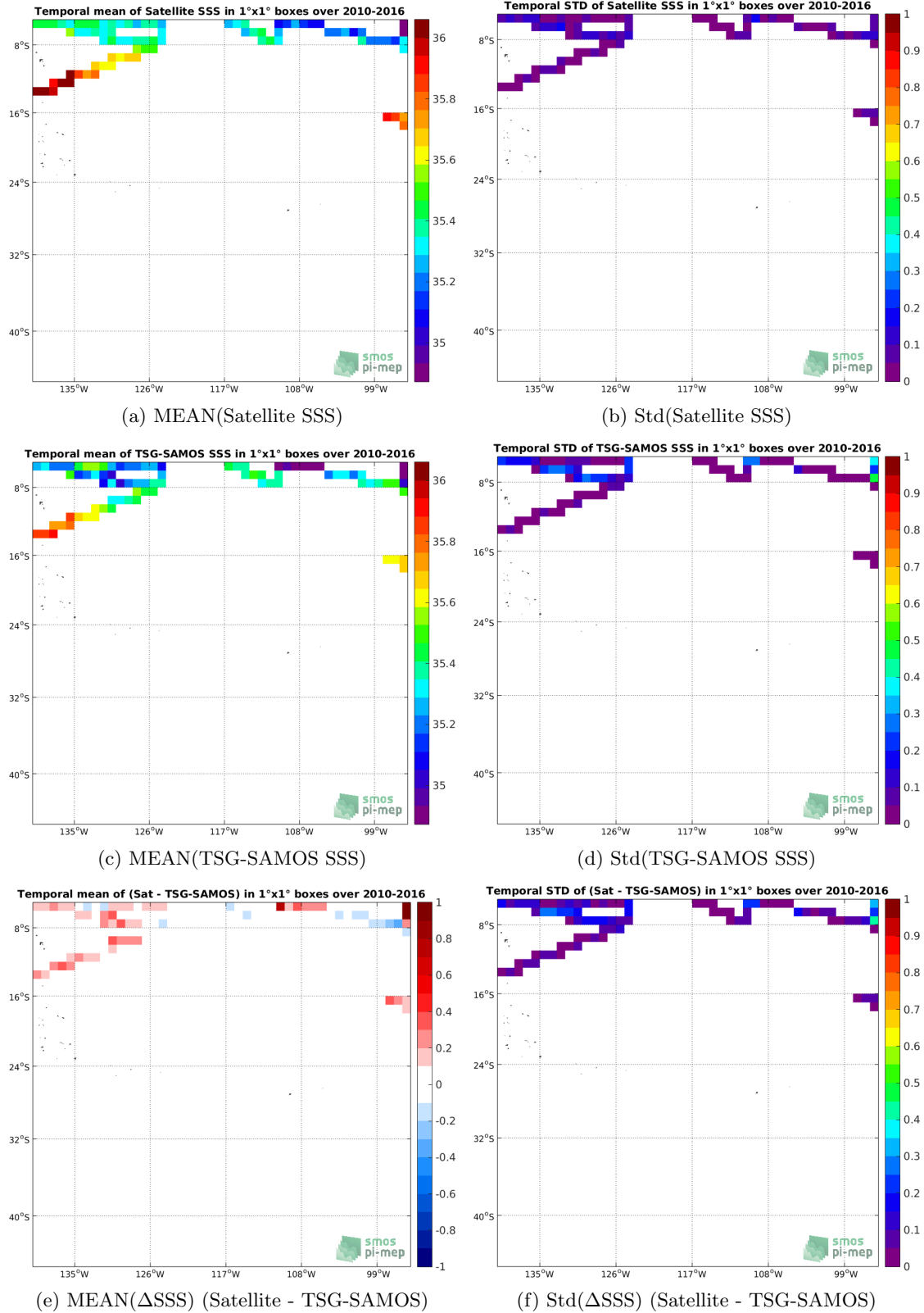
Figure 6: Temporal mean (left) and Std (right) of SSS from SMOS-L3-BEC-OA-V1-9DAYS-0.25DEG (top), TSG-SAMOS (middle), and of \Delta SSS (Satellite - TSG-SAMOS). Only match-up pairs are used to generate these maps.
