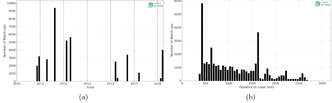
Figure 1: Number of match-ups between TSG-SAMOS and SMOS-L3-BEC-OA-V1-9DAYS-0.25DEG SSS as a function of time (a) and as function of the distance to coast (b) over the OTT zone Pi-MEP region and for the full satellite product period.
