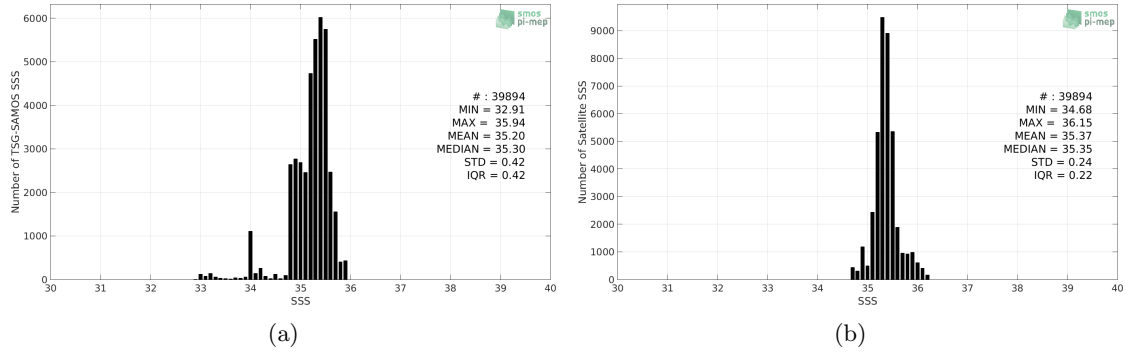
Figure 2: Histograms of SSS from TSG-SAMOS (a) and SMOS-L3-BEC-OA-V1-9DAYS-0.25DEG (b) considering all match-up pairs per bins of 0.1 over the OTT zone Pi-MEP region and for the full satellite product period.
