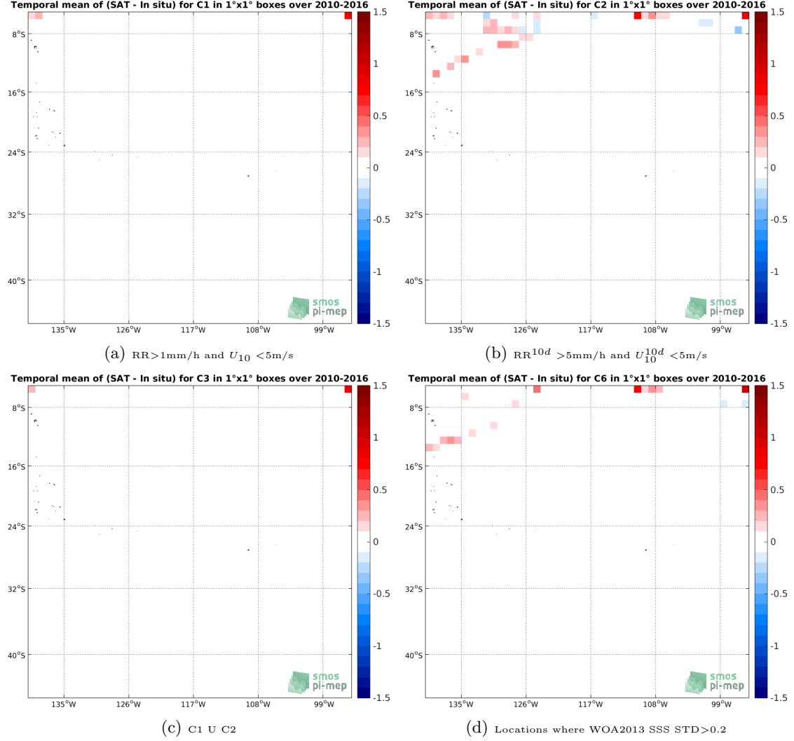
Figure 12: Temporal mean gridded over spatial boxes of size 1^\circ \times 1^\circ of \Delta SSS (SMOS-L3-BEC-OA-V1-9DAYS-0.25DEG - TSG-SAMOS) for 4 different subdatasets corresponding to: RR > 1mm/h and U_{10} < 5\text{m/s} (a), RR^{10d} > 5\text{mm/h} and U_{10}^{10d} < 5\text{m/s} (b), C1 U C2 (c), Locations where WOA2013 SSS STD > 0.2 (d).
