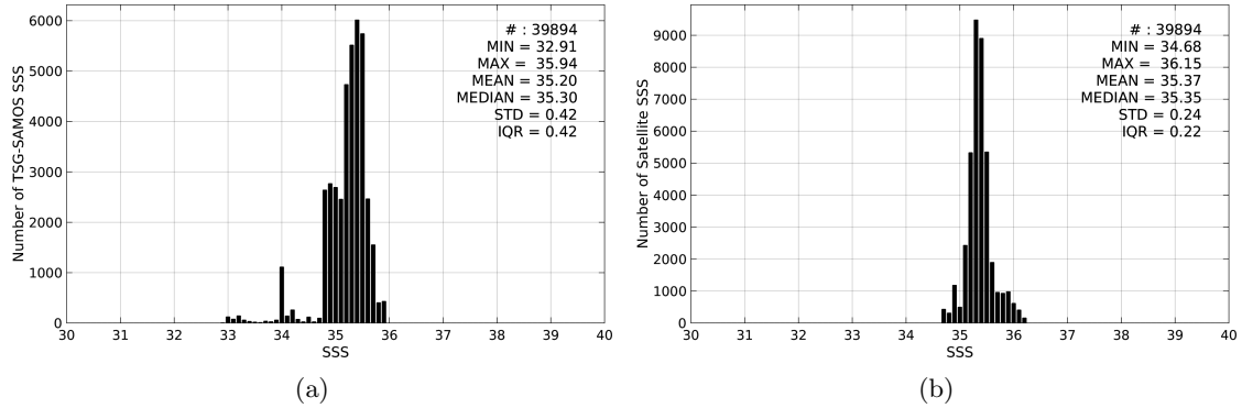
Figure 2: Histograms of SSS from TSG-SAMOS (a) and SMOS-L3-BEC-OA-V1-9DAYS-0.25DEG (b) considering all match-up pairs per bins of 0.1 over the OTT zone Pi-MEP region and for the full satellite product period.
