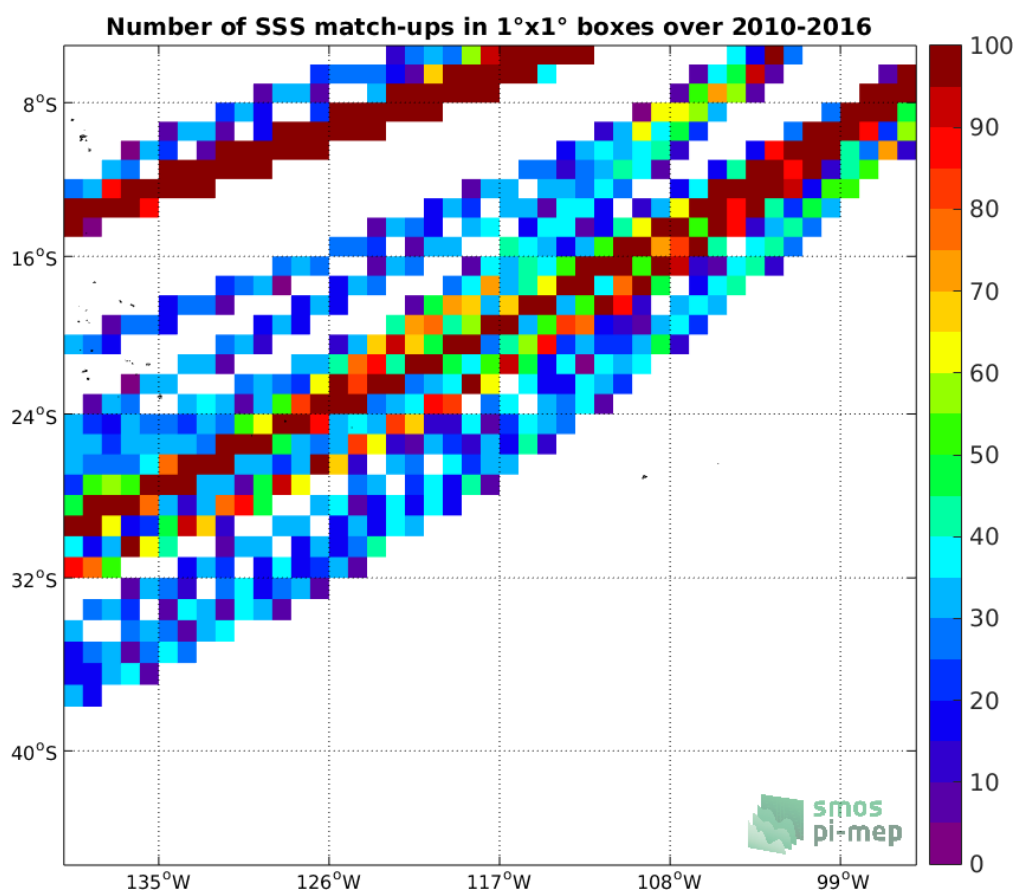
Figure 4: Number of SSS match-ups between TSG-LEGOS-DM SSS and the SMOS-L3-BEC-OA-V1-9DAYS-0.25DEG SSS product for the OTT zone Pi-MEP region over 1°x1° boxes and for the full satellite product period.
