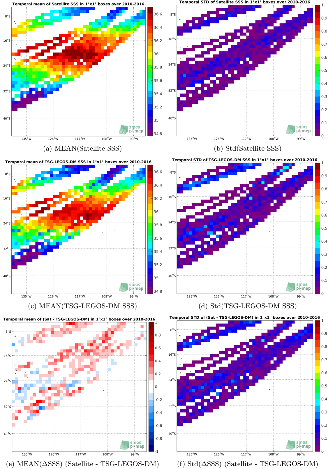
Figure 6: Temporal mean (left) and Std (right) of SSS from SMOS-L3-BEC-OA-V1-9DAYS-0.25DEG (top), TSG-LEGOS-DM (middle), and of \Delta SSS (Satellite - TSG-LEGOS-DM). Only match-up pairs are used to generate these maps.
