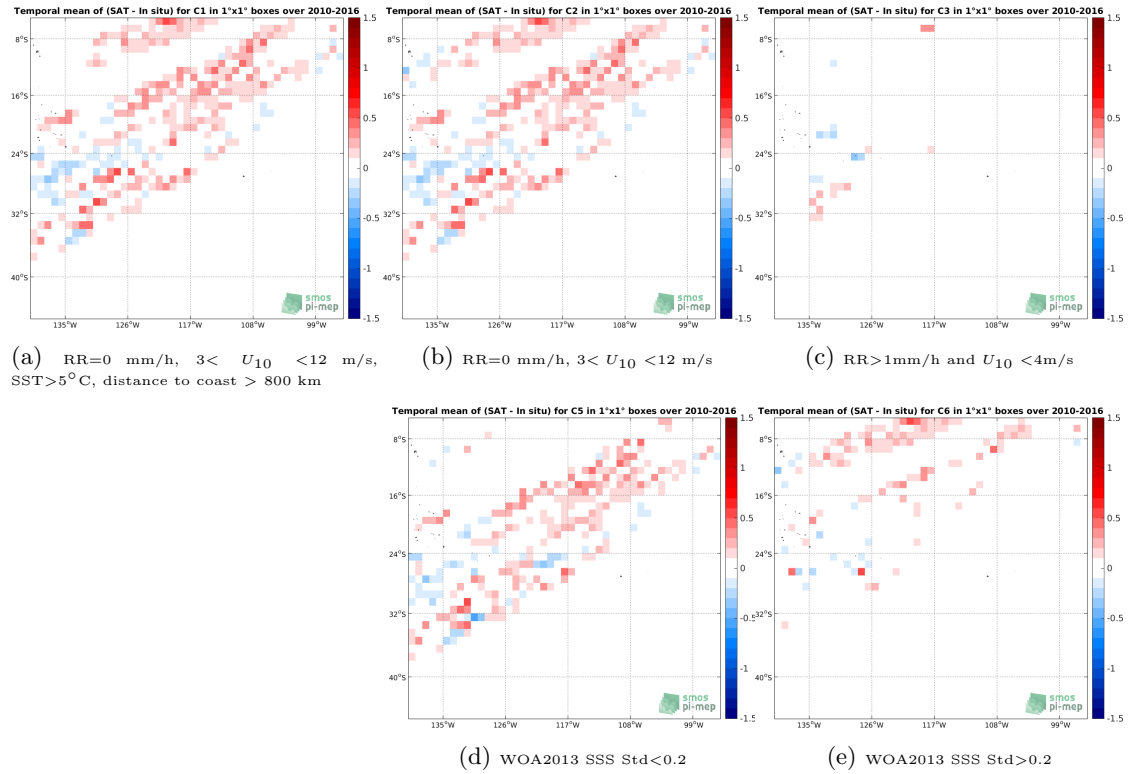
Figure 12: Temporal mean gridded over spatial boxes of size 1^\circ \times 1^\circ of \Delta SSS (SMOS-L3-BEC-OA-V1-9DAYS-0.25DEG - TSG-LEGOS-DM) for 5 different subdatasets corresponding to:RR=0 mm/h, 3 < U_{10} < 12 m/s, SST >5^\circ C, distance to coast > 800 km (a), RR=0 mm/h, 3 < U_{10} < 12 m/s (b), RR >1 mm/h and U_{10} < 4 m/s (c), WOA2013 SSS Std <0.2 (d), WOA2013 SSS Std >0.2 (e).
