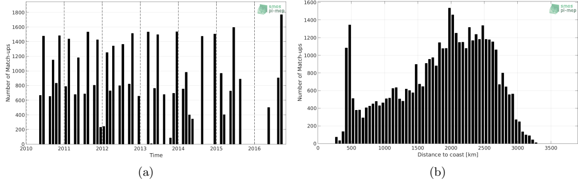
Figure 1: Number of match-ups between TSG-LEGOS-DM and SMOS-L3-BEC-OA-V1-9DAYS-0.25DEG SSS as a function of time (a) and as function of the distance to coast (b) over the OTT zone Pi-MEP region and for the full satellite product period.
