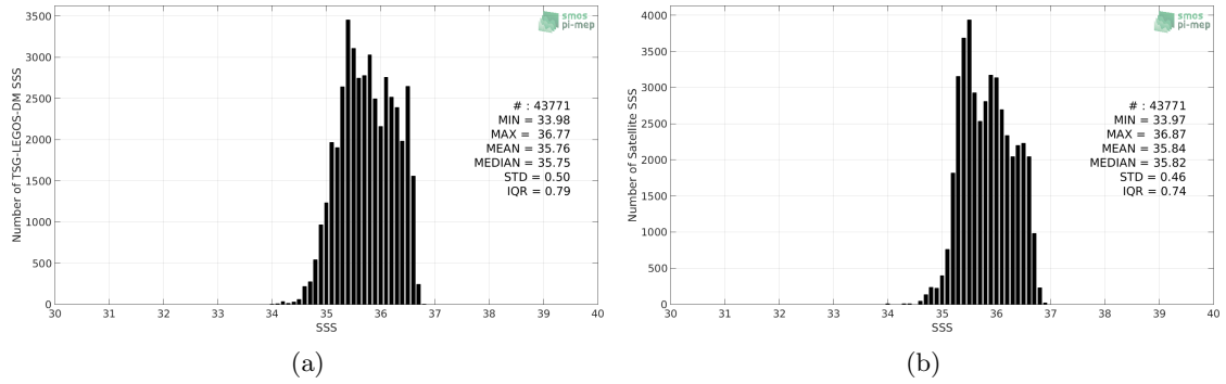
Figure 2: Histograms of SSS from TSG-LEGOS-DM (a) and SMOS-L3-BEC-OA-V1-9DAYS-0.25DEG (b) considering all match-up pairs per bins of 0.1 over the OTT zone Pi-MEP region and for the full satellite product period.
