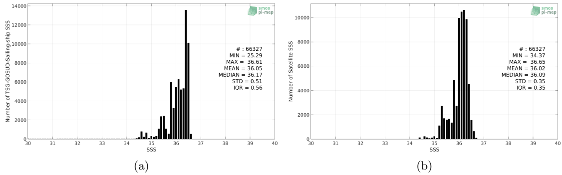
Figure 2: Histograms of SSS from TSG-GOSUD-Sailing-ship (a) and SMOS-L3-BEC-OA-V1-9DAYS-0.25DEG (b) considering all match-up pairs per bins of 0.1 over the OTT zone Pi-MEP region and for the full satellite product period.
