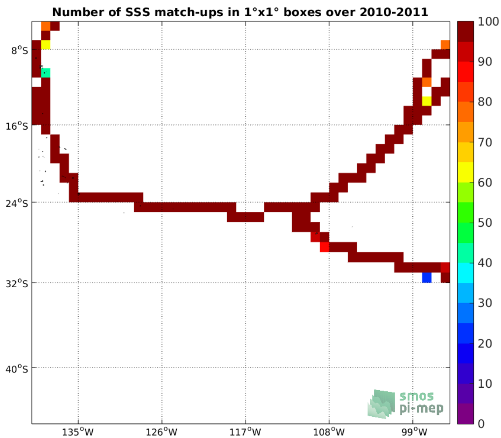
Figure 4: Number of SSS match-ups between TSG-GOSUD-Sailing-ship SSS and the SMOS-L3-BEC-OA-V1-9DAYS-0.25DEG SSS product for the OTT zone Pi-MEP region over 1°x1° boxes and for the full satellite product period.
