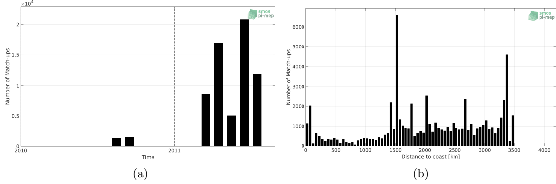
Figure 1: Number of match-ups between TSG-GOSUD-Sailing-ship and SMOS-L3-BEC-OA-V1-9DAYS-0.25DEG SSS as a function of time (a) and as function of the distance to coast (b) over the OTT zone Pi-MEP region and for the full satellite product period.
