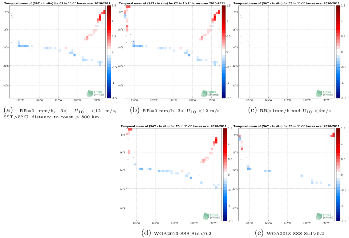
Figure 12: Temporal mean gridded over spatial boxes of size 1^\circ \times 1^\circ of \Delta SSS (SMOS-L3-BEC-OA-V1-9DAYS-0.25DEG - TSG-GOSUD-Sailing-ship) for 5 different subdatasets corresponding to:RR=0 mm/h, 3 < U_{10} < 12 m/s, SST >5^\circ\text{C} , distance to coast > 800 km (a), RR=0 mm/h, 3 < U_{10} < 12 m/s (b), RR >1 mm/h and U_{10} < 4 m/s (c), WOA2013 SSS Std <0.2 (d), WOA2013 SSS Std >0.2 (e).
