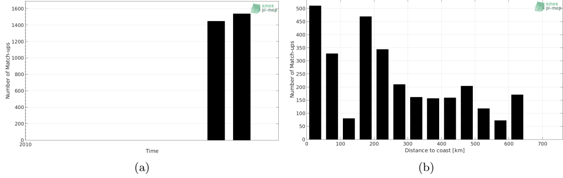
Figure 1: Number of match-ups between TSG-GOSUD-Sailing-ship and SMOS-L3-BEC-OA-V1-9DAYS-0.25DEG SSS as a function of time (a) and as function of the distance to coast (b) over the OTT zone Pi-MEP region and for the full satellite product period.
