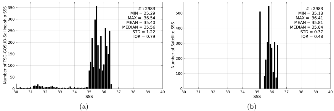
Figure 2: Histograms of SSS from TSG-GOSUD-Sailing-ship (a) and SMOS-L3-BEC-OA-V1-9DAYS-0.25DEG (b) considering all match-up pairs per bins of 0.1 over the OTT zone Pi-MEP region and for the full satellite product period.
