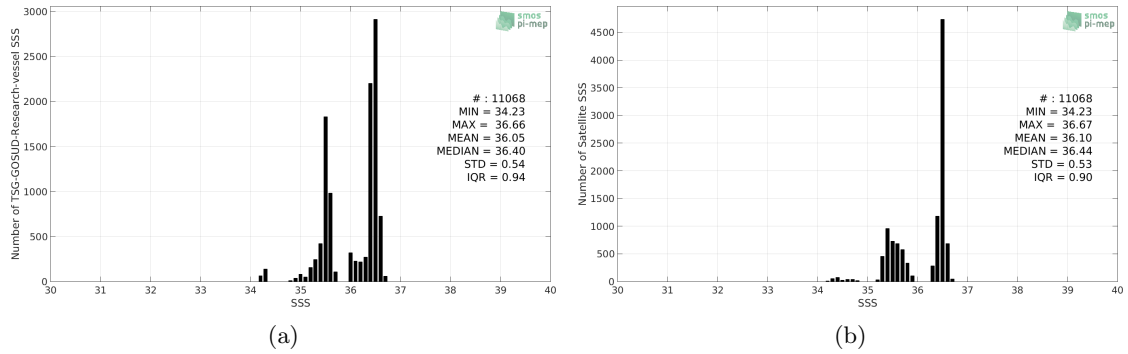
Figure 2: Histograms of SSS from TSG-GOSUD-Research-vessel (a) and SMOS-L3-BEC-OA-V1-9DAYS-0.25DEG (b) considering all match-up pairs per bins of 0.1 over the OTT zone Pi-MEP region and for the full satellite product period.
