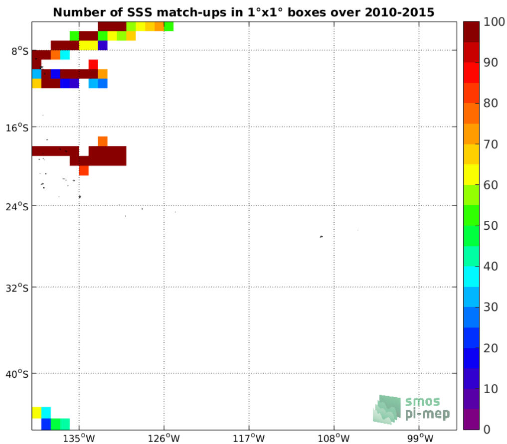
Figure 4: Number of SSS match-ups between TSG-GOSUD-Research-vessel SSS and the SMOS-L3-BEC-OA-V1-9DAYS-0.25DEG SSS product for the OTT zone Pi-MEP region over 1°x1° boxes and for the full satellite product period.
