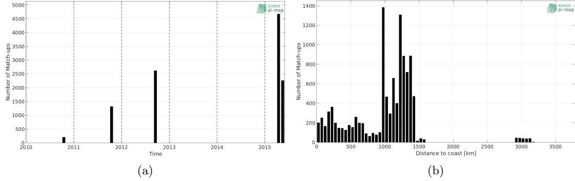
Figure 1: Number of match-ups between TSG-GOSUD-Research-vessel and SMOS-L3-BEC-OA-V1-9DAYS-0.25DEG SSS as a function of time (a) and as function of the distance to coast (b) over the OTT zone Pi-MEP region and for the full satellite product period.
