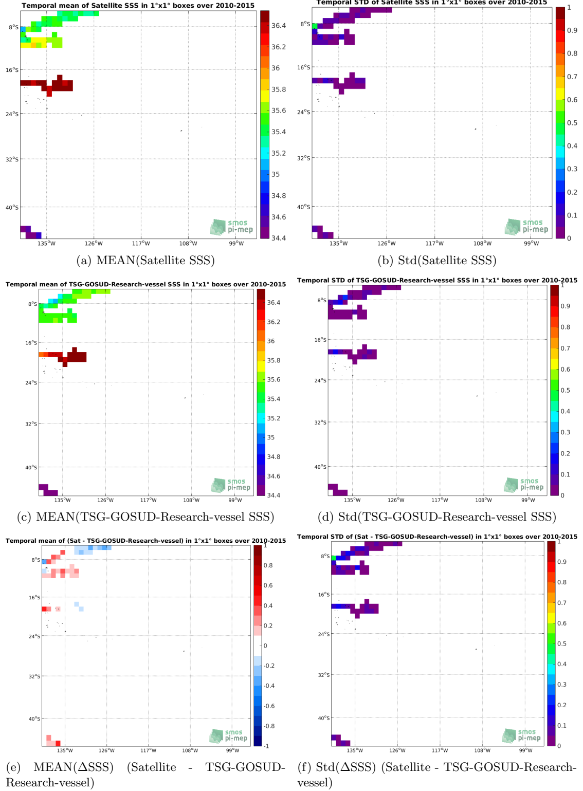
Figure 6: Temporal mean (left) and Std (right) of SSS from SMOS-L3-BEC-OA-V1-9DAYS-0.25DEG (top), TSG-GOSUD-Research-vessel (middle), and of \Delta SSS (Satellite - TSG-GOSUD-Research-vessel). Only match-up pairs are used to generate these maps.
