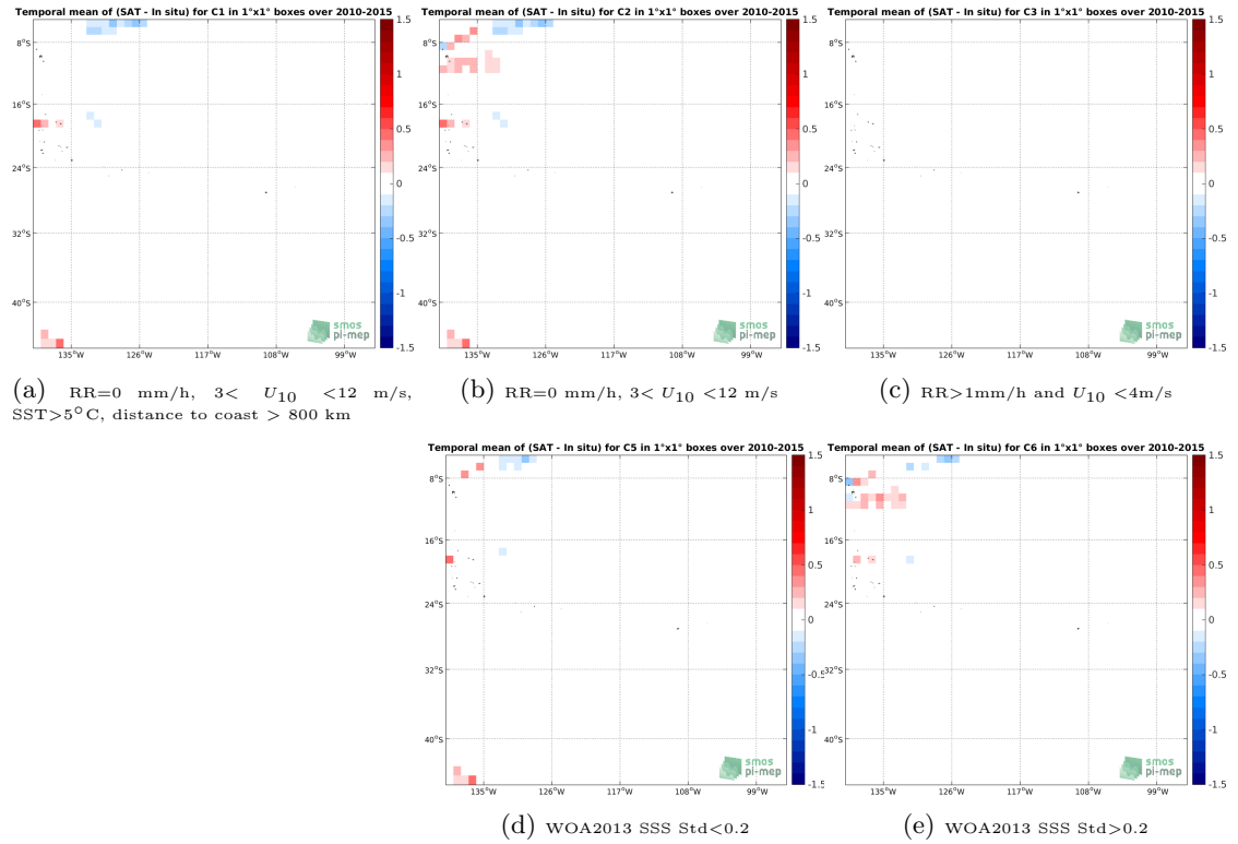
Figure 12: Temporal mean gridded over spatial boxes of size 1^\circ \times 1^\circ of \Delta SSS (SMOS-L3-BEC-OA-V1-9DAYS-0.25DEG - TSG-GOSUD-Research-vessel) for 5 different subdatasets corresponding to:RR=0 mm/h, 3 < U_{10} < 12 m/s, SST >5^\circ\text{C} , distance to coast > 800 km (a), RR=0 mm/h, 3 < U_{10} < 12 m/s (b), RR >1 mm/h and U_{10} < 4 m/s (c), WOA2013 SSS Std <0.2 (d), WOA2013 SSS Std >0.2 (e).
