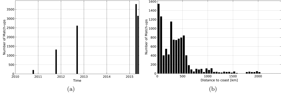
Figure 1: Number of match-ups between TSG-GOSUD-Research-vessel and SMOS-L3-BEC-OA-V1-9DAYS-0.25DEG SSS as a function of time (a) and as function of the distance to coast (b) over the OTT zone Pi-MEP region and for the full satellite product period.
