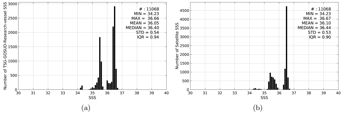
Figure 2: Histograms of SSS from TSG-GOSUD-Research-vessel (a) and SMOS-L3-BEC-OA-V1-9DAYS-0.25DEG (b) considering all match-up pairs per bins of 0.1 over the OTT zone Pi-MEP region and for the full satellite product period.
