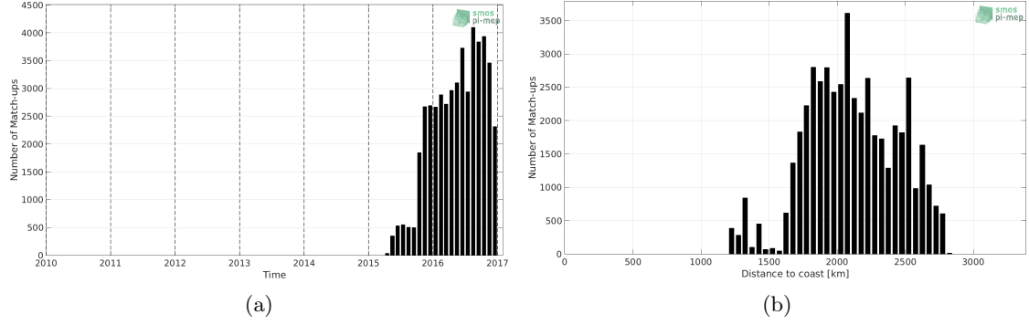
Figure 1: Number of match-ups between Surface drifters and SMOS-L3-BEC-OA-V1-9DAYS-0.25DEG SSS as a function of time (a) and as function of the distance to coast (b) over the OTT zone Pi-MEP region and for the full satellite product period.
