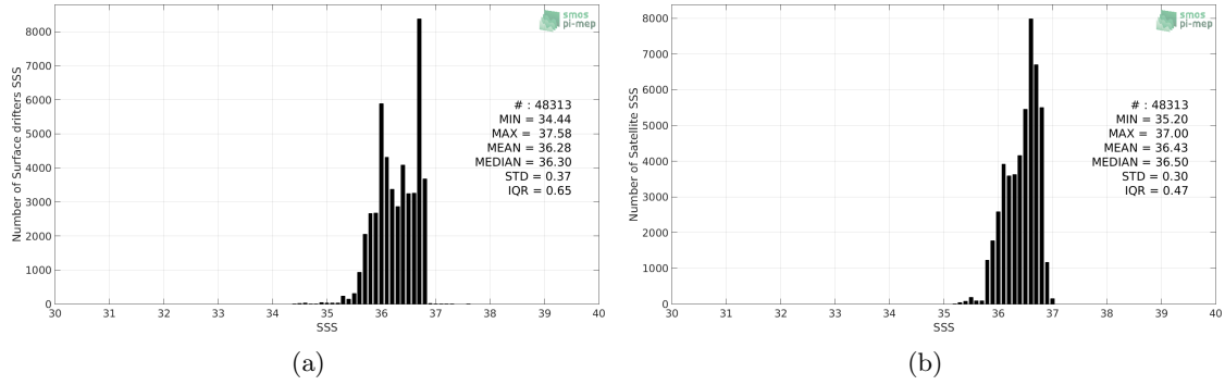
Figure 2: Histograms of SSS from Surface drifters (a) and SMOS-L3-BEC-OA-V1-9DAYS-0.25DEG (b) considering all match-up pairs per bins of 0.1 over the OTT zone Pi-MEP region and for the full satellite product period.
