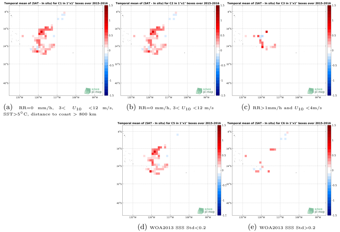
Figure 11: Temporal mean gridded over spatial boxes of size 1^\circ \times 1^\circ of \Delta SSS (SMOS-L3-BEC-OA-V1-9DAYS-0.25DEG - Surface drifters) for 5 different subdatasets corresponding to: RR=0 mm/h, 3 < U_{10} < 12 m/s, SST > 5^\circ C , distance to coast > 800 km (a), RR=0 mm/h, 3 < U_{10} < 12 m/s (b), RR > 1 mm/h and U_{10} < 4 m/s (c), WOA2013 SSS Std < 0.2 (d), WOA2013 SSS Std > 0.2 (e).
