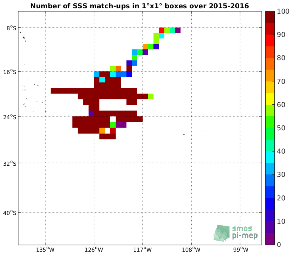
Figure 3: Number of SSS match-ups between Surface drifters SSS and the SMOS-L3-BEC-OA-V1-9DAYS-0.25DEG SSS product for the OTT zone Pi-MEP region over 1°x1° boxes and for the full satellite product period.
