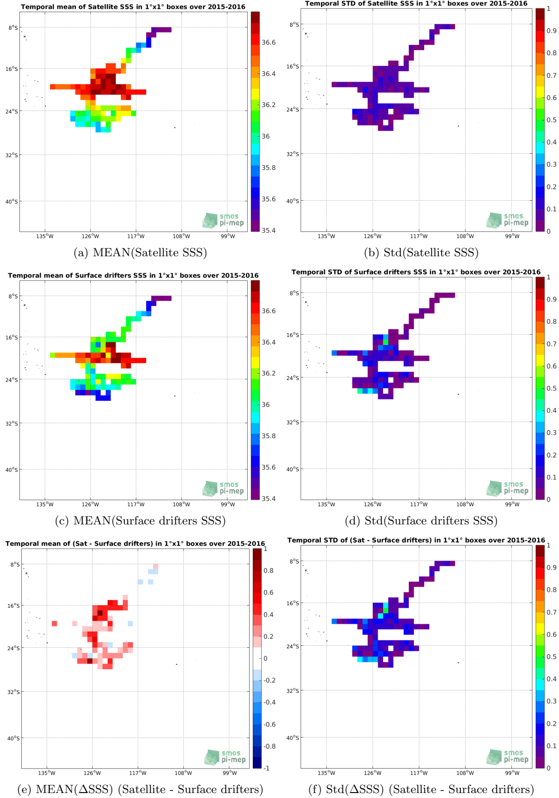
Figure 5: Temporal mean (left) and Std (right) of SSS from SMOS-L3-BEC-OA-V1-9DAYS-0.25DEG (top), Surface drifters (middle), and of \Delta SSS (Satellite - Surface drifters). Only match-up pairs are used to generate these maps.
