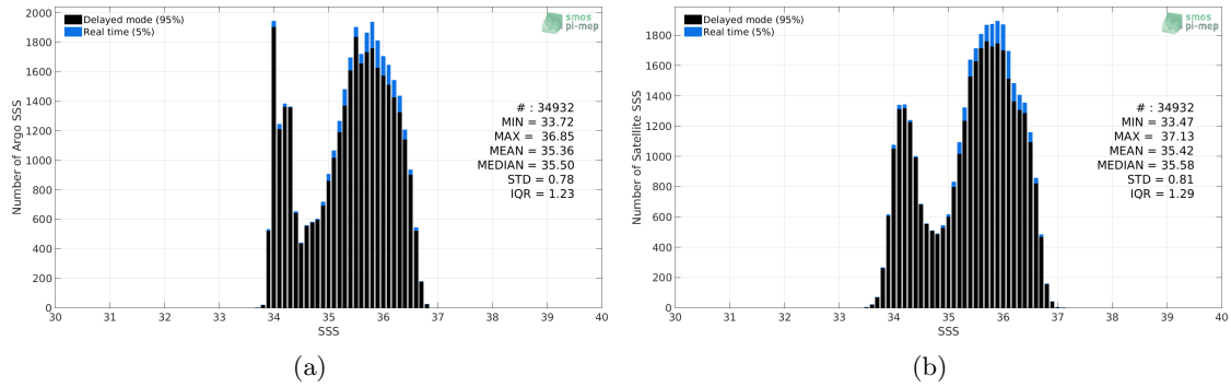
Figure 2: Histograms of SSS from Argo (a) and SMOS-L3-BEC-OA-V1-9DAYS-0.25DEG (b) considering all match-up pairs per bins of 0.1 over the OTT zone Pi-MEP region and for the full satellite product period.
