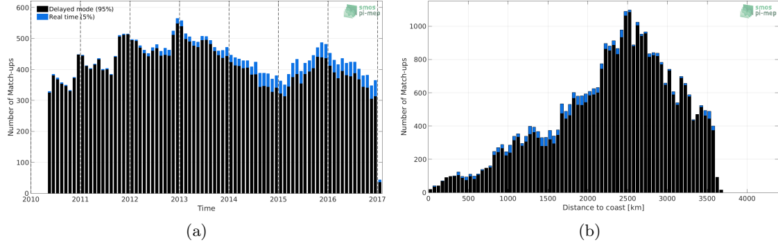
Figure 1: Number of match-ups between Argo and SMOS-L3-BEC-OA-V1-9DAYS-0.25DEG SSS as a function of time (a) and as function of the distance to coast (b) over the OTT zone Pi-MEP region and for the full satellite product period.
