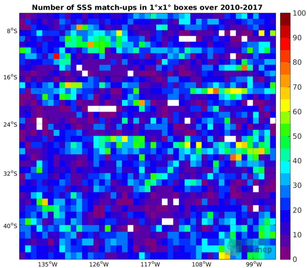
Figure 4: Number of SSS match-ups between Argo SSS and the SMOS-L3-BEC-OA-V1-9DAYS-0.25DEG SSS product for the OTT zone Pi-MEP region over 1°x1° boxes and for the full satellite product period.
