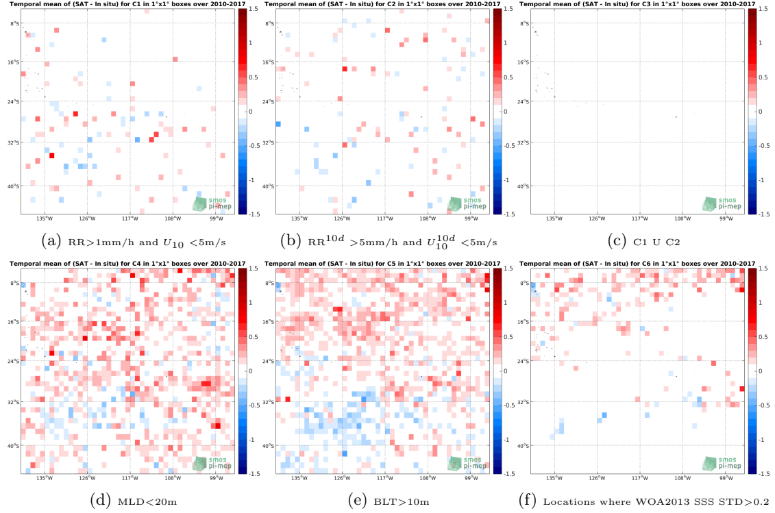
Figure 12: Temporal mean gridded over spatial boxes of size 1^\circ \times 1^\circ of \Delta\text{SSS} (SMOS-L3-BEC-OA-V1-9DAYS-0.25DEG - Argo) for 6 different subdatasets corresponding to: \text{RR} > 1\text{mm/h} and U_{10} < 5\text{m/s} (a), \text{RR}^{10d} > 5\text{mm/h} and U_{10} < 5\text{m/s} (b), C1 U C2 (c), \text{MLD} < 20\text{m} (d), \text{BLT} > 10\text{m} (e), Locations where WOA2013 SSS STD > 0.2 (f).
