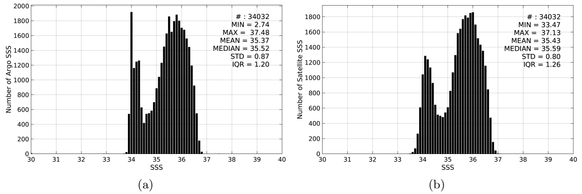
Figure 2: Histograms of SSS from Argo (a) and SMOS-L3-BEC-OA-V1-9DAYS-0.25DEG (b) considering all match-up pairs per bins of 0.1 over the OTT zone Pi-MEP region and for the full satellite product period.
