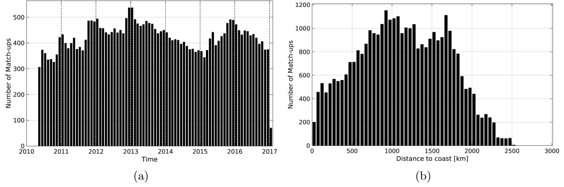
Figure 1: Number of match-ups between Argo and SMOS-L3-BEC-OA-V1-9DAYS-0.25DEG SSS as a function of time (a) and as function of the distance to coast (b) over the OTT zone Pi-MEP region and for the full satellite product period.
