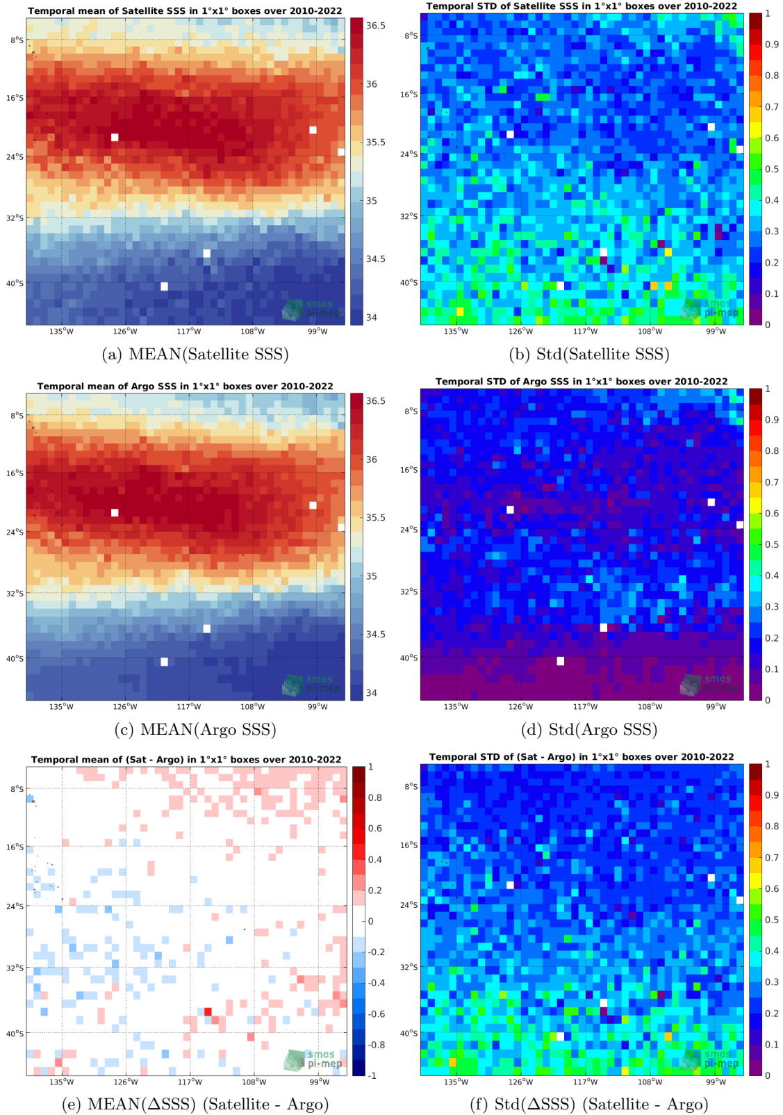
Figure 6: Temporal mean (left) and Std (right) of SSS from SMOS SSS L2-AVERAGED v700 (ESA) (top), Argo (middle), and of \Delta SSS (Satellite - Argo). Only match-up pairs are used to generate these maps.
