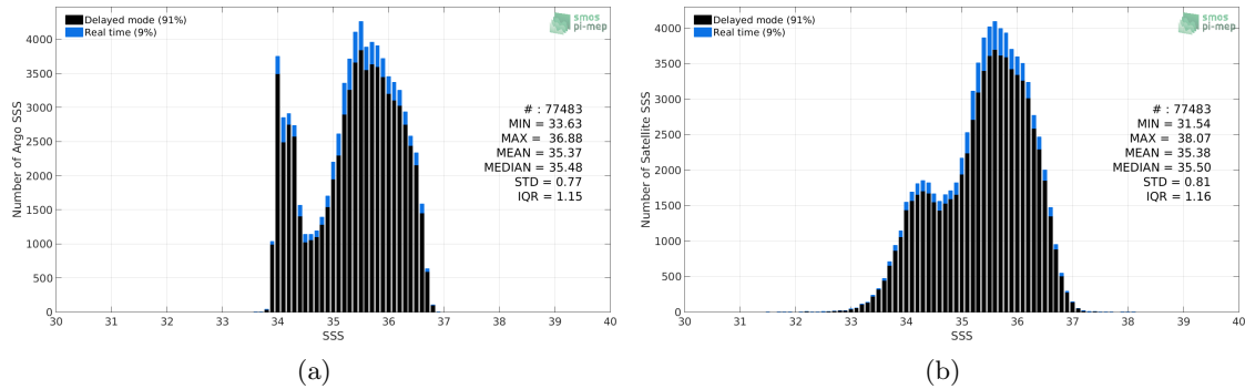
Figure 2: Histograms of SSS from Argo (a) and SMOS SSS L2-AVERAGED v700 (ESA) (b) considering all match-up pairs per bins of 0.1 over the OTT zone Pi-MEP region and for the full satellite product period.
