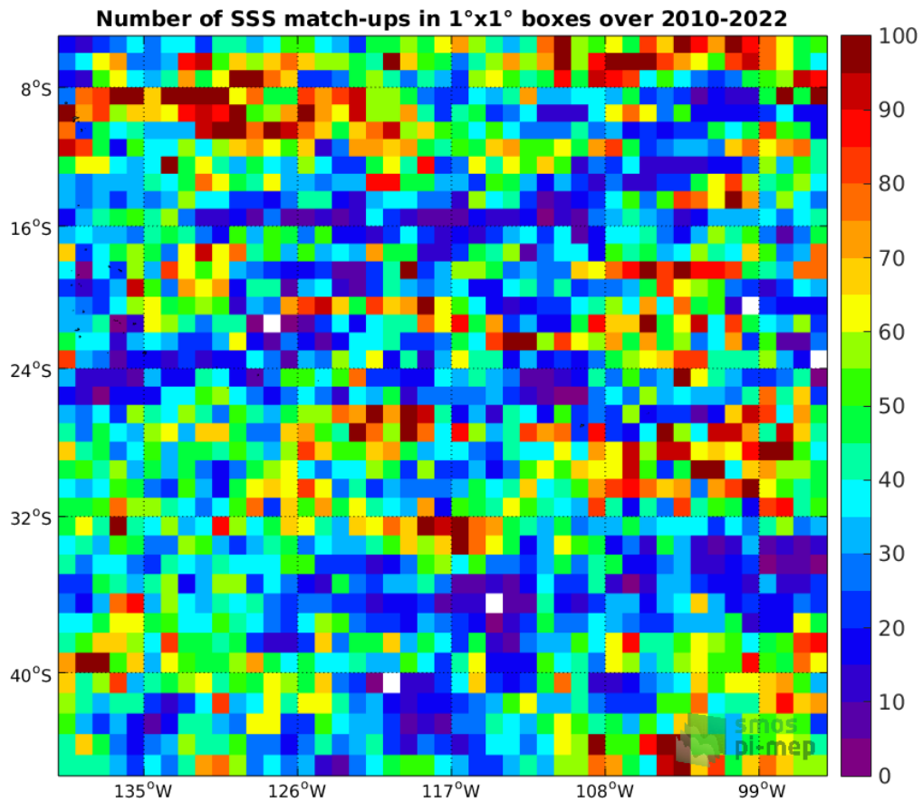
Figure 4: Number of SSS match-ups between Argo SSS and the SMOS SSS L2-AVERAGED v700 (ESA) SSS product for the OTT zone Pi-MEP region over 1°×1° boxes and for the full satellite product period.
