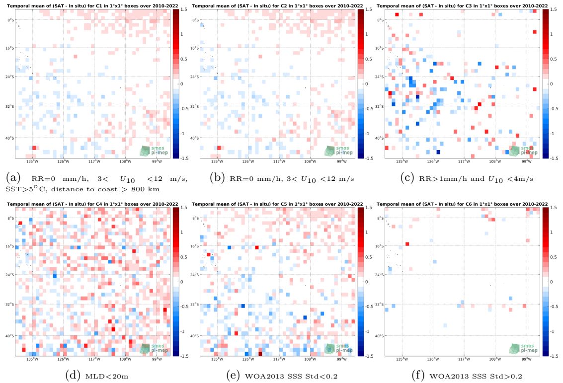
Figure 12: Temporal mean gridded over spatial boxes of size 1^\circ \times 1^\circ of \Delta SSS (SMOS SSS L2-AVERAGED v700 (ESA) - Argo) for 6 different subdatasets corresponding to:RR=0 mm/h, 3 < U_{10} < 12 m/s, SST >5^\circ C, distance to coast > 800 km (a), RR=0 mm/h, 3 < U_{10} < 12 m/s (b), RR >1 mm/h and U_{10} < 4 m/s (c),MLD <20 m (d),WOA2013 SSS Std <0.2 (e),WOA2013 SSS Std >0.2 (f).
