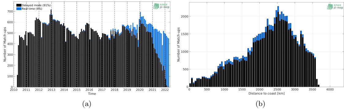
Figure 1: Number of match-ups between Argo and SMOS SSS L2-AVERAGED v700 (ESA) SSS as a function of time (a) and as function of the distance to coast (b) over the OTT zone Pi-MEP region and for the full satellite product period.
