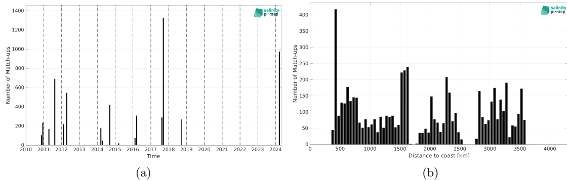
Figure 2: Number of match-ups between TSG (SAMOS) and SMOS SSS L2 v700 (ESA) SSS as a function of time (a) and as function of the distance to coast (b) over the OTT zone Pi-MEP region and for the full satellite product period.
