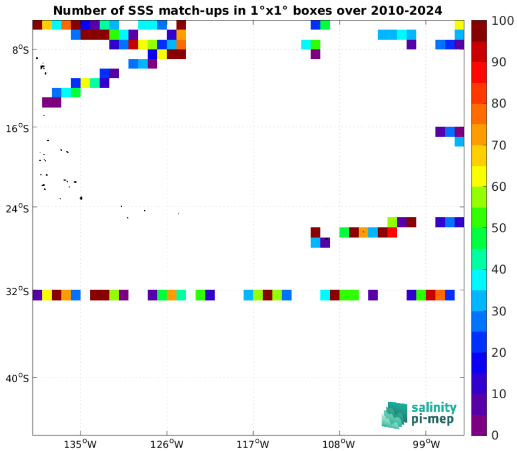
Figure 5: Number of SSS match-ups between TSG (SAMOS) SSS and the SMOS SSS L2 v700 (ESA) SSS product for the OTT zone Pi-MEP region over 1^\circ \times 1^\circ boxes and for the full satellite product period.
