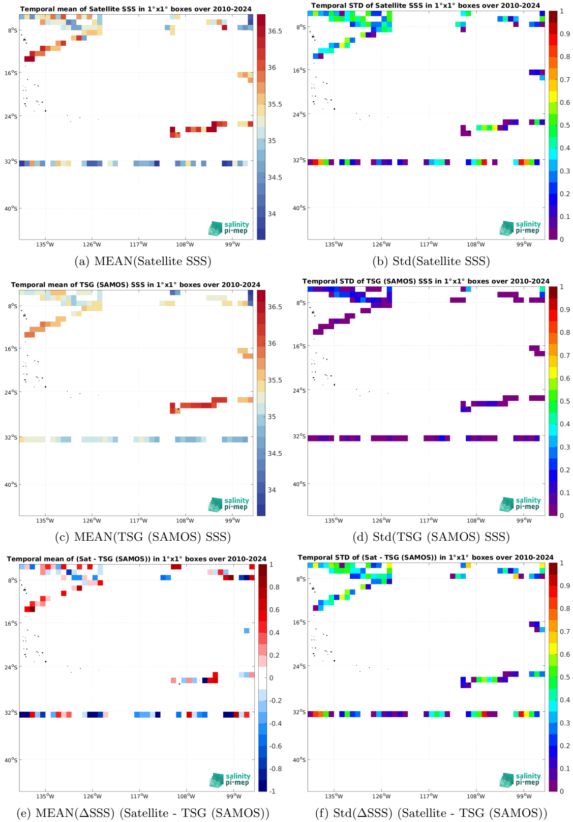
Figure 7: Temporal mean (left) and Std (right) of SSS from SMOS SSS L2 v700 (ESA) (top), TSG (SAMOS) (middle), and of \Delta SSS (Satellite - TSG (SAMOS)). Only match-up pairs are used to generate these maps.
