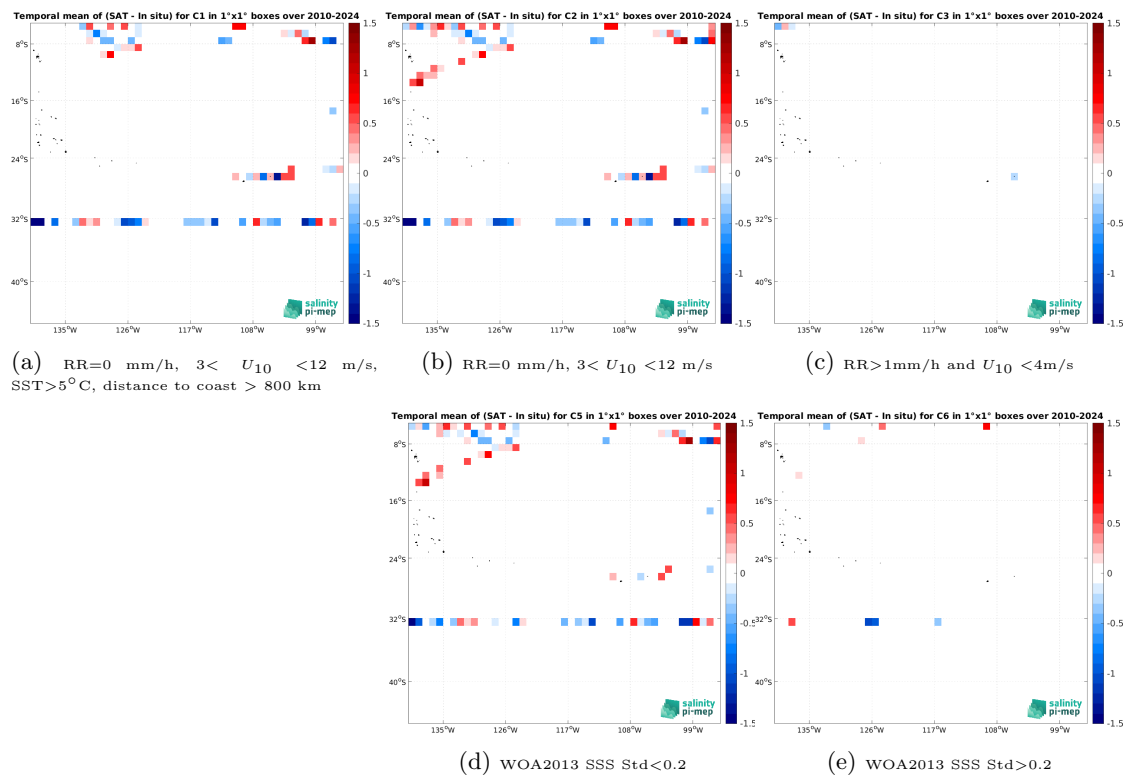
Figure 14: Temporal mean gridded over spatial boxes of size 1^\circ \times 1^\circ of \Delta SSS (SMOS SSS L2 v700 (ESA) - TSG (SAMOS)) for 5 different subdatasets corresponding to: RR=0 mm/h, 3 < U_{10} < 12 m/s, SST > 5^\circ C , distance to coast > 800 km (a), RR=0 mm/h, 3 < U_{10} < 12 m/s (b), RR > 1 mm/h and U_{10} < 4 m/s (c), WOA2013 SSS Std <0.2 (d), WOA2013 SSS Std >0.2 (e).
