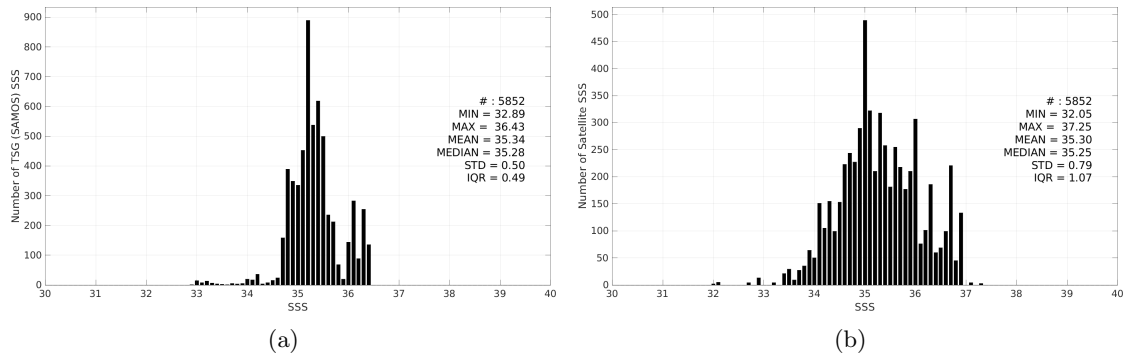
Figure 3: Histograms of SSS from TSG (SAMOS) (a) and SMOS SSS L2 v700 (ESA) (b) considering all match-up pairs per bins of 0.1 over the OTT zone Pi-MEP region and for the full satellite product period.
