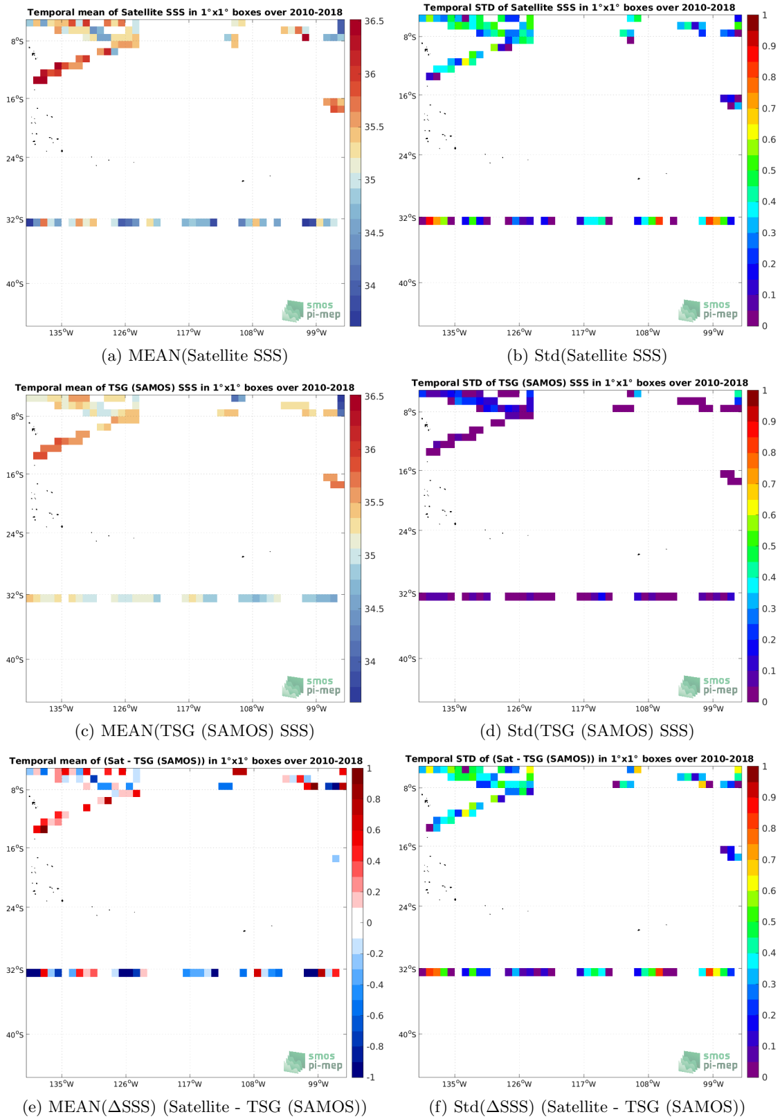
Figure 6: Temporal mean (left) and Std (right) of SSS from SMOS SSS L2 v700 (ESA) (top), TSG (SAMOS) (middle), and of \Delta SSS (Satellite - TSG (SAMOS)). Only match-up pairs are used to generate these maps.
