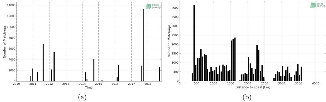
Figure 1: Number of match-ups between TSG (SAMOS) and SMOS SSS L2 v700 (ESA) SSS as a function of time (a) and as function of the distance to coast (b) over the OTT zone Pi-MEP region and for the full satellite product period.
