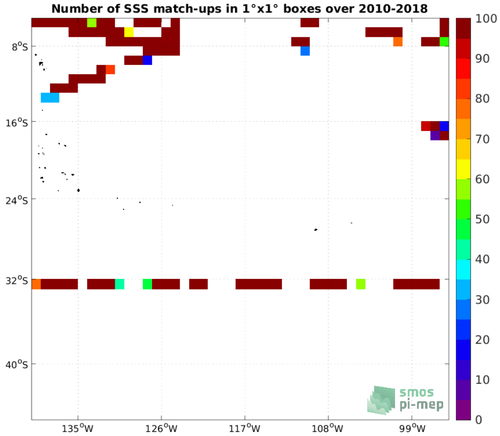
Figure 4: Number of SSS match-ups between TSG (SAMOS) SSS and the SMOS SSS L2 v700 (ESA) SSS product for the OTT zone Pi-MEP region over 1^\circ \times 1^\circ boxes and for the full satellite product period.
