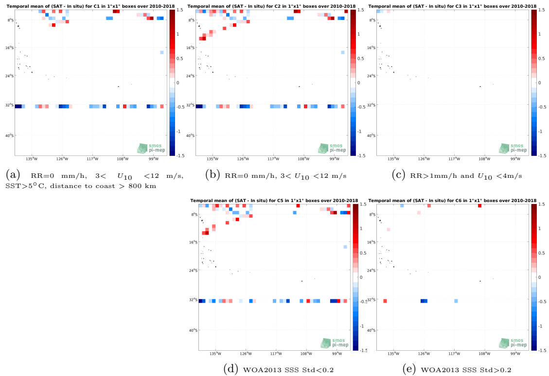
Figure 12: Temporal mean gridded over spatial boxes of size 1^\circ \times 1^\circ of \Delta SSS (SMOS SSS L2 v700 (ESA) - TSG (SAMOS)) for 5 different subdatasets corresponding to: RR=0 mm/h, 3 < U_{10} < 12 m/s, SST > 5^\circ C , distance to coast > 800 km (a), RR=0 mm/h, 3 < U_{10} < 12 m/s (b), RR > 1 mm/h and U_{10} < 4 m/s (c), WOA2013 SSS Std < 0.2 (d), WOA2013 SSS Std > 0.2 (e).
