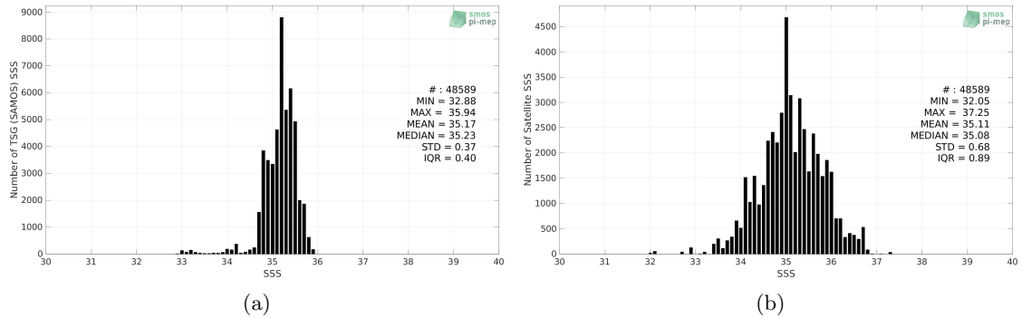
Figure 2: Histograms of SSS from TSG (SAMOS) (a) and SMOS SSS L2 v700 (ESA) (b) considering all match-up pairs per bins of 0.1 over the OTT zone Pi-MEP region and for the full satellite product period.
