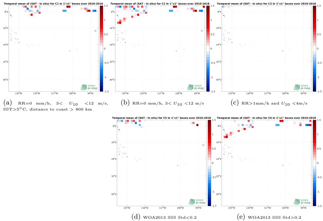
Figure 12: Temporal mean gridded over spatial boxes of size 1^\circ \times 1^\circ of \Delta SSS (SMOS SSS L2 v700 (ESA) - TSG (SAMOS)) for 5 different subdatasets corresponding to:RR=0 mm/h, 3 < U_{10} < 12 m/s, SST >5^\circ C, distance to coast > 800 km (a), RR=0 mm/h, 3 < U_{10} < 12 m/s (b), RR >1 mm/h and U_{10} < 4 m/s (c), WOA2013 SSS Std <0.2 (d), WOA2013 SSS Std >0.2 (e).
