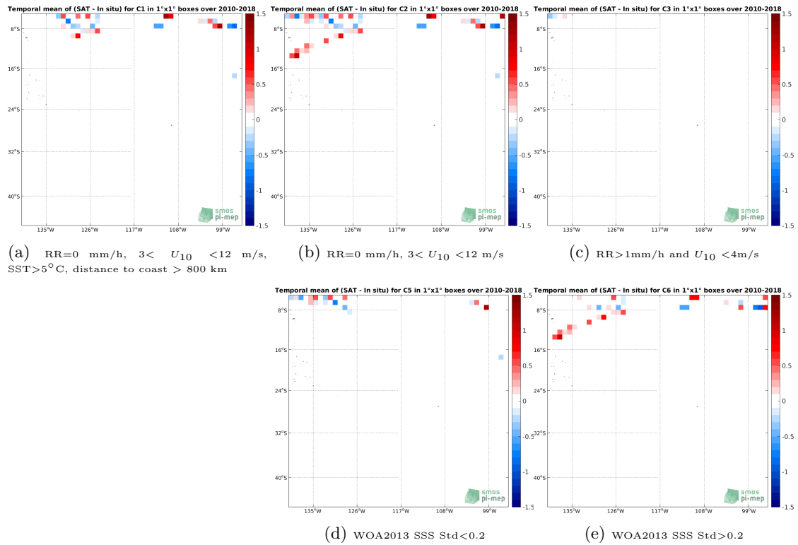
Figure 12: Temporal mean gridded over spatial boxes of size 1^\circ \times 1^\circ of \Delta\text{SSS} (SMOS SSS L2 v700 (ESA) - TSG (SAMOS)) for 5 different subdatasets corresponding to: \text{RR}=0 mm/h, 3 < U_{10} < 12 m/s, \text{SST} > 5^\circ\text{C} , distance to coast > 800 km (a), \text{RR}=0 mm/h, 3 < U_{10} < 12 m/s (b), \text{RR} > 1 mm/h and U_{10} < 4 m/s (c), WOA2013 SSS Std < 0.2 (d), WOA2013 SSS Std > 0.2 (e).
