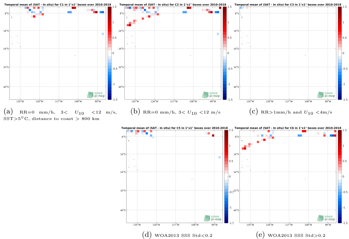
Figure 12: Temporal mean gridded over spatial boxes of size 1^\circ \times 1^\circ of \Delta\text{SSS} (SMOS SSS L2 v700 (ESA) - TSG (SAMOS)) for 5 different subdatasets corresponding to:RR=0 mm/h, 3 < U_{10} < 12 m/s, SST >5^\circ\text{C} , distance to coast > 800 km (a), RR=0 mm/h, 3 < U_{10} < 12 m/s (b), RR >1 mm/h and U_{10} < 4 m/s (c), WOA2013 SSS Std <0.2 (d), WOA2013 SSS Std >0.2 (e).
