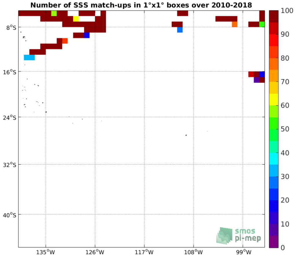
Figure 4: Number of SSS match-ups between TSG (SAMOS) SSS and the SMOS SSS L2 v700 (ESA) SSS product for the OTT zone Pi-MEP region over 1°x1° boxes and for the full satellite product period.
