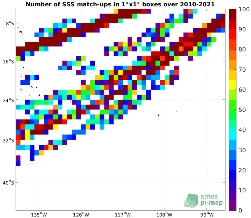
Figure 4: Number of SSS match-ups between TSG (LEGOS-DM) SSS and the SMOS SSS L2 v700 (ESA) SSS product for the OTT zone Pi-MEP region over 1°x1° boxes and for the full satellite product period.
