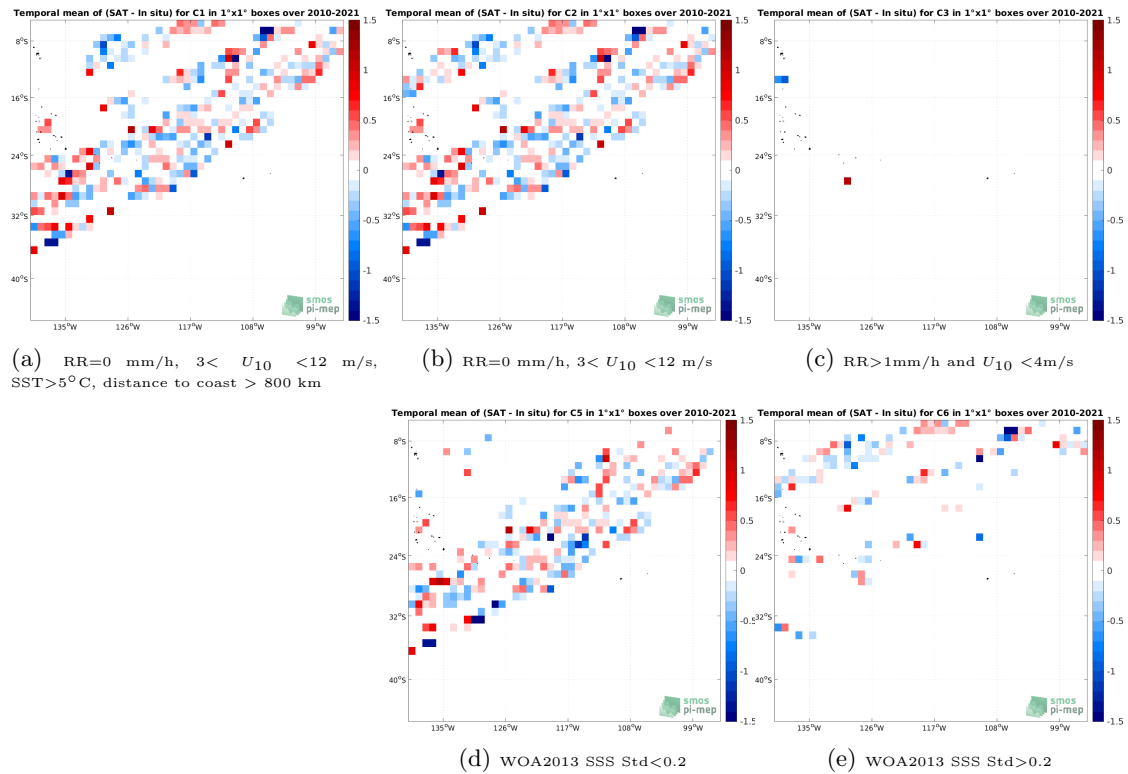
Figure 12: Temporal mean gridded over spatial boxes of size 1^\circ \times 1^\circ of \Delta SSS (SMOS SSS L2 v700 (ESA) - TSG (LEGOS-DM)) for 5 different subdatasets corresponding to:RR=0 mm/h, 3 < U_{10} < 12 m/s, SST >5^\circ C, distance to coast > 800 km (a), RR=0 mm/h, 3 < U_{10} < 12 m/s (b), RR >1 mm/h and U_{10} < 4 m/s (c), WOA2013 SSS Std <0.2 (d), WOA2013 SSS Std >0.2 (e).
