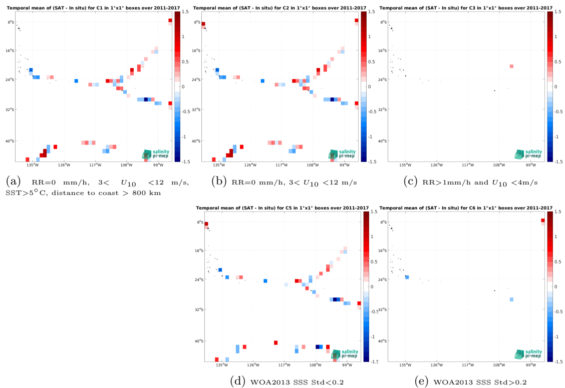
Figure 14: Temporal mean gridded over spatial boxes of size 1^\circ \times 1^\circ of \Delta SSS (SMOS SSS L2 v700 (ESA) - TSG (GOSUD-Sailing-ship)) for 5 different subdatasets corresponding to:RR=0 mm/h, 3 < U_{10} < 12 m/s, SST >5^\circ\text{C} , distance to coast > 800 km (a), RR=0 mm/h, 3 < U_{10} < 12 m/s (b), RR >1 mm/h and U_{10} < 4 m/s (c), WOA2013 SSS Std <0.2 (d), WOA2013 SSS Std >0.2 (e).
