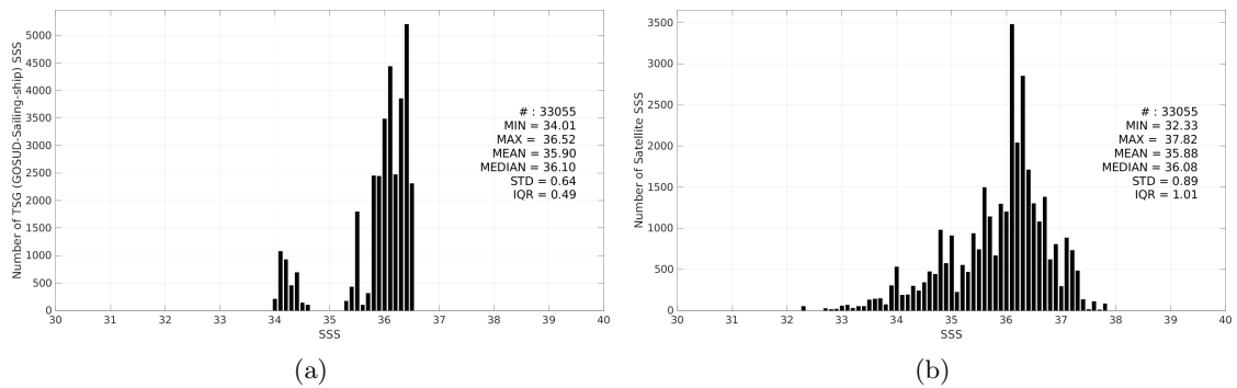
Figure 3: Histograms of SSS from TSG (GOSUD-Sailing-ship) (a) and SMOS SSS L2 v700 (ESA) (b) considering all match-up pairs per bins of 0.1 over the OTT zone Pi-MEP region and for the full satellite product period.
