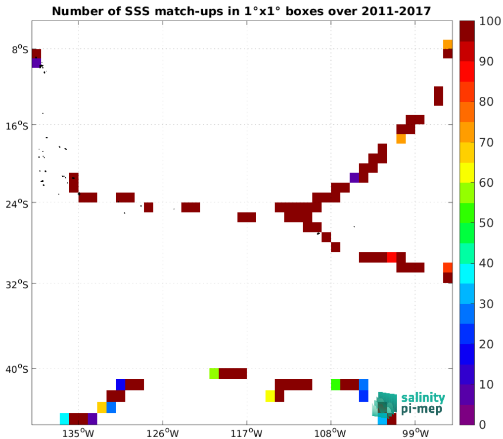
Figure 4: Number of SSS match-ups between TSG (GOSUD-Sailing-ship) SSS and the SMOS SSS L2 v700 (ESA) SSS product for the OTT zone Pi-MEP region over 1°x1° boxes and for the full satellite product period.
