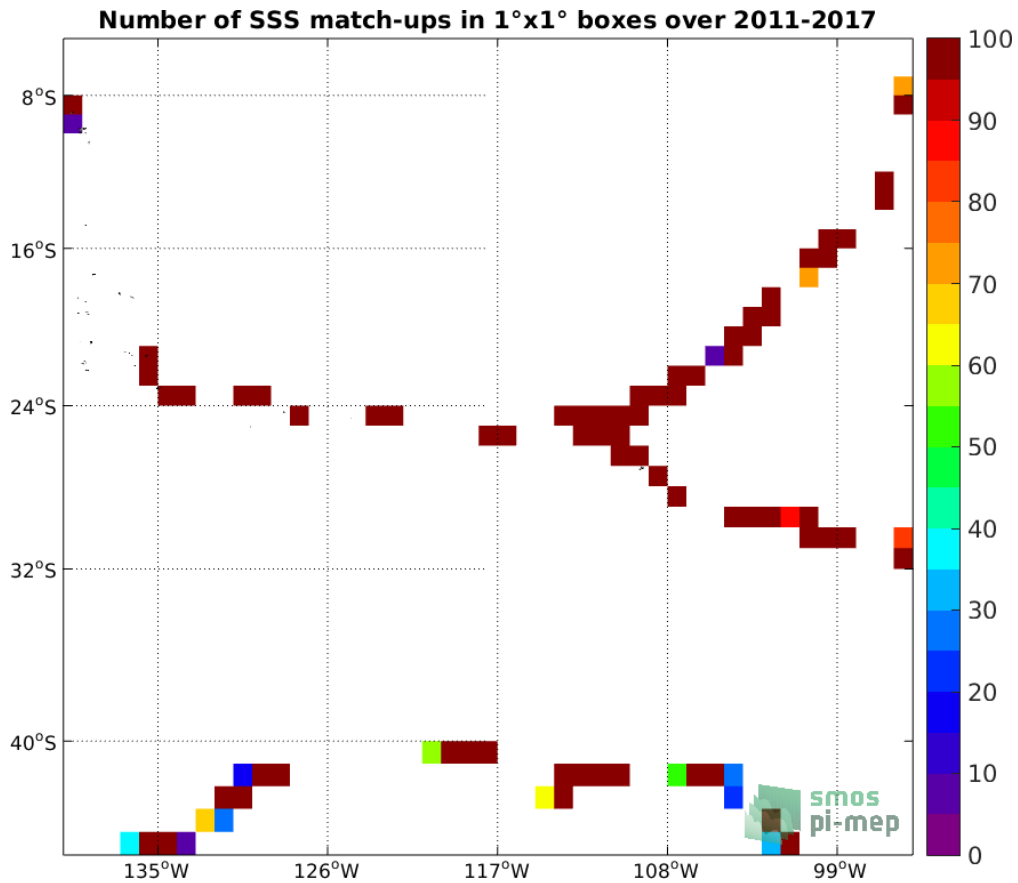
Figure 4: Number of SSS match-ups between TSG (GOSUD-Sailing-ship) SSS and the SMOS SSS L2 v700 (ESA) SSS product for the OTT zone Pi-MEP region over 1^\circ \times 1^\circ boxes and for the full satellite product period.
