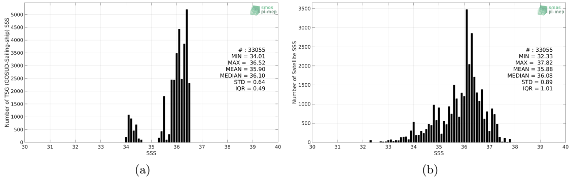
Figure 2: Histograms of SSS from TSG (GOSUD-Sailing-ship) (a) and SMOS SSS L2 v700 (ESA) (b) considering all match-up pairs per bins of 0.1 over the OTT zone Pi-MEP region and for the full satellite product period.
