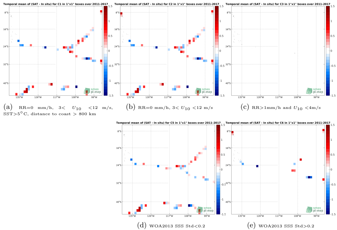
Figure 12: Temporal mean gridded over spatial boxes of size 1^\circ \times 1^\circ of \Delta\text{SSS} (SMOS SSS L2 v700 (ESA) - TSG (GOSUD-Sailing-ship)) for 5 different subdatasets corresponding to: RR=0 mm/h, 3 < U_{10} < 12 m/s, SST > 5°C, distance to coast > 800 km (a), RR=0 mm/h, 3 < U_{10} < 12 m/s (b), RR > 1mm/h and U_{10} < 4 m/s (c), WOA2013 SSS Std < 0.2 (d), WOA2013 SSS Std > 0.2 (e).
