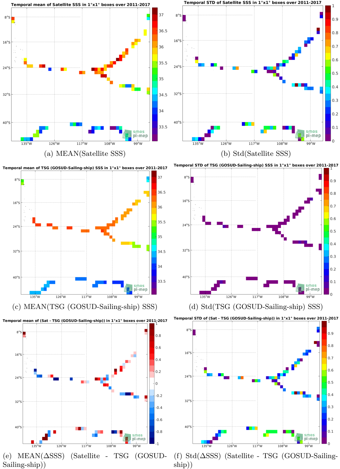
Figure 6: Temporal mean (left) and Std (right) of SSS from SMOS SSS L2 v700 (ESA) (top), TSG (GOSUD-Sailing-ship) (middle), and of \Delta SSS (Satellite - TSG (GOSUD-Sailing-ship)). Only match-up pairs are used to generate these maps.
