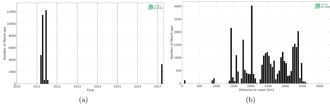
Figure 1: Number of match-ups between TSG (GOSUD-Sailing-ship) and SMOS SSS L2 v700 (ESA) SSS as a function of time (a) and as function of the distance to coast (b) over the OTT zone Pi-MEP region and for the full satellite product period.
