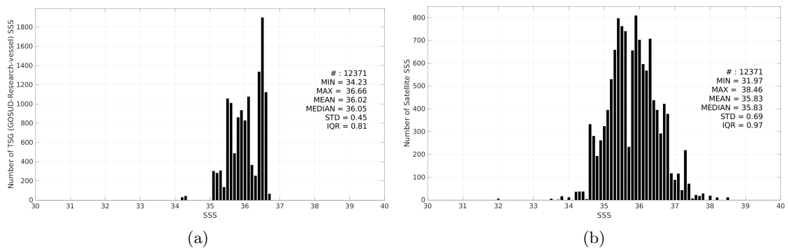
Figure 3: Histograms of SSS from TSG (GOSUD-Research-vessel) (a) and SMOS SSS L2 v700 (ESA) (b) considering all match-up pairs per bins of 0.1 over the OTT zone Pi-MEP region and for the full satellite product period.
