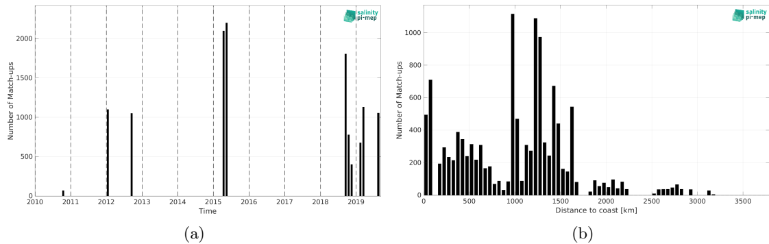
Figure 2: Number of match-ups between TSG (GOSUD-Research-vessel) and SMOS SSS L2 v700 (ESA) SSS as a function of time (a) and as function of the distance to coast (b) over the OTT zone Pi-MEP region and for the full satellite product period.
