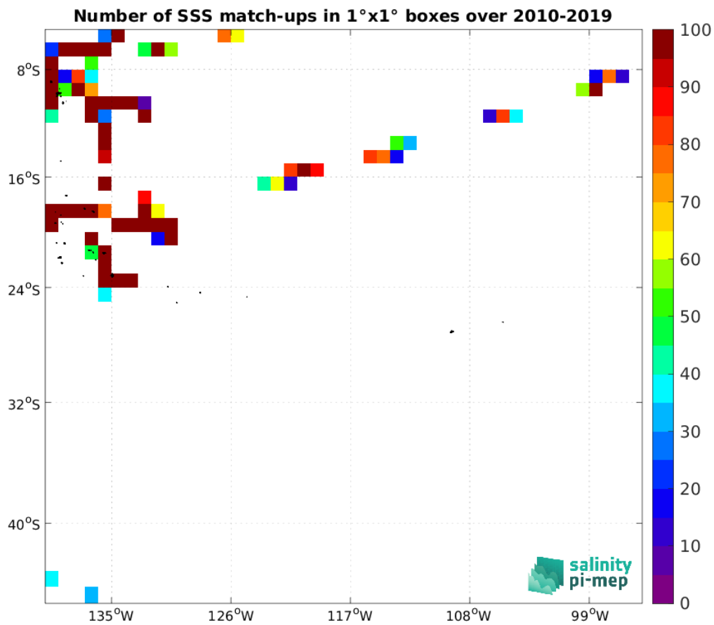
Figure 4: Number of SSS match-ups between TSG (GOSUD-Research-vessel) SSS and the SMOS SSS L2 v700 (ESA) SSS product for the OTT zone Pi-MEP region over 1^{\circ} \times 1^{\circ} boxes and for the full satellite product period.
