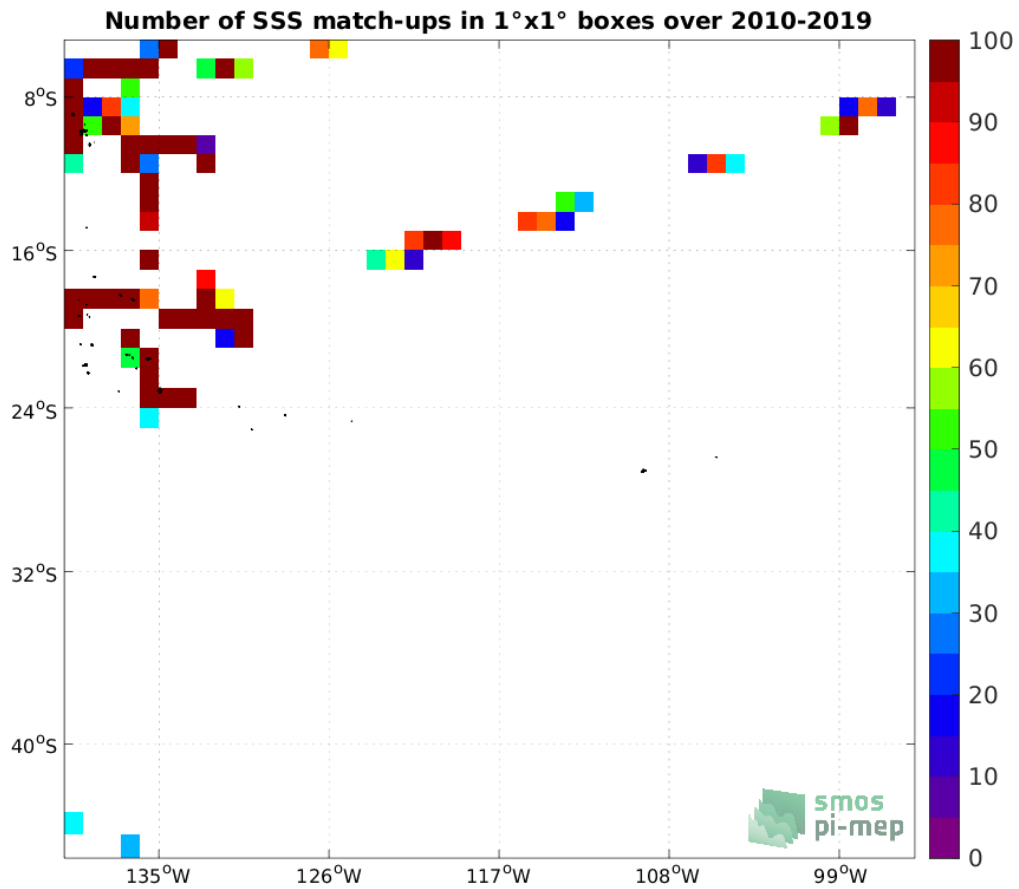
Figure 4: Number of SSS match-ups between TSG (GOSUD-Research-vessel) SSS and the SMOS SSS L2 v700 (ESA) SSS product for the OTT zone Pi-MEP region over 1°×1° boxes and for the full satellite product period.
