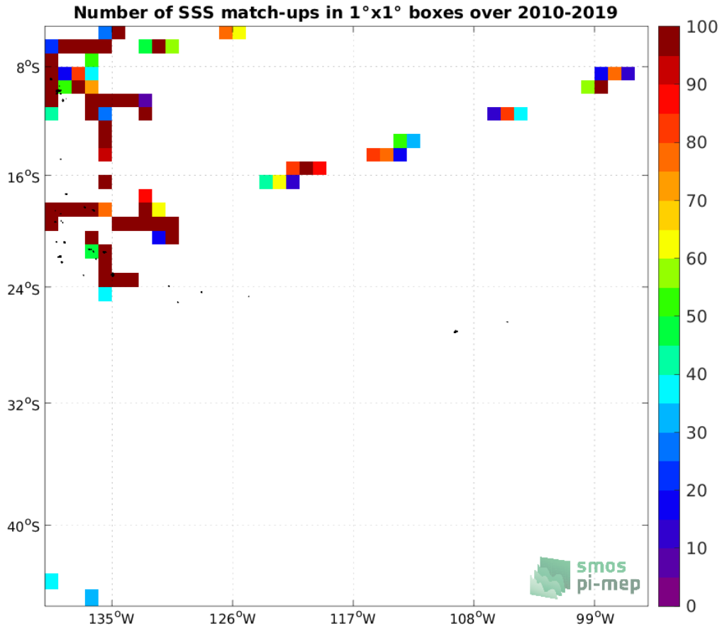
Figure 4: Number of SSS match-ups between TSG (GOSUD-Research-vessel) SSS and the SMOS SSS L2 v700 (ESA) SSS product for the OTT zone Pi-MEP region over 1^\circ \times 1^\circ boxes and for the full satellite product period.
