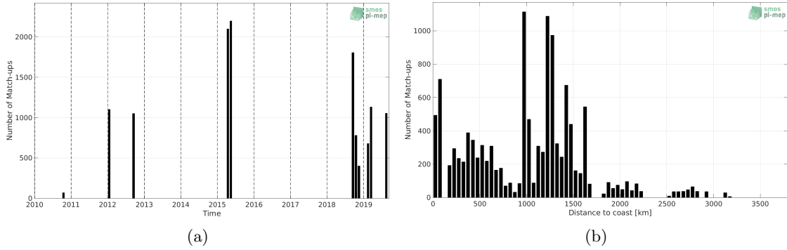
Figure 1: Number of match-ups between TSG (GOSUD-Research-vessel) and SMOS SSS L2 v700 (ESA) SSS as a function of time (a) and as function of the distance to coast (b) over the OTT zone Pi-MEP region and for the full satellite product period.
