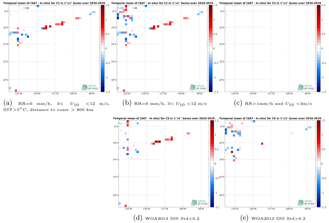
Figure 12: Temporal mean gridded over spatial boxes of size 1^\circ \times 1^\circ of \Delta SSS (SMOS SSS L2 v700 (ESA) - TSG (GOSUD-Research-vessel)) for 5 different subdatasets corresponding to: RR=0 mm/h, 3 < U_{10} < 12 m/s, SST > 5^\circ C , distance to coast > 800 km (a), RR=0 mm/h, 3 < U_{10} < 12 m/s (b), RR > 1 mm/h and U_{10} < 4 m/s (c), WOA2013 SSS Std < 0.2 (d), WOA2013 SSS Std > 0.2 (e).
