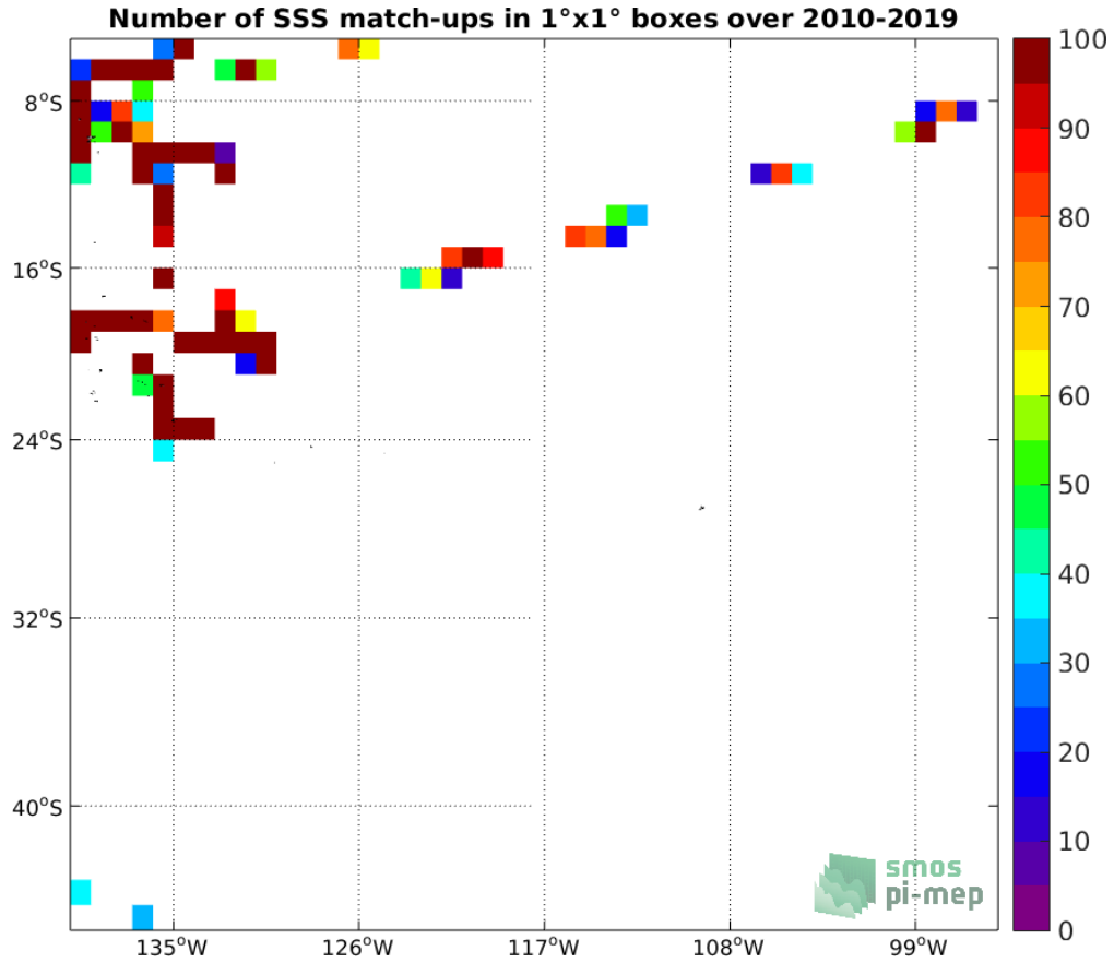
Figure 4: Number of SSS match-ups between TSG (GOSUD-Research-vessel) SSS and the SMOS SSS L2 v700 (ESA) SSS product for the OTT zone Pi-MEP region over 1°x1° boxes and for the full satellite product period.
