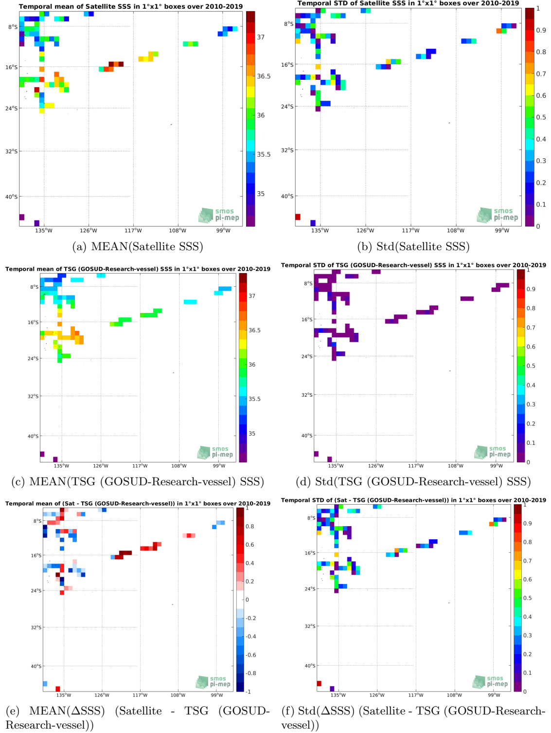
Figure 6: Temporal mean (left) and Std (right) of SSS from SMOS SSS L2 v700 (ESA) (top), TSG (GOSUD-Research-vessel) (middle), and of \Delta SSS (Satellite - TSG (GOSUD-Research-vessel)). Only match-up pairs are used to generate these maps.
