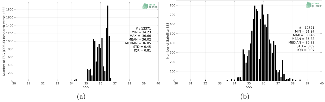
Figure 2: Histograms of SSS from TSG (GOSUD-Research-vessel) (a) and SMOS SSS L2 v700 (ESA) (b) considering all match-up pairs per bins of 0.1 over the OTT zone Pi-MEP region and for the full satellite product period.
