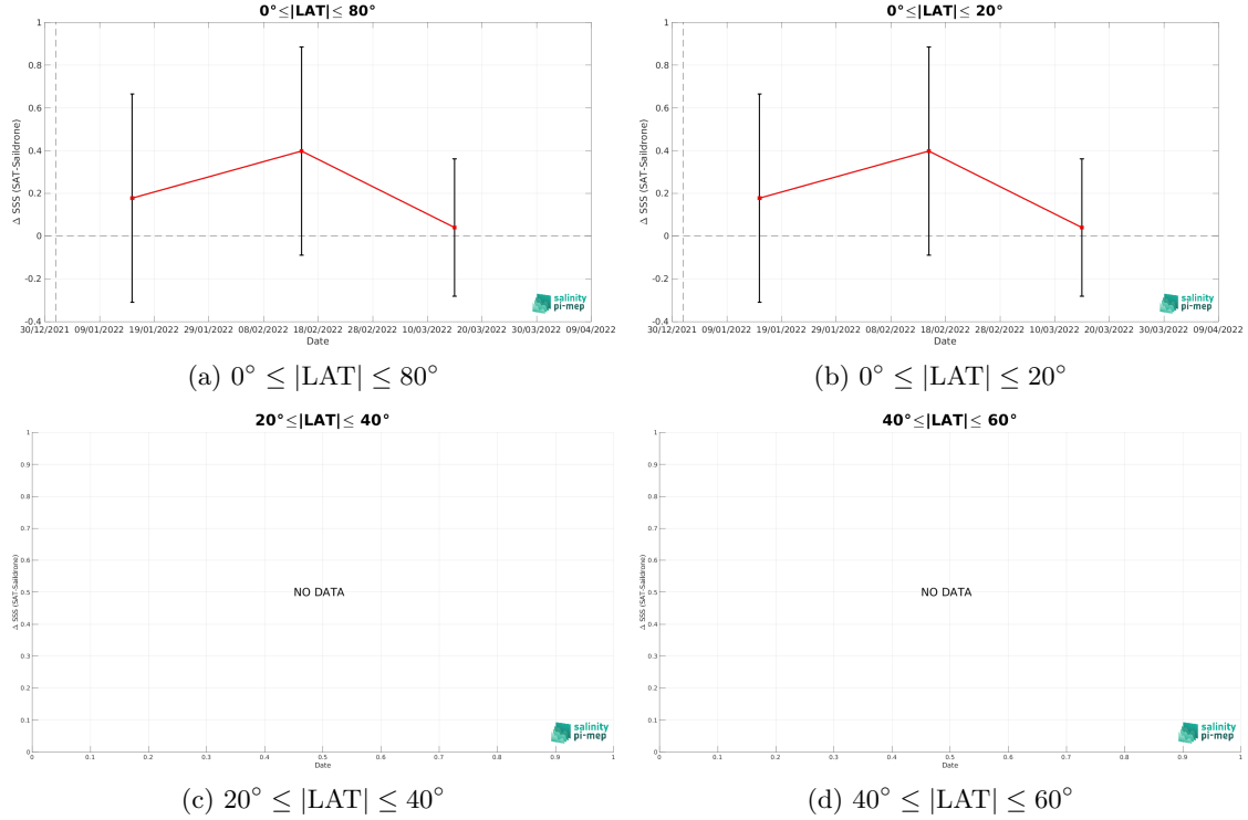
Figure 10: Monthly median (red curves) of \Delta SSS (Satellite - Saldrone) and \pm 1 Std (black vertical thick bars) as function of time for all the collected Pi-MEP match-up pairs estimated over the OTT zone Pi-MEP region and for the full satellite product period are shown for different latitude bands: (a) 80°S-80°N, (b) 20°S-20°N, (c) 40°S-20°S and 20°N-40°N and (d) 60°S-40°S and 40°N-60°N.
