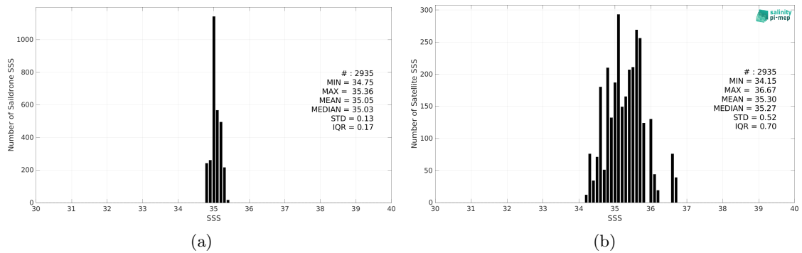
Figure 2: Histograms of SSS from Saildrone (a) and SMOS SSS L2 v700 (ESA) (b) considering all match-up pairs per bins of 0.1 over the OTT zone Pi-MEP region and for the full satellite product period.
