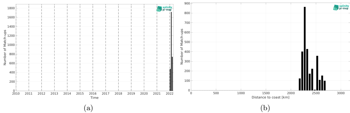
Figure 1: Number of match-ups between Saildrone and SMOS SSS L2 v700 (ESA) SSS as a function of time (a) and as function of the distance to coast (b) over the OTT zone Pi-MEP region and for the full satellite product period.
