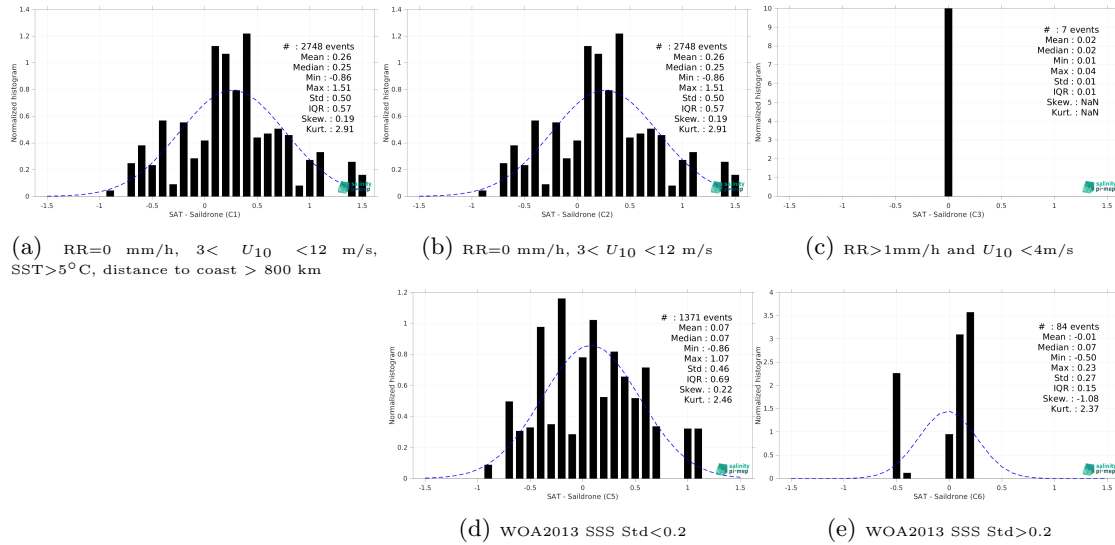
Figure 13: Normalized histogram of \Delta SSS (SMOS SSS L2 v700 (ESA) - Saldrone) for 5 different subdatasets corresponding to: RR=0 mm/h, 3 < U_{10} < 12 m/s, SST > 5°C, distance to coast > 800 km (a), RR=0 mm/h, 3 < U_{10} < 12 m/s (b), RR > 1mm/h and U_{10} < 4 m/s (c), WOA2013 SSS Std < 0.2 (d), WOA2013 SSS Std > 0.2 (e).
