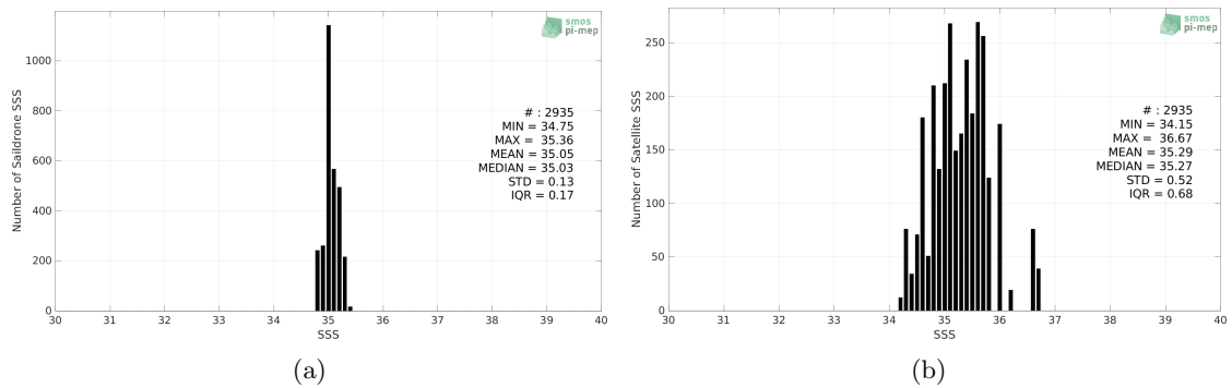
Figure 2: Histograms of SSS from Sairdrone (a) and SMOS SSS L2 v700 (ESA) (b) considering all match-up pairs per bins of 0.1 over the OTT zone Pi-MEP region and for the full satellite product period.
