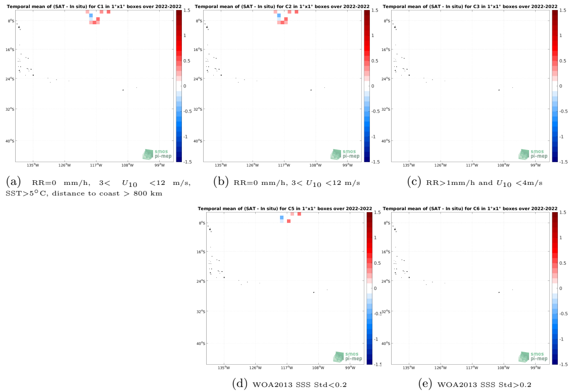
Figure 12: Temporal mean gridded over spatial boxes of size 1^\circ \times 1^\circ of \Delta SSS (SMOS SSS L2 v700 (ESA) - Sairdrone) for 5 different subdatasets corresponding to:RR=0 mm/h, 3 < U_{10} < 12 m/s, SST >5^\circ C, distance to coast > 800 km (a), RR=0 mm/h, 3 < U_{10} < 12 m/s (b), RR >1 mm/h and U_{10} < 4 m/s (c), WOA2013 SSS Std <0.2 (d), WOA2013 SSS Std >0.2 (e).
