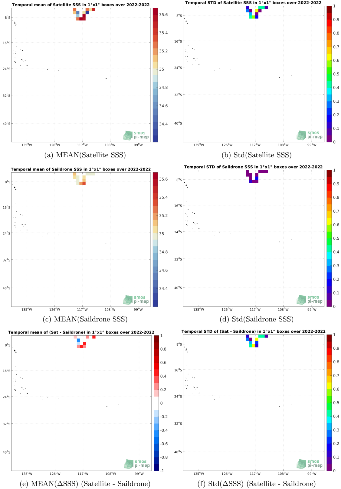
Figure 6: Temporal mean (left) and Std (right) of SSS from SMOS SSS L2 v700 (ESA) (top), Saildrone (middle), and of \Delta SSS (Satellite - Saildrone). Only match-up pairs are used to generate these maps.
