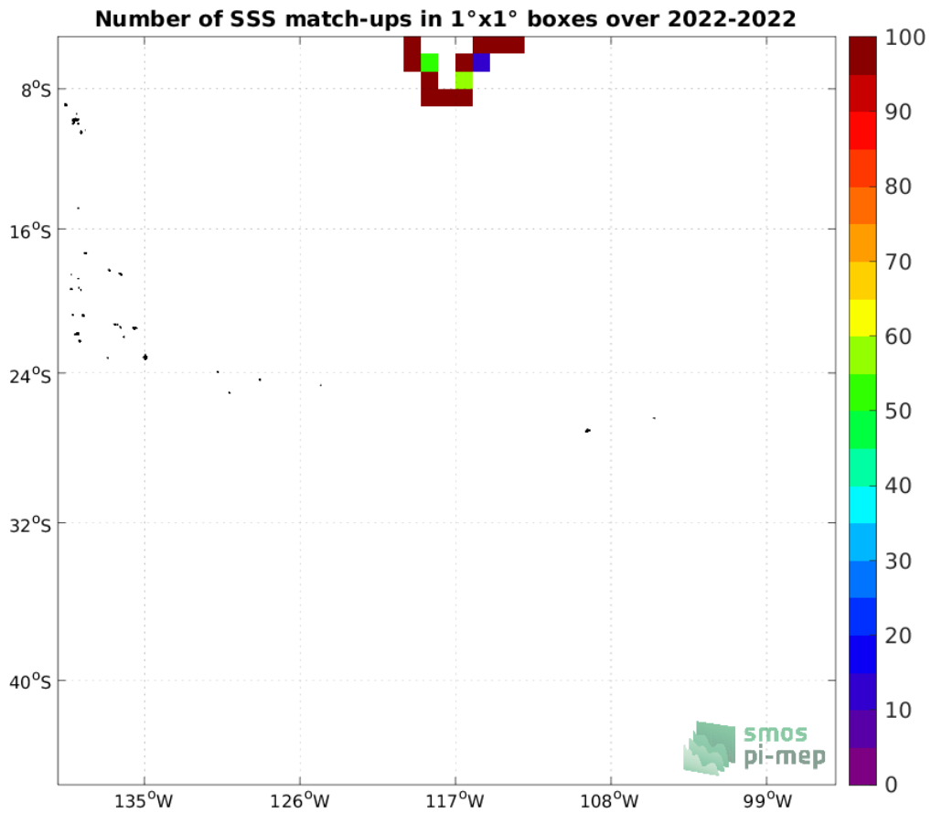
Figure 4: Number of SSS match-ups between Saildrone SSS and the SMOS SSS L2 v700 (ESA) SSS product for the OTT zone Pi-MEP region over 1^\circ \times 1^\circ boxes and for the full satellite product period.
