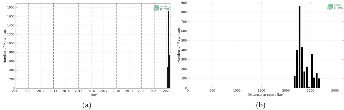
Figure 1: Number of match-ups between Sairdrone and SMOS SSS L2 v700 (ESA) SSS as a function of time (a) and as function of the distance to coast (b) over the OTT zone Pi-MEP region and for the full satellite product period.
