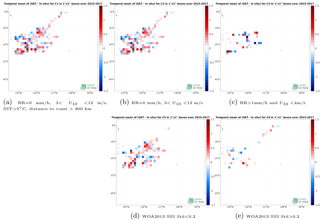
Figure 11: Temporal mean gridded over spatial boxes of size 1^\circ \times 1^\circ of \Delta SSS (SMOS SSS L2 v700 (ESA) - Surface drifters) for 5 different subdatasets corresponding to:RR=0 mm/h, 3 < U_{10} < 12 m/s, SST >5^\circ C, distance to coast > 800 km (a), RR=0 mm/h, 3 < U_{10} < 12 m/s (b), RR >1 mm/h and U_{10} < 4 m/s (c), WOA2013 SSS Std <0.2 (d), WOA2013 SSS Std >0.2 (e).
