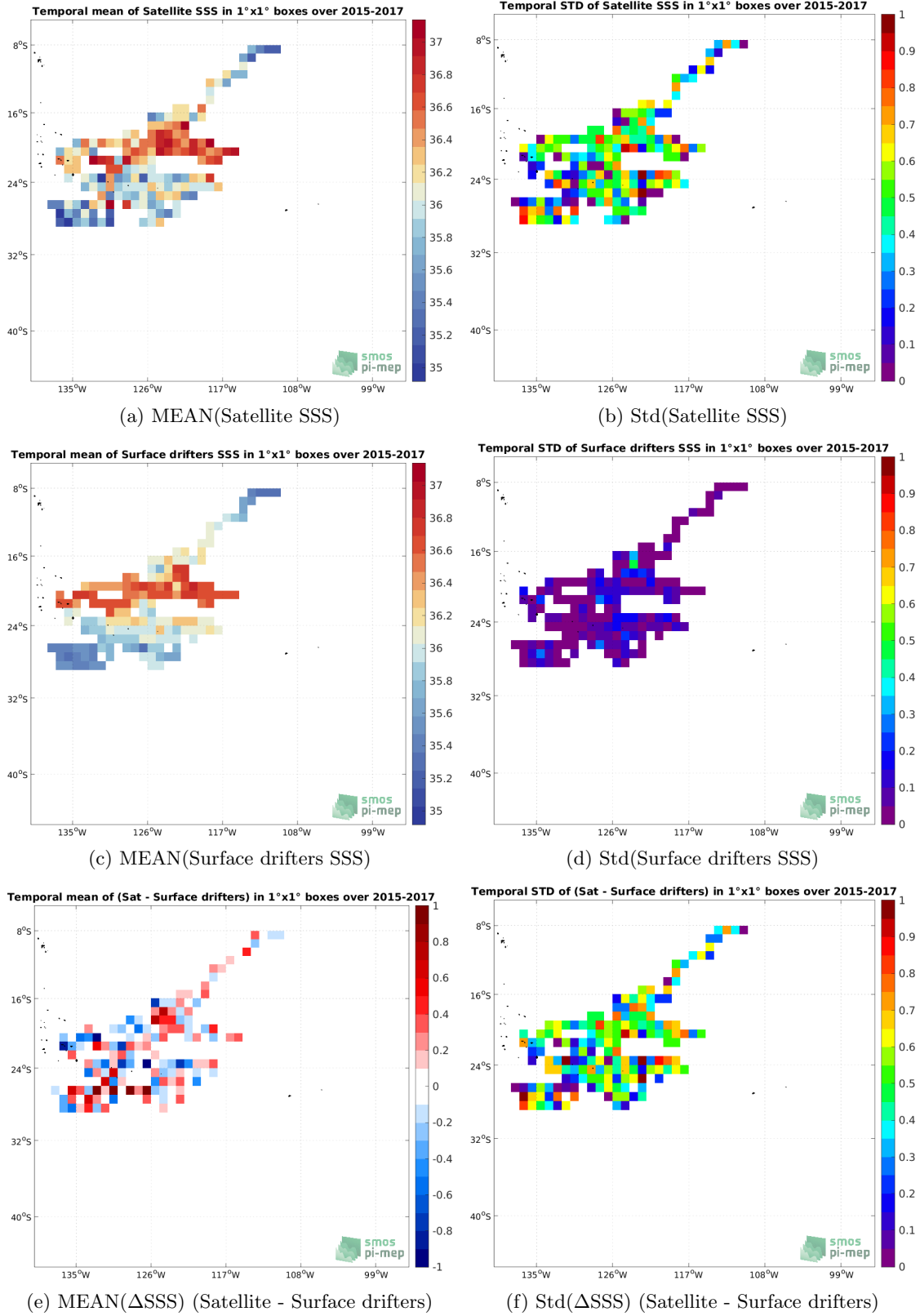
Figure 5: Temporal mean (left) and Std (right) of SSS from SMOS SSS L2 v700 (ESA) (top), Surface drifters (middle), and of \Delta SSS (Satellite - Surface drifters). Only match-up pairs are used to generate these maps.
