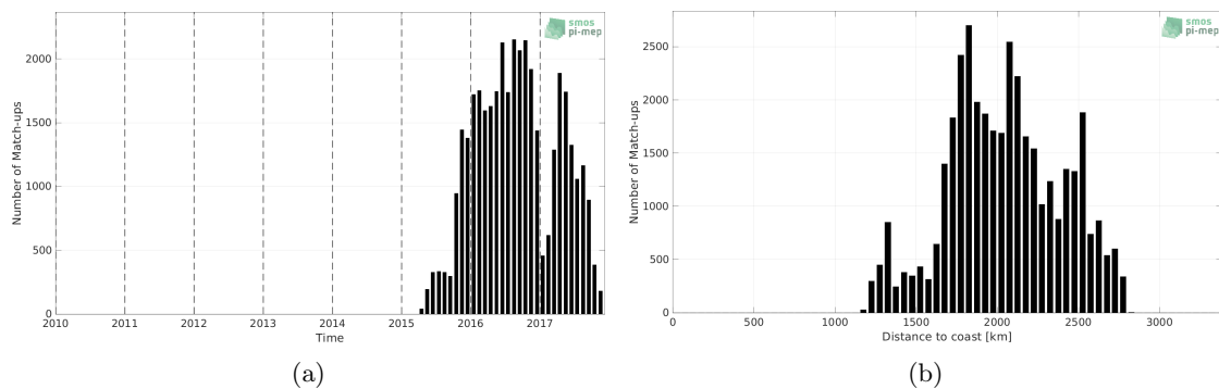
Figure 1: Number of match-ups between Surface drifters and SMOS SSS L2 v700 (ESA) SSS as a function of time (a) and as function of the distance to coast (b) over the OTT zone Pi-MEP region and for the full satellite product period.
