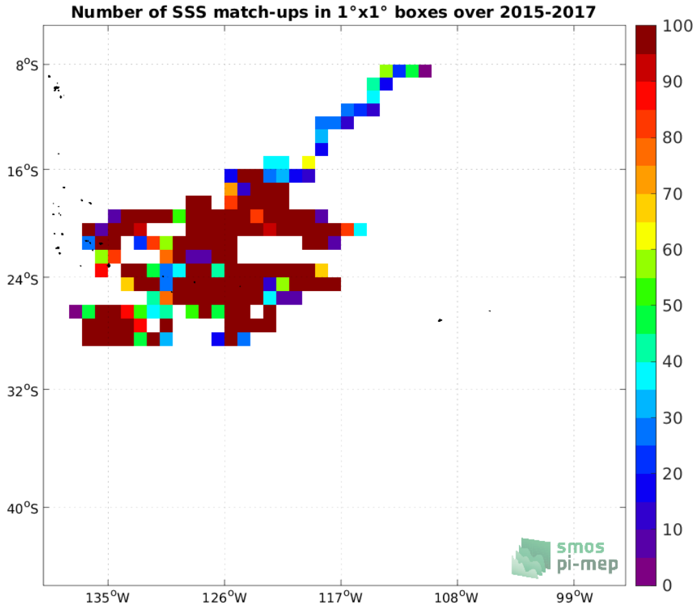
Figure 3: Number of SSS match-ups between Surface drifters SSS and the SMOS SSS L2 v700 (ESA) SSS product for the OTT zone Pi-MEP region over 1^\circ \times 1^\circ boxes and for the full satellite product period.
