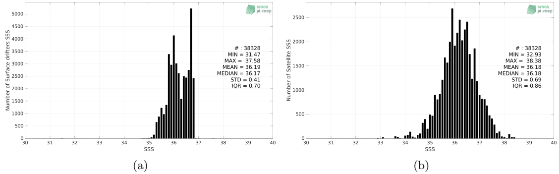
Figure 2: Histograms of SSS from Surface drifters (a) and SMOS SSS L2 v700 (ESA) (b) considering all match-up pairs per bins of 0.1 over the OTT zone Pi-MEP region and for the full satellite product period.
