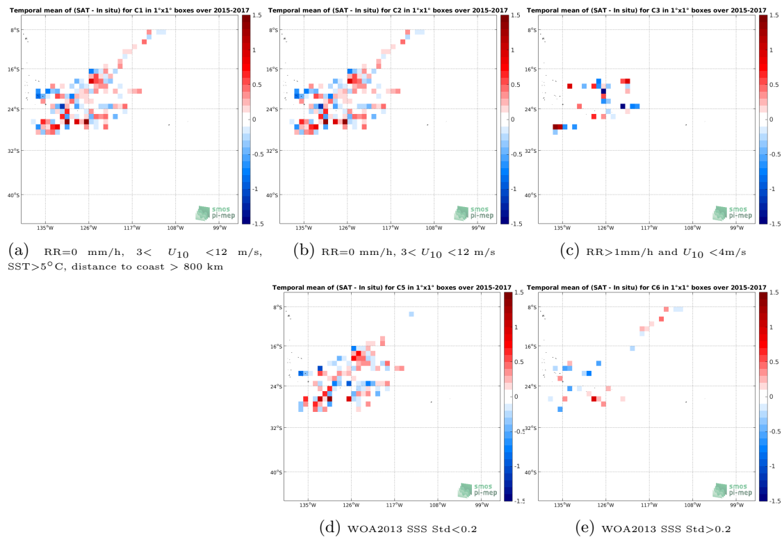
Figure 11: Temporal mean gridded over spatial boxes of size 1^\circ \times 1^\circ of \Delta\text{SSS} (SMOS SSS L2 v700 (ESA) - Surface drifters) for 5 different subdatasets corresponding to:RR=0 mm/h, 3 < U_{10} < 12 m/s, SST >5^\circ\text{C} , distance to coast > 800 km (a), RR=0 mm/h, 3 < U_{10} < 12 m/s (b), RR >1 mm/h and U_{10} < 4 m/s (c), WOA2013 SSS Std <0.2 (d), WOA2013 SSS Std >0.2 (e).
