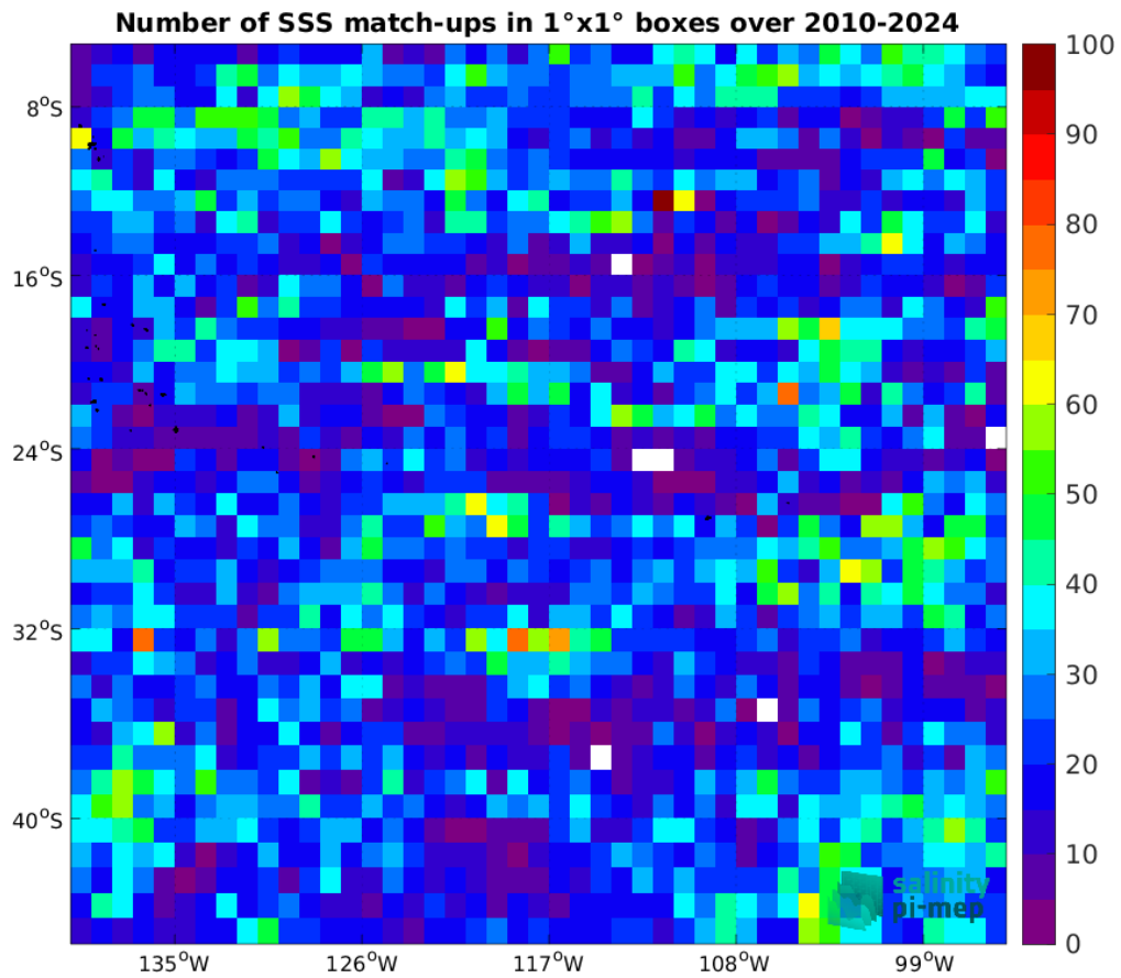
Figure 5: Number of SSS match-ups between Argo SSS and the SMOS SSS L2 v700 (ESA) SSS product for the OTT zone Pi-MEP region over 1°×1° boxes and for the full satellite product period.
