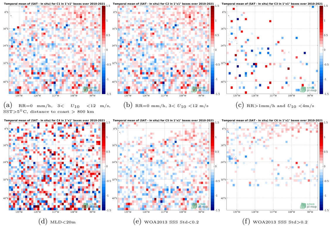
Figure 12: Temporal mean gridded over spatial boxes of size 1^\circ \times 1^\circ of \Delta SSS (SMOS SSS L2 v700 (ESA) - Argo) for 6 different subdatasets corresponding to:RR=0 mm/h, 3 < U_{10} < 12 m/s, SST >5^\circ C, distance to coast > 800 km (a), RR=0 mm/h, 3 < U_{10} < 12 m/s (b), RR >1 mm/h and U_{10} < 4 m/s (c),MLD <20 m (d),WOA2013 SSS Std <0.2 (e),WOA2013 SSS Std >0.2 (f).
