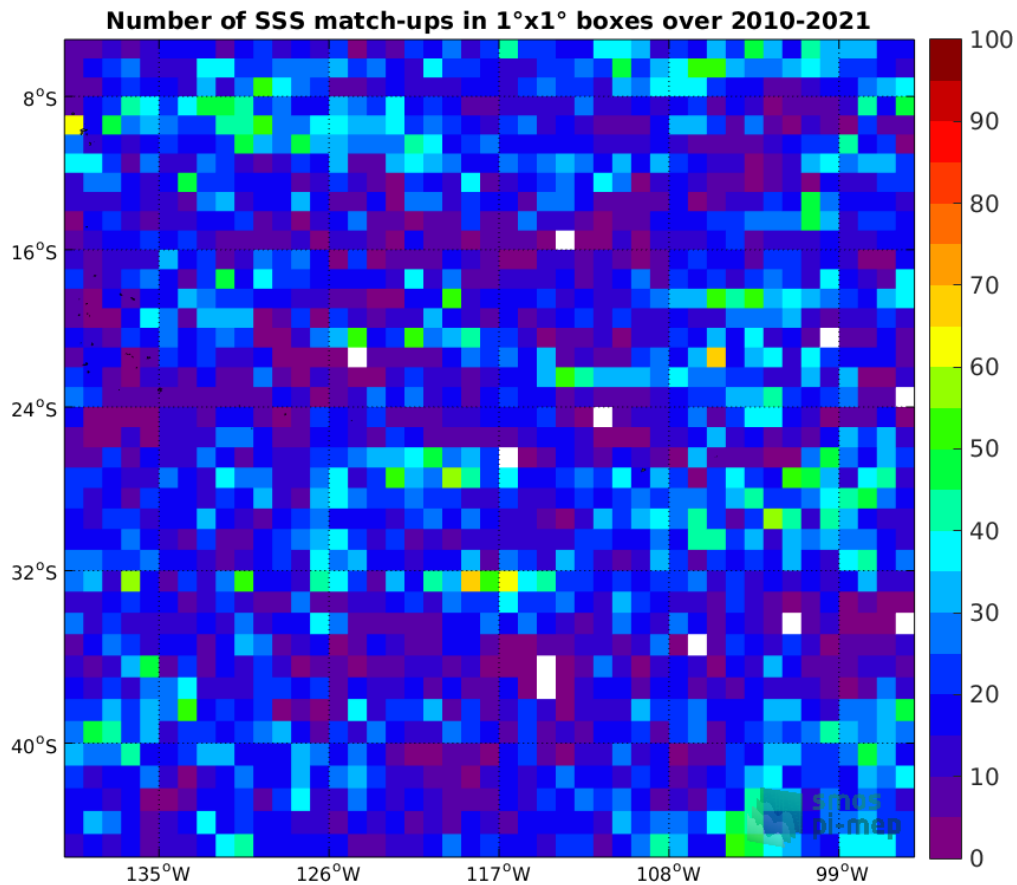
Figure 4: Number of SSS match-ups between Argo SSS and the SMOS SSS L2 v700 (ESA) SSS product for the OTT zone Pi-MEP region over 1^\circ \times 1^\circ boxes and for the full satellite product period.
