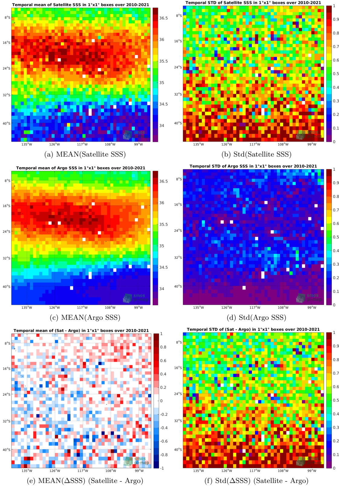
Figure 6: Temporal mean (left) and Std (right) of SSS from SMOS SSS L2 v700 (ESA) (top), Argo (middle), and of \Delta SSS (Satellite - Argo). 25 Only match-up pairs are used to generate these maps.
