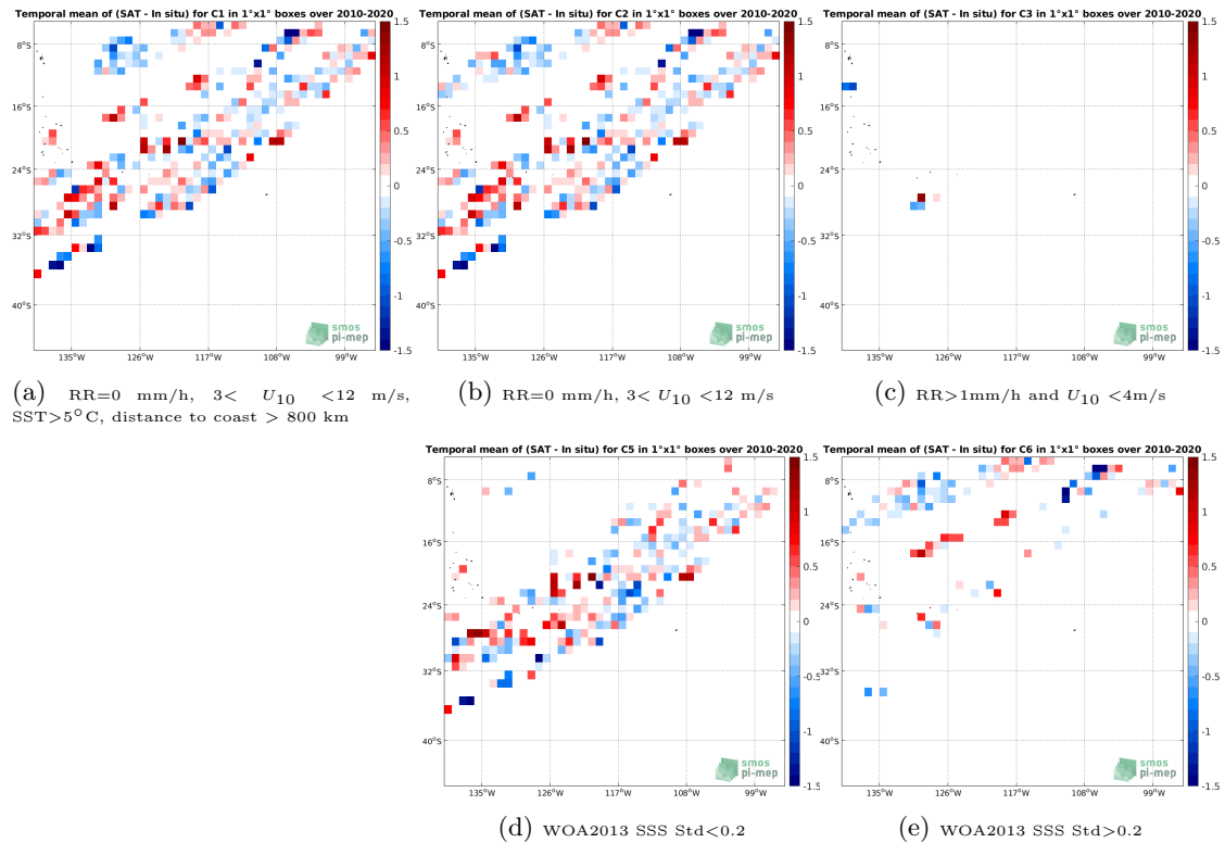
Figure 12: Temporal mean gridded over spatial boxes of size 1^\circ \times 1^\circ of \Delta SSS (SMOS SSS L2 v662 (ESA) - TSG (LEGOS-DM)) for 5 different subdatasets corresponding to: RR=0 mm/h, 3 < U_{10} < 12 m/s, SST > 5^\circ\text{C} , distance to coast > 800 km (a), RR=0 mm/h, 3 < U_{10} < 12 m/s (b), RR > 1 mm/h and U_{10} < 4 m/s (c), WOA2013 SSS Std < 0.2 (d), WOA2013 SSS Std > 0.2 (e).
