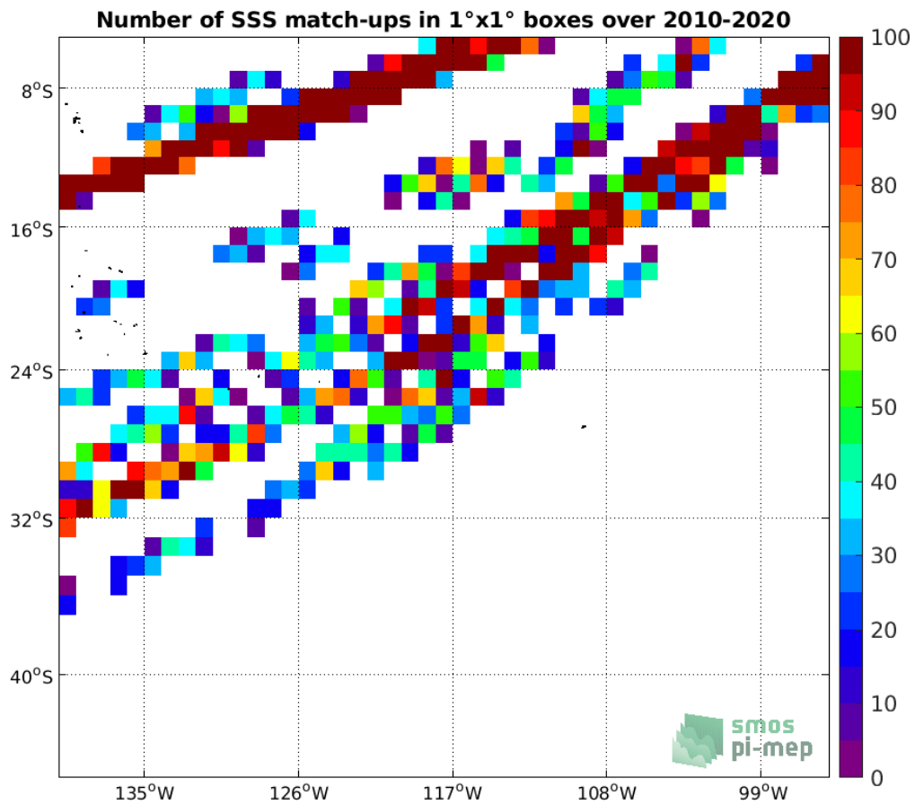
Figure 4: Number of SSS match-ups between TSG (LEGOS-DM) SSS and the SMOS SSS L2 v662 (ESA) SSS product for the OTT zone Pi-MEP region over 1^\circ \times 1^\circ boxes and for the full satellite product period.
