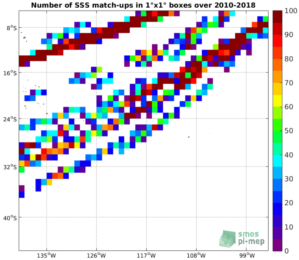
Figure 4: Number of SSS match-ups between TSG (LEGOS-DM) SSS and the SMOS SSS L2 v662 (ESA) SSS product for the OTT zone Pi-MEP region over 1°x1° boxes and for the full satellite product period.
