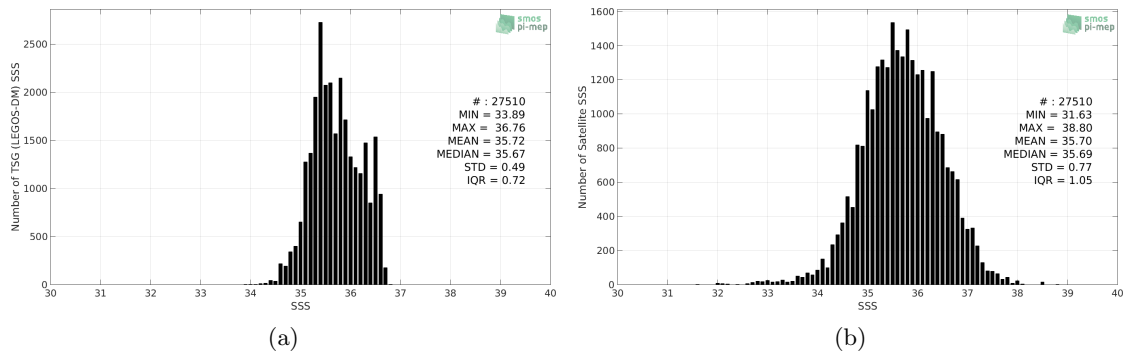
Figure 2: Histograms of SSS from TSG (LEGOS-DM) (a) and SMOS SSS L2 v662 (ESA) (b) considering all match-up pairs per bins of 0.1 over the OTT zone Pi-MEP region and for the full satellite product period.
