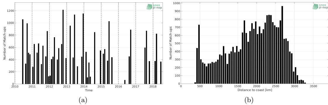
Figure 1: Number of match-ups between TSG (LEGOS-DM) and SMOS SSS L2 v662 (ESA) SSS as a function of time (a) and as function of the distance to coast (b) over the OTT zone Pi-MEP region and for the full satellite product period.
