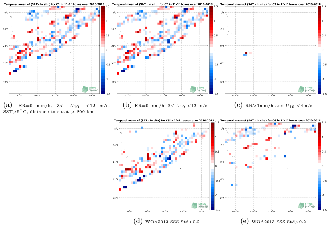
Figure 12: Temporal mean gridded over spatial boxes of size 1^\circ \times 1^\circ of \Delta SSS (SMOS SSS L2 v662 (ESA) - TSG (LEGOS-DM)) for 5 different subdatasets corresponding to:RR=0 mm/h, 3 < U_{10} < 12 m/s, SST >5^\circ\text{C} , distance to coast > 800 km (a), RR=0 mm/h, 3 < U_{10} < 12 m/s (b), RR >1 mm/h and U_{10} < 4 m/s (c), WOA2013 SSS Std <0.2 (d), WOA2013 SSS Std >0.2 (e).
