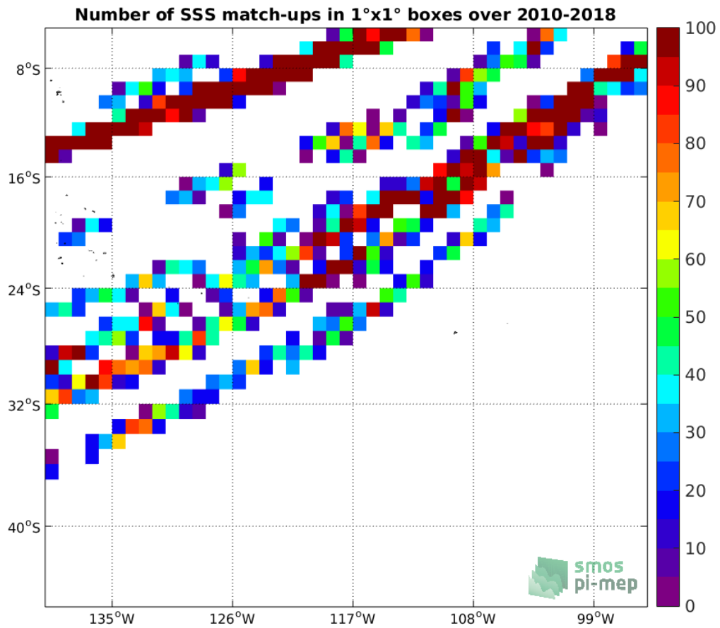
Figure 4: Number of SSS match-ups between TSG-LEGOS-DM SSS and the SMOS L2 v662 (ESA) SSS product for the OTT zone Pi-MEP region over 1°x1° boxes and for the full satellite product period.
