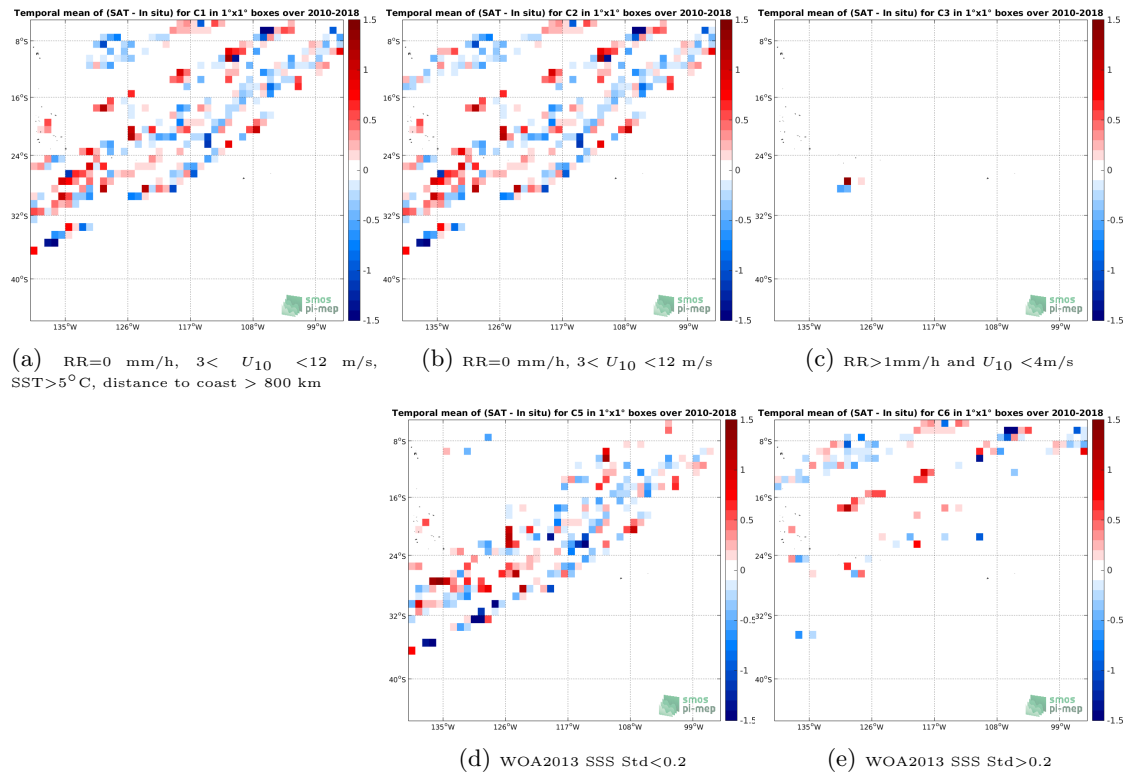
Figure 12: Temporal mean gridded over spatial boxes of size 1^\circ \times 1^\circ of \Delta SSS (SMOS L2 v662 (ESA) - TSG-LEGOS-DM) for 5 different subdatasets corresponding to:RR=0 mm/h, 3 < U_{10} < 12 m/s, SST >5^\circ C, distance to coast > 800 km (a), RR=0 mm/h, 3 < U_{10} < 12 m/s (b), RR >1 mm/h and U_{10} < 4 m/s (c), WOA2013 SSS Std <0.2 (d), WOA2013 SSS Std >0.2 (e).
