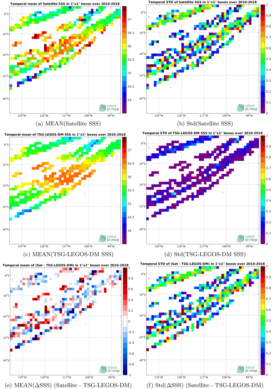
Figure 6: Temporal mean (left) and Std (right) of SSS from SMOS L2 v662 (ESA) (top), TSG-LEGOS-DM (middle), and of \Delta SSS (Satellite - TSG-LEGOS-DM). Only match-up pairs are used to generate these maps.
