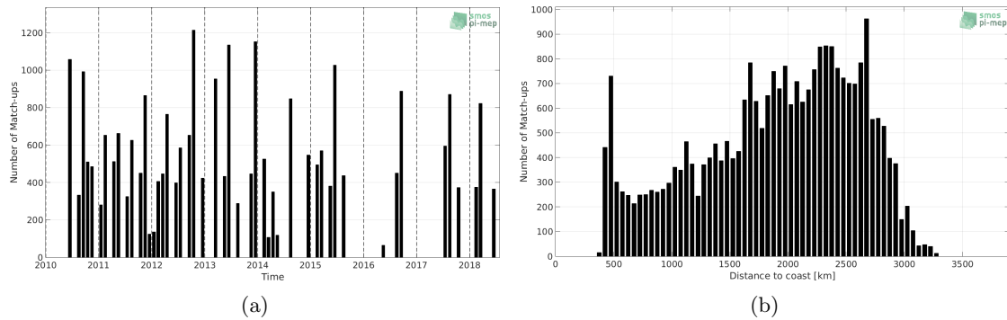
Figure 1: Number of match-ups between TSG-LEGOS-DM and SMOS L2 v662 (ESA) SSS as a function of time (a) and as function of the distance to coast (b) over the OTT zone Pi-MEP region and for the full satellite product period.
