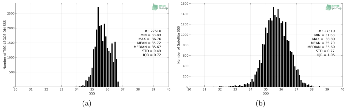
Figure 2: Histograms of SSS from TSG-LEGOS-DM (a) and SMOS L2 v662 (ESA) (b) considering all match-up pairs per bins of 0.1 over the OTT zone Pi-MEP region and for the full satellite product period.
