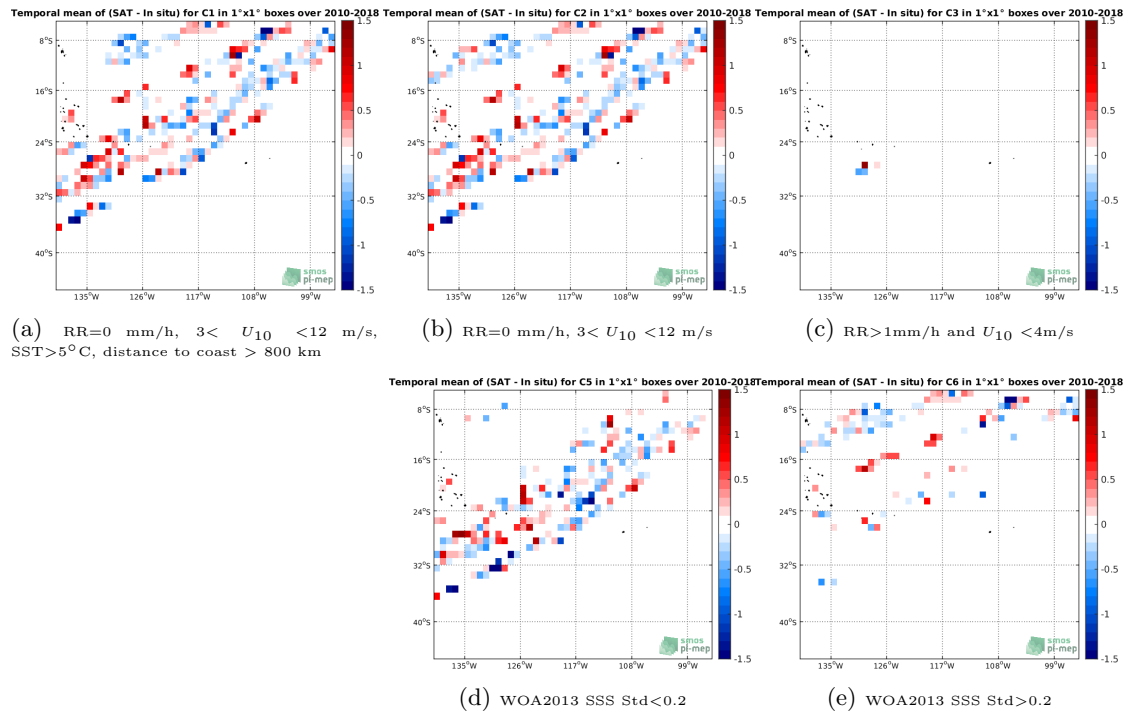
Figure 12: Temporal mean gridded over spatial boxes of size 1^\circ \times 1^\circ of \Delta SSS (SMOS-L2-DPGS-v662 - TSG-LEGOS-DM) for 5 different subdatasets corresponding to: RR=0 mm/h, 3 < U_{10} < 12 m/s, SST > 5^\circ C, distance to coast > 800 km (a), RR=0 mm/h, 3 < U_{10} < 12 m/s (b), RR > 1 mm/h and U_{10} < 4 m/s (c), WOA2013 SSS Std < 0.2 (d), WOA2013 SSS Std > 0.2 (e).
