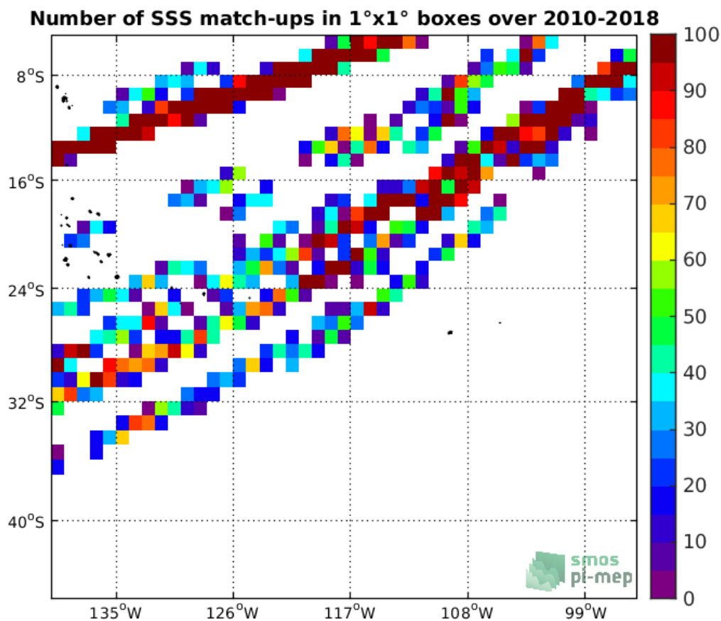
Figure 4: Number of SSS match-ups between TSG-LEGOS-DM SSS and the SMOS-L2-DPGS-v662 SSS product for the OTT zone Pi-MEP region over 1°x1° boxes and for the full satellite product period.
