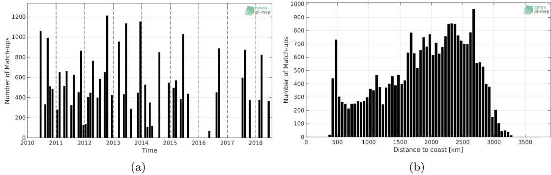
Figure 1: Number of match-ups between TSG-LEGOS-DM and SMOS-L2-DPGS-v662 SSS as a function of time (a) and as function of the distance to coast (b) over the OTT zone Pi-MEP region and for the full satellite product period.
