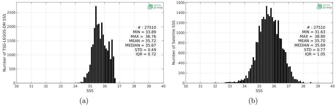
Figure 2: Histograms of SSS from TSG-LEGOS-DM (a) and SMOS-L2-DPGS-v662 (b) considering all match-up pairs per bins of 0.1 over the OTT zone Pi-MEP region and for the full satellite product period.
