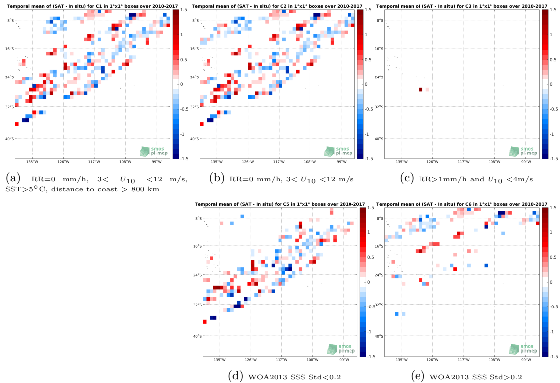
Figure 12: Temporal mean gridded over spatial boxes of size 1^\circ \times 1^\circ of \Delta SSS (SMOS-L2-DPGS-v662 - TSG-LEGOS-DM) for 5 different subdatasets corresponding to:RR=0 mm/h, 3 < U_{10} < 12 m/s, SST >5^\circ C, distance to coast > 800 km (a), RR=0 mm/h, 3 < U_{10} < 12 m/s (b), RR >1 mm/h and U_{10} < 4 m/s (c), WOA2013 SSS Std <0.2 (d), WOA2013 SSS Std >0.2 (e).
